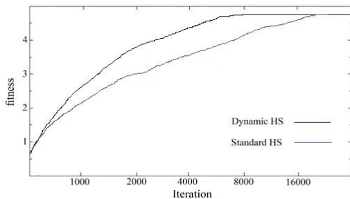
FIGURE 4. Comparison between the standard HS and Dynamic HS (DHS)
