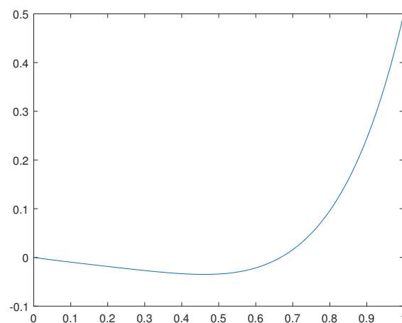
Figure 1. solution u_0(x) for the case f(x) = 0 .
