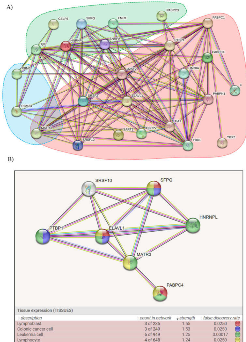
Figure 2. a) The graph displays the connection between all known RBPs, which are grouped by the motif to which they can bind. b) The set of proteins in the network is provided in the table under "Count in Network." Strength (observed/expected: Log10) indicates the size of the enrichment effect. It is the ratio between the number of proteins in query that are annotated with a term and the number of proteins we would anticipate in a randomly generated network of the same size. False Discovery Rate indicates the importance of the enrichment. The Benjamini-Hochberg method is used to adjust the p-values for multiple testing within each category and is shown.
