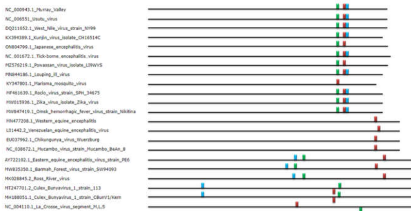
Figure 1. a) The conserved sequences that were found by comparing all of the strains are included in this figure. All consensus motifs are reported using "motif logos" and according to IUPAC nomenclature. Moreover, a complete list of RBPs has been supplied. b) RBPs binding site distribution on arbovirus sequences analyzed. The colors red, green, and light blue correspond to the motifs shown in a).
