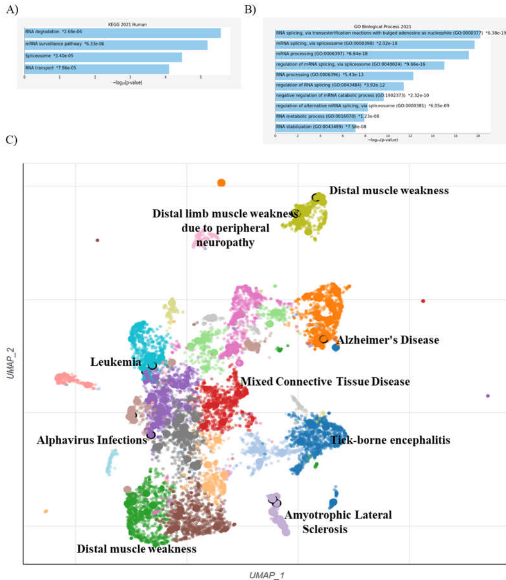
Figure 3. a). The bar chart shows the top 4 enriched terms in KEGG_2021 library, along with their corresponding p-values. Colored bars correspond to terms with significant p-values ( <0.05 ). An asterisk (*) next to a p-value indicates the term also has a significant adjusted p-value ( <0.05 ). b) The bar chart of the top 10 enriched terms in GO-biological process library c) UMAP scatterplot enriched analysis for the DisGeNET database. A library term is represented by each point. The gene set associated with each word had its term frequency-inverse document frequency (TF-IDF) values calculated, and the resulting values were then subjected to UMAP. The first two UMAP dimensions are used to map the terms. Term positions tend to be closer together for gene sets that are more similar. The TF-IDF data are transformed into automatically selected clusters using the Leiden technique. The query is more profoundly enhanced the darker and bigger the point.
