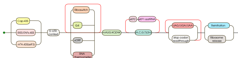
Figure 1. Translational regulation graph in eukaryotes. Key regulatory contexts: Cap – five-prime cap, 43S – 43S preinitiation complex, IRES – internal ribosome entry site, ITAFs – IRES-transacting factors, m^6A – N^6 -methyladenosine, G4 – G-quadruplexes, uORF – upstream open reading frames, mAUG – main AUG, KOZAK – Kozak consensus sequences, aa-tRNA – aminoacyl-tRNA, eIF* – eukaryotic initiation factors, eEF* – eukaryotic elongation factors. Edges corresponding to the direct course of the translation process are marked in black; cycles within the translation are marked in red.
