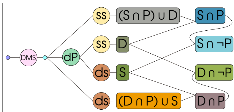
Figure 2. Obtaining complete mRNA structure data by combining Structure-seq and PIP-seq. DMS – dimethyl sulphate, dP – proteinase treatment, ss – single-strand-specific nuclease treatment, ds – double-strand-specific nuclease treatment, D – set of double-stranded mRNA fragments, S – set of single-stranded mRNA fragments, P – set of protein-shielded mRNA fragments.
