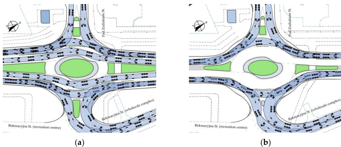
Figure A6. Examples of swept path analysis for elliptical turbo roundabouts with straight-through movements from the main approach legs plus right-turn movements: (a) With two exit lanes on the main approach legs – III type; (b) With one lane on the main approach legs – IV type. Source: own work.
