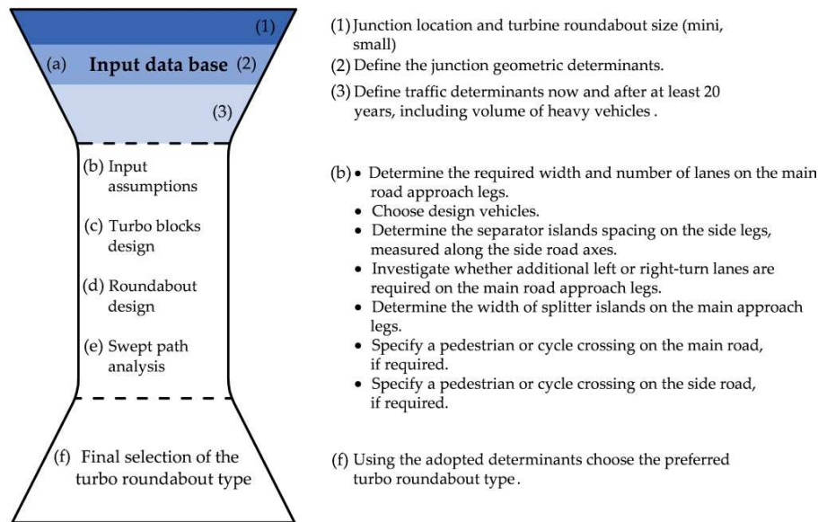
Figure 4. The turbo roundabout selection method for constrained areas is presented in IMRAD diagram.
