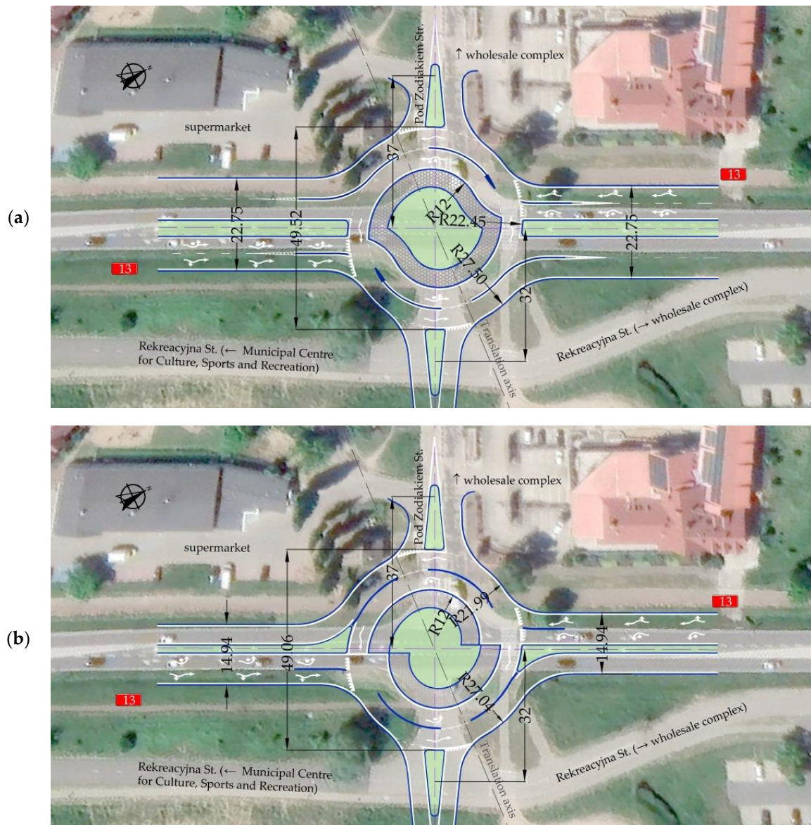
Figure 7. Constraints and selected parameters of Egg turbo roundabout located in the outskirts of Szczecin – a case study: (a) 0.7 m wide raised separation lane, inner lane started in the old manner; (b) 0.24 m wide separation lane, inner lane started in a new manner. Source: own work on a satellite image background, roundabout site example from Google Earth [11].
