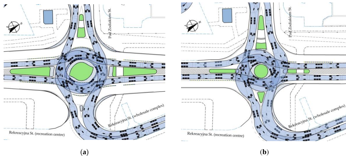
Figure 12. Examples of swept path analyses for "flattened" roundabouts left-turn movements: (a) With two exit lanes on the main approach legs – I type; (b) With one lane on the main approach legs – II type. Source: own work.
