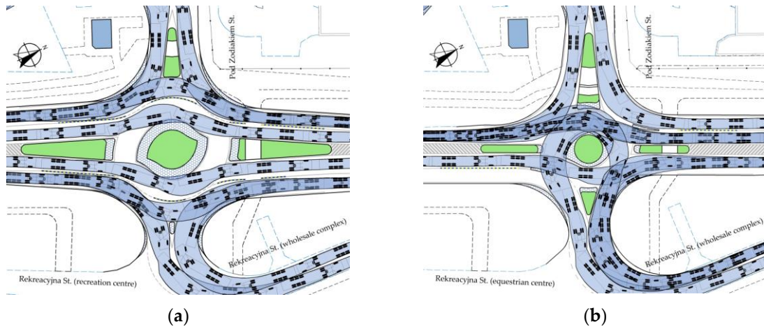
Figure A5. Examples of swept path analysis for "flattened" roundabouts with straight-through movements from the main approach legs plus right-turn movements: (a) With two exit lanes on the main approach legs – I type; (b) With one lane on the main approach legs – II type. Source: own work.
