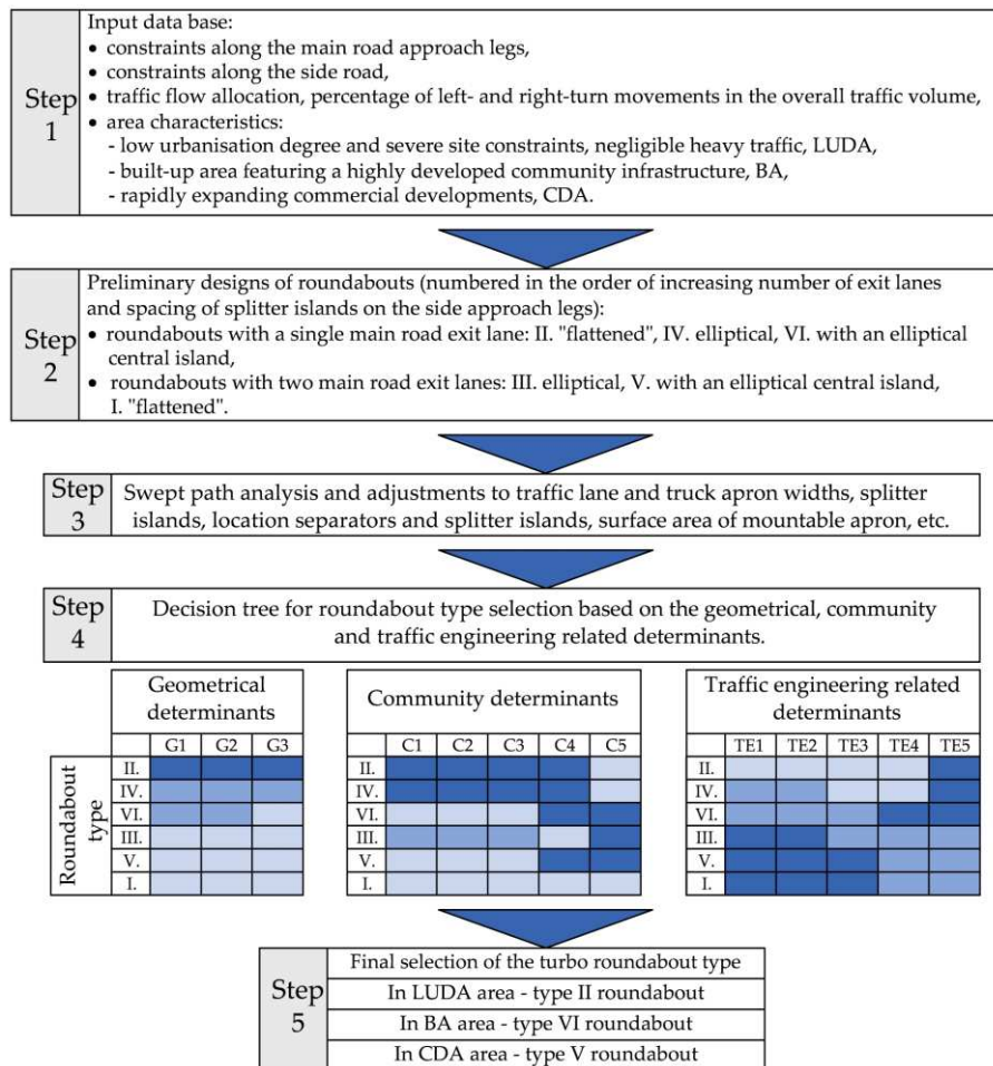
Figure 19. Analysis of the adopted determinants and selection of the turbo roundabout type for constrained site projects.
