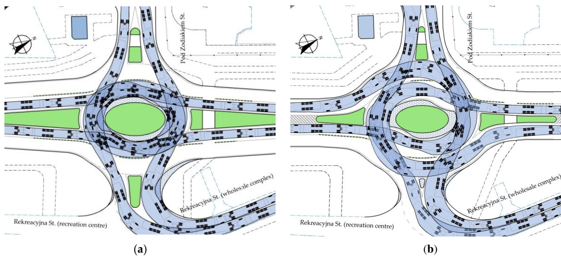
Figure 18. Examples of swept path analyses for elliptical roundabouts featuring an elliptical central island: (a) With two exit lanes on the main approach legs – V type; (b) With one lane on the main approach legs – VI type. Source: own work.
