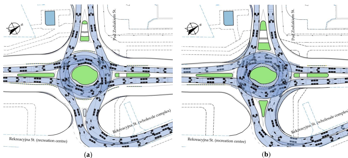
Figure 15. Examples of swept path analyses for elliptical roundabout left-turn movements: (a) With two exit lanes on the main approach legs – III type; (b) With one lane on the main approach legs – IV type. Source: own work.
