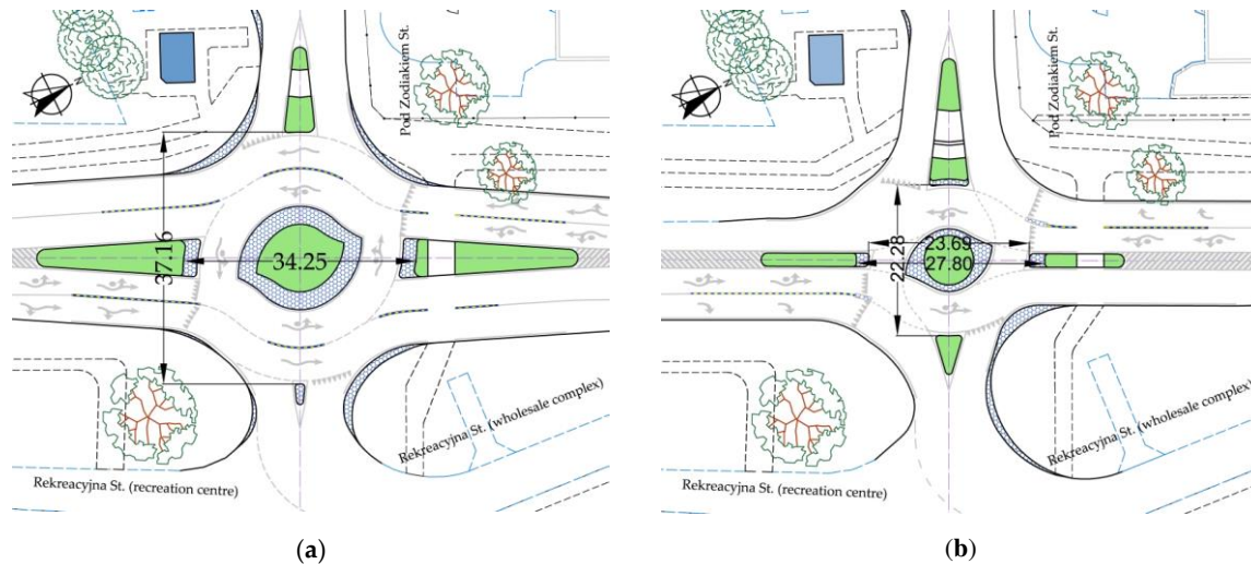
Figure 11. Examples of "flattened" roundabouts: (a) With two exit lanes on the main approach legs – I type; (b) With one lane on the main approach legs – II type. Source: own work.
