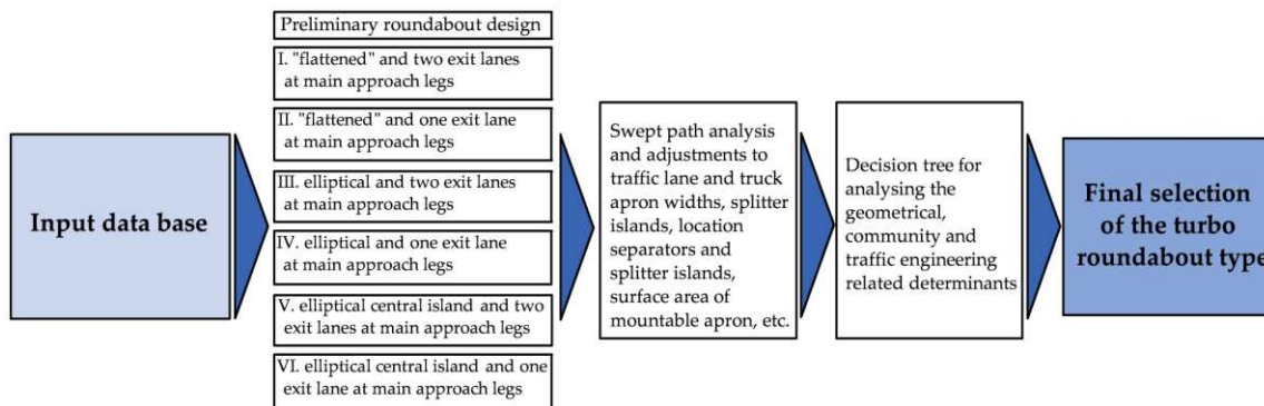
Figure 9. Turbo roundabout selection diagram step by step for constrained project sites.
