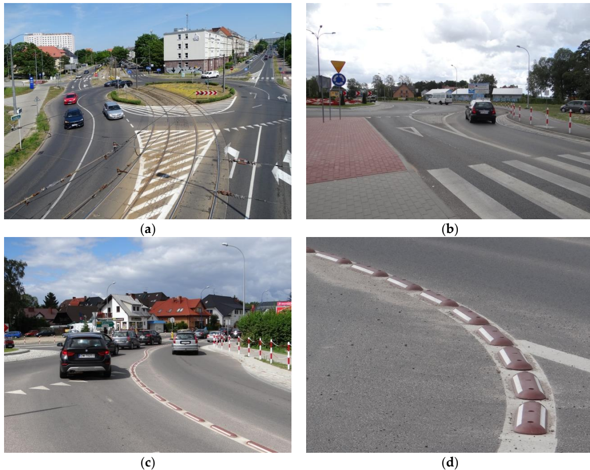
Figure 8. Examples of different separation lanes used in Poland: (a) Szczecin ( 53^{\circ}25'16.84''N , 14^{\circ}31'40.99''E ) – separation lane consisting of line markings only; (b) Dziwnówek ( 54^{\circ}1'56.65''N , 14^{\circ}48'26.53''E ) – traversable splitter island and line marking as the approach separation; (c) 0.24 m wide separation consisting of a line marking and U-25 raised separator; (d) detail of U-25 separator attached to the pavement on the line marking. (Photo by A. Sołowczuk).
