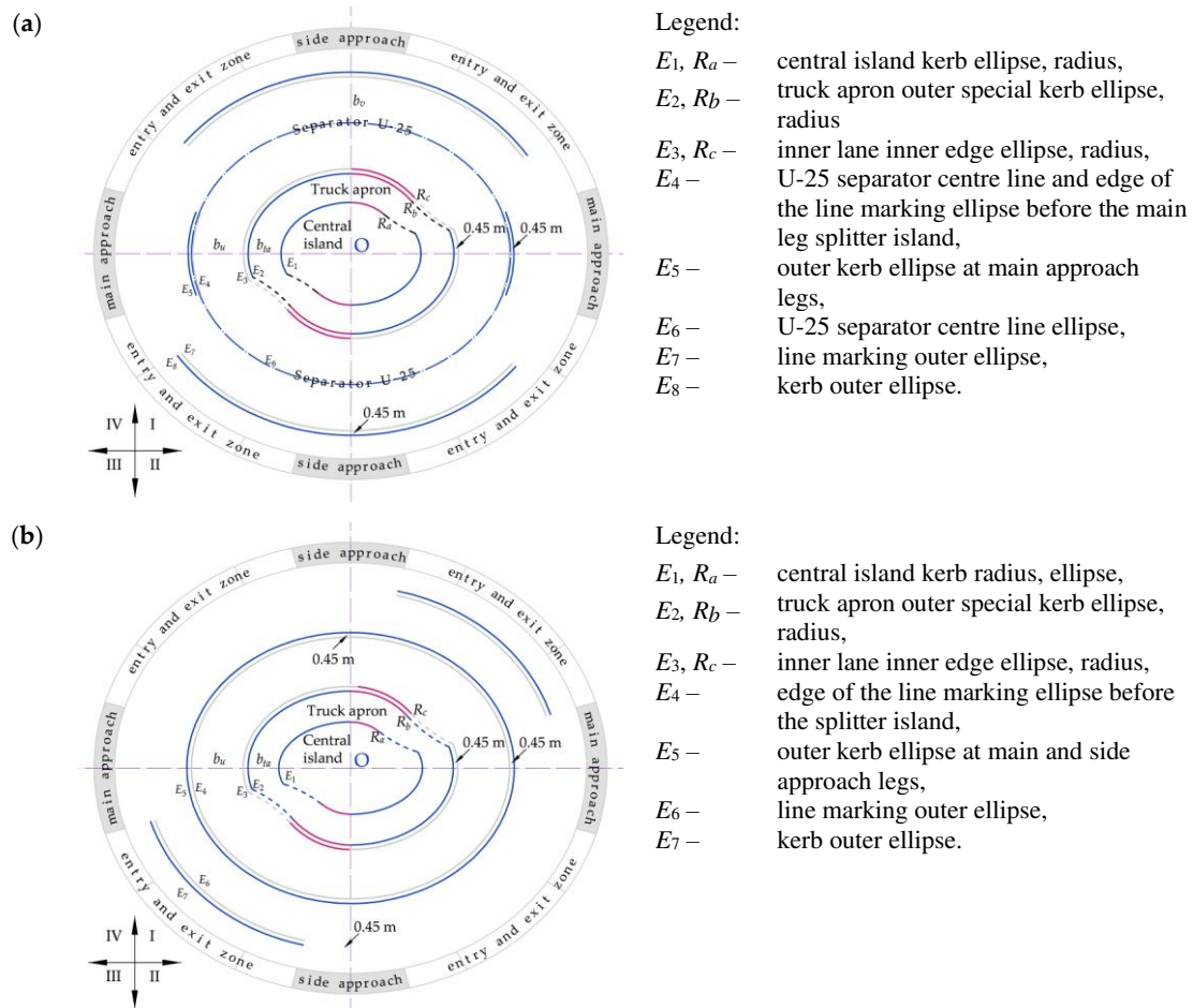
Figure 13. One exit lane at main approach legs. Turbo block for laying out elliptical turbo roundabouts: (a) With two exit lanes on the main approach legs – III type; (b) With one lane on the main approach legs – IV type. Source: own work.
