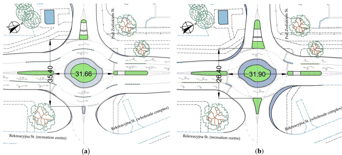
Figure 14. Examples of elliptical turbo roundabouts: (a) With two exit lanes on the main approach legs – III type; (b) With one lane on the main approach legs – IV type. Source: own work.
