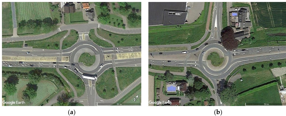
Figure 1. Examples of Egg turbo roundabouts located in constrained areas in vicinity of buildings in the Netherlands: (a) Wierden ( 52^{\circ}20'39.79''\text{N} , 6^{\circ}34'23.27''\text{E} ); (b) Krimpen aan den IJssel ( 51^{\circ}48'36.17''\text{N} , 4^{\circ}26'7.30''\text{E} ). (Source: Google Earth [11]).
