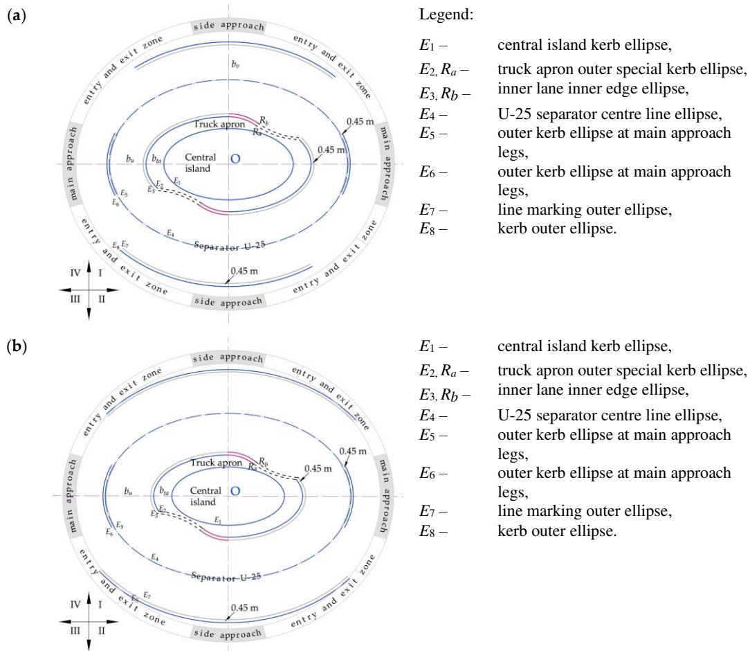
Figure 16. Turbo block for laying out elliptical turbo roundabouts featuring elliptical central island: (a) With two exit lanes on the main approach legs – V type; (b) With one lane on the main approach legs – VI type. Source: own work.
