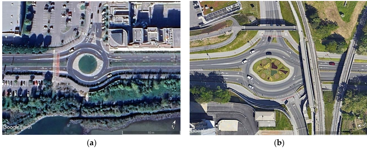
Figure 3. Examples of "flattened" roundabouts located in a constrained, built-up area in Slovenia: (a) Koper ( 45^{\circ}32'33.37''\text{N} , 13^{\circ}44'21.78''\text{E} ); (b) Maribor ( 46^{\circ}33'4.09''\text{N} , 15^{\circ}38'59.64''\text{E} ). (Source: Google Earth [11]).
