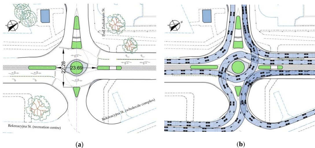
Figure 20. Example of "flattened" turbo roundabout with a single traffic lane on the main road approach leg, recommended for areas of low urbanisation degree LUDA – single-family neighbourhoods or woonerf: (a) Roundabout; (b) Swept path DV2. Source: own work.
