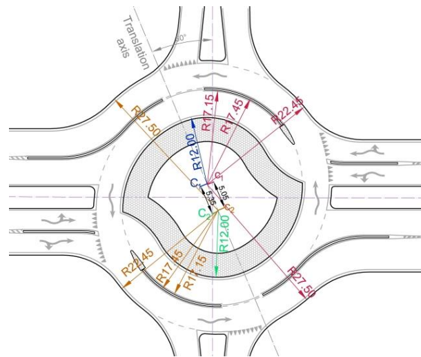
Figure A4. Turbo block of a conventional Egg small turbo roundabouts.
