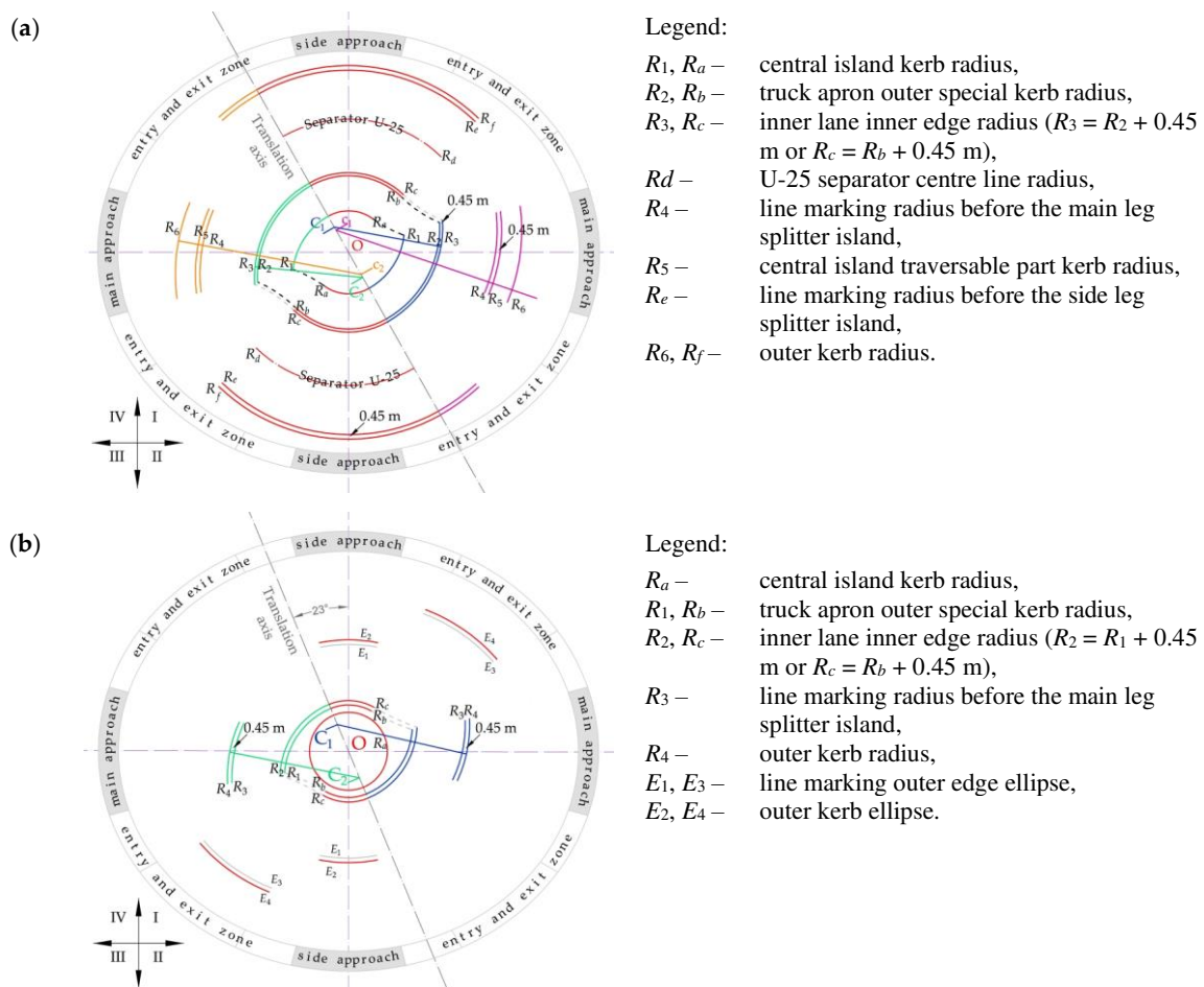
Figure 10. Turbo block to lay out "flattened" roundabouts: (a) With two exit lanes on the main approach legs – I type; (b) With one lane on the main approach legs – II type. Source: own work.
