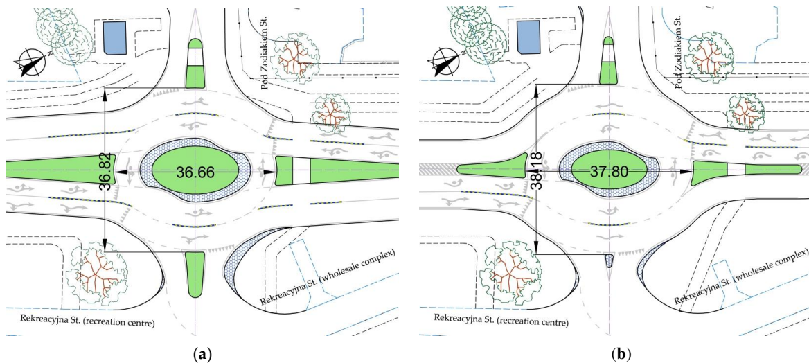
Figure 17. Examples of elliptical turbo roundabouts with an elliptical central island: (a) With two exit lanes on the main approach legs – V type; (b) With one lane on the main approach legs – VI type. Source: own work.
