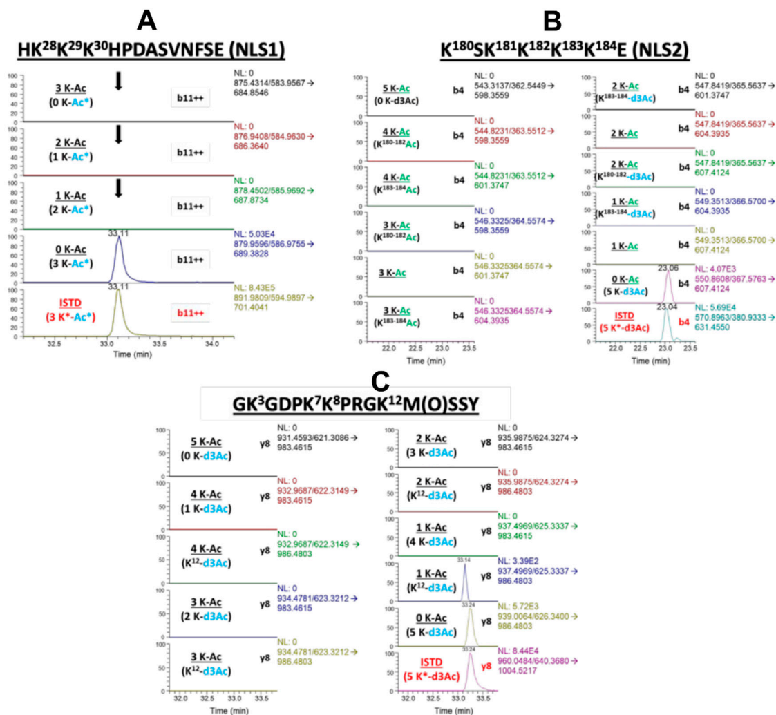
Figure 3. Cisplatin induced secretion of unacetylated HMGB1. Lysine-containing peptides from cisplatin treated A549 media were analyzed for acetylation by nano liquid chromatography parallel reaction monitoring/high-resolution mass spectrometry (nanoLC-PRM/HRMS). Chromatograms show light (black) and heavy (red) transitions with CD 3 or endogenous CH 3 -acetylation. (A) NanoLC-PRM/HRMS chromatograms for NLS1 peptide HK 28 K 29 K 30 HPDASVNFSE comparing b11 transitions for triply (first panel), doubly (second panel), and singly (third panel) acetylated NLS1 compared to unacetylated NLS1 peptide (fourth panel) and heavy NLS1 peptide (fifth panel). (B) NanoLC-PRM/HRMS chromatograms for NLS2 peptide K 180 SK 181 K 182 K 183 K 184 E comparing y8 transitions of different possible acetylation states. (C) NanoLC-PRM/HRMS chromatograms for N-terminal peptide GK 3 GDPK 7 K 8 PRGK 12 M(O)SSY comparing b4 transitions of different possible acetylation states.
