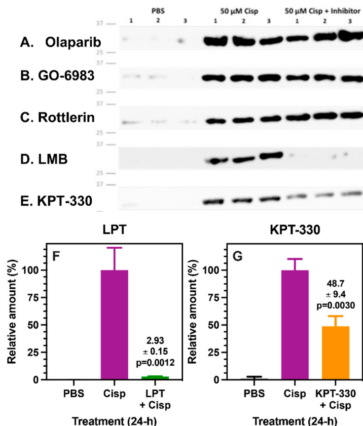
Figure 6. Cisplatin mediated high mobility group box 1 (HMGB1) secretion is regulated by nuclear exportin 1 (XPO1). Representative anti-HMGB1 immunoblots from biological replicates (n=3) of A549 cell culture media using anti-HMGB1 rabbit pAb against the C-terminal acidic tail of HMGB1. (A) Olaparib (50 μM) (B) GO-6983 (120 nM), and (C) Rottlerin (100 μM) treatments showed no effect on cisplatin (50 μM) mediated HMGB1 secretion from A549 cells. Conversely, XPO1 (chromosomal maintenance 1; CRM1) inhibitors (E) leptomycin B (LMB) (4.5 nM) and (E) KPT-330 (75 nM) significantly attenuated cisplatin mediated HMGB1 secretion. Normalized immunoblot quantification of HMGB1 in A549 cell culture media comparing effects of XPO1 inhibitors on cisplatin mediated HMGB1 secretion. (F) LMB (4.5 nM). (G) KPT-330 (75 nM). Significant differences were determined using an unpaired Student's t-test). Error bars show ± SD.
