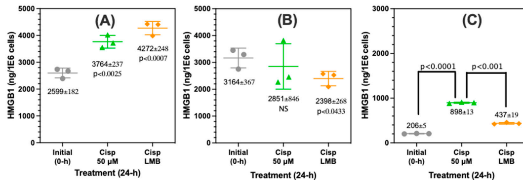
Figure 7. Increased cisplatin mediated nuclear HMGB1 accumulation and decreased secretion after inhibition of nuclear transporter 1 (XPO1). HMGB1 levels were quantified in A549 cells by nano liquid chromatography-parallel reaction monitoring/high resolution/mass spectrometry in A549 subcellular fractions and A549 cell media after treatment with 50 μM cisplatin and a combination of 50 μM cisplatin with 4.5 nM leptomyacin B (LMB). (A). Nuclear fraction. (B) Cytosolic fraction. (C) Cell media. Values are mean ± standard deviation. Statistical analysis was conducted using an unpaired student's t-test.
