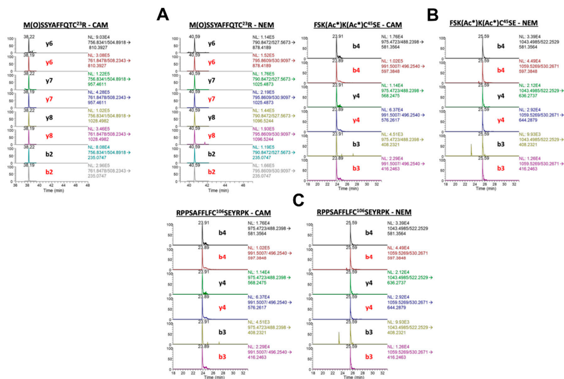
Figure 5. Nano liquid chromatography parallel reaction monitoring/high-resolution mass spectrometry analysis of Cys-containing peptides from cisplatin treated A549 media. Chromatograms show corresponding light (black) and heavy (red) transitions. Carbamidomethyl (CAM)-modified transitions indicate free (reduced) Cys proteoforms and N-ethyl maleimide (NEM)-modified transitions indicate disulfide (oxidized) Cys proteoforms. (A) tryptic peptide M(O)SSYAFFQTC 23 R with CAM-modified transitions (left) and NEM-modified transitions (right). (B) Glu-C peptide FSK(Ac*)K(Ac*)C 45 SE with CAM-modified transitions (left) and NEM-modified transitions (right). (C) tryptic peptide RPPSAFFLFC 106 SEYRPK with CAM-modified transitions (left) and NEM-modified transitions (right).
