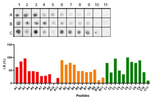
Figure 5. Performance of the mutated and non-mutated RBA IgA-epitopes as a target in a membrane synthesized peptide. The Spot-synthesis membrane immunoassay was prepared as described before to detect human IgA in sera collected during the first phase of the pandemic (A, red), after vaccination (B, orange; AstraZeneca), and during the mutated COVID-19 appeared (C, 2nd phase, green). Epitope SC/14huA (Spot A1, B1 and C1; GGGYADSFVIRGDGG), epitope SC/16huA (Spot A2, B2 and C2; WNANLDSKVGGNYN), epitope SC/17huA (Spot A5, B5 and C5; GGG LKPFER DISTGG). Epitope X (Spot A7, B7 and C7; PLRSYSFRPPYGVGH), epitope Omicron BA.1 and Omicron BA2.12.1 (Spot A8, B8 and C8; PLQSYGFRPTYGVGH) Omicron BA.4 (Spot A9; PLQSYG FRPTYGV GH) and BA.5 (Spot A10; PLQSYGFRPTYGVGH). The distribution of the synthesized peptides in the membranes is presented in Table S3.
