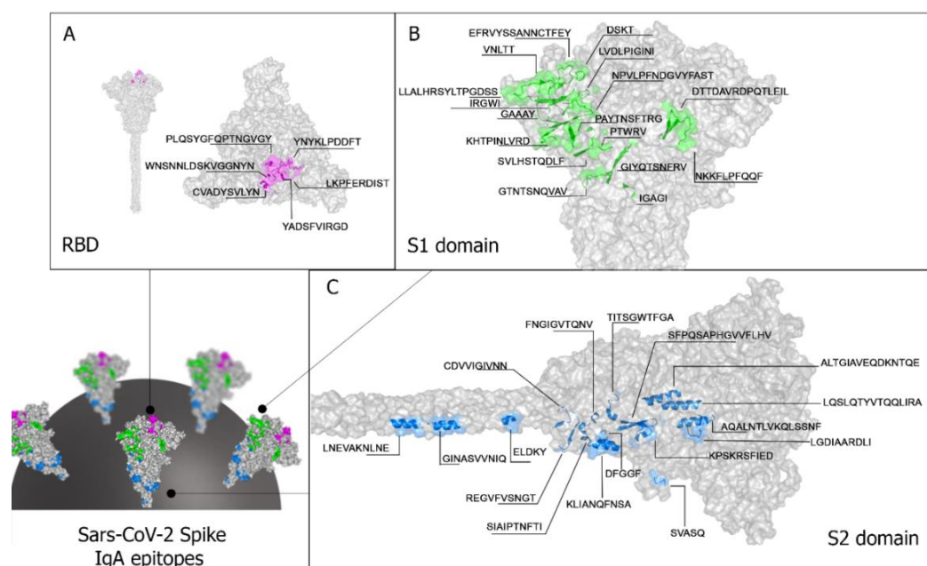
Figure 3. Spatial distribution of IgA reactive epitopes. The figure depicts the spatial positioning of IgA reactive epitopes within the Receptor-Binding Domain (RBD) (A), the S1 domain (B), and the S2 domain of the spike protein. No IgA epitope was identified within the protein's transmembrane (TM) domains (aa1213-1237). The 3D conformation and structure of the protein were obtained from I-Tasser ( https://zhanggroup.org/I-TASSER/ ).
