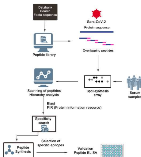
Figure 1. Schematic representation of the strategy used to identify and select SARS-CoV-2 IgA epitopes. Peptide libraries of 15 mer with overlapping of 10 residues were constituted using a software and the positive peptides revealed with patients sera and secondary labelled antibodies. The chemiluminescent positive spots were quantified using a scanner and those with the best performance listed according to their hierarchical position using a software. The possible cross reactivity of the epitopes was checked in databanks and those considered specific were synthesized as single or multi epitopes peptides and validated by ELISA.
