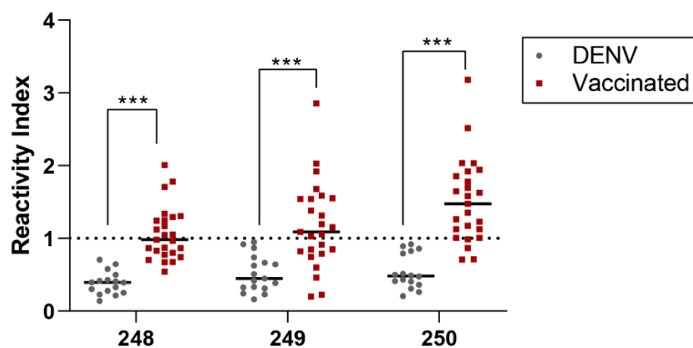
Figure 6. pELISA assays for IgA using Spike pep-248 (GSYADSFVIRDGGSG), pep-249 (GSNNSN NDSKVGSGS) and pep-250 (GSLKPFERDISTGSG) and sera from COVID-19 vaccinated (n=25) and DENV-positive samples (n= 16; pre-pandemic). Data shows the reactivity index of samples. Kruskal-Wallis's test was applied to identify statistical differences, followed by Dunn's multiple comparisons tests. Significant differences were considered with p < 0.05 .
