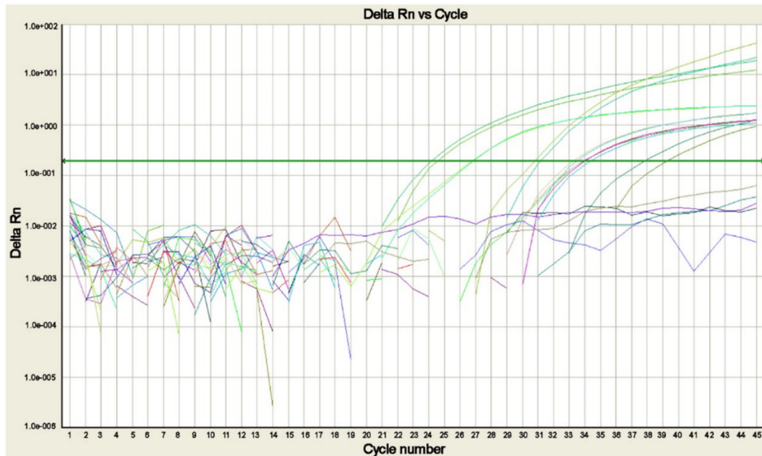
Figure 3. Real-time PCR amplification plot for Plasmodium DNA detected in blood samples of patients with suspected malaria. The plot shows the amplification of P. falciparum , P. malariae , P. ovale curtisi , P. ovale wallikeri , and P. vivax positive controls and of the sample positive for P. falciparum , each tested in duplicate [modified from 14].
