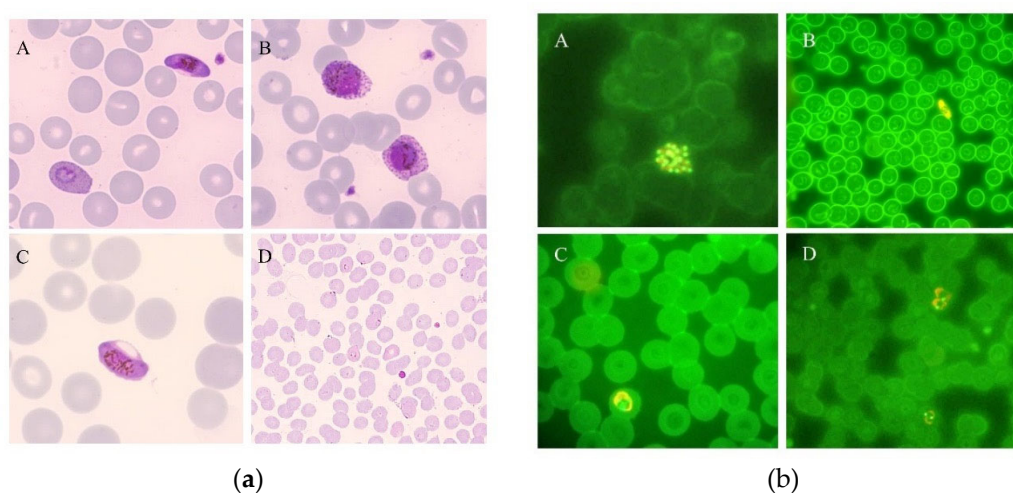
Figure 1. (a). Thin blood smears of blood samples from malaria cases prepared and stained with Giemsa. (A) P. falciparum gametocyte and P. ovale trophozoite (100 \times ). (B) P. ovale gametocytes (100 \times ). (C) P. falciparum gametocyte (100 \times ). (D) P. falciparum trophozoites (40 \times ). (modified from [14]). (b). Thin blood smears of blood samples from malaria cases prepared and stained with acridine orange. (A) P. vivax schizont (100 \times ). (B) P. falciparum gametocyte (40 \times ). (C) P. ovale trophozoite (100 \times ). (D) P. vivax trophozoites (100 \times ). (modified from [14]).
