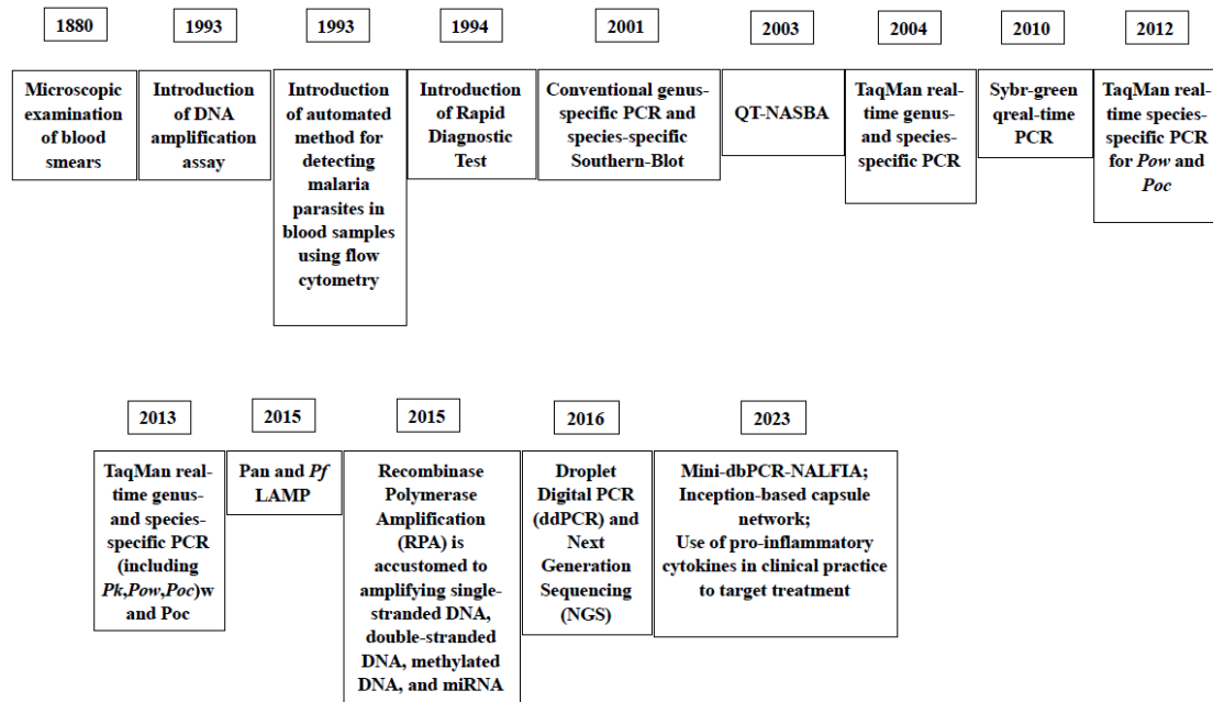
Figure 4. Milestones of the introduction of laboratory assays for the diagnosis of malaria through the years. [41,72,73,81–84,108,115,116,119].
