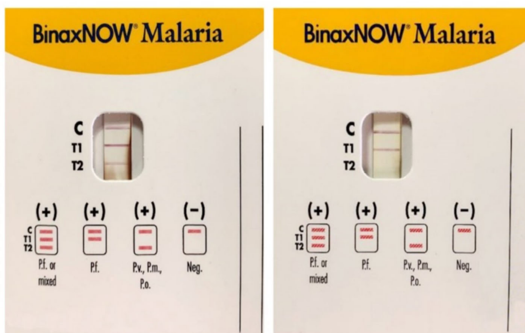
Figure 2. Immunocromatographic assay for the detection of Plasmodium sp. antigens in blood samples: P. falciparum ( Pf ), P. malariae ( Pm ), P. vivax ( Pv ), and P. ovale ( Po ). C is the control line for human blood, T1 line specific to P. falciparum ( Pf ) Histidine-Rich Protein2 (HRP2), and T2 line is for the parasite lactate aldolase. A Pf or mixed infection on the left and a Pf infection on the right [modified form14].
