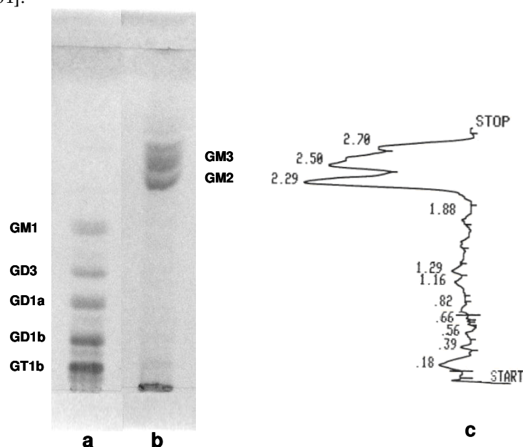
Figure 5. High performance thin-layer chromatography of gangliosides extracted from: (a) HB and (b) BMLA; (c) densitometric quantification of ganglioside fractions from BMLA. Reprinted permission from [164].
