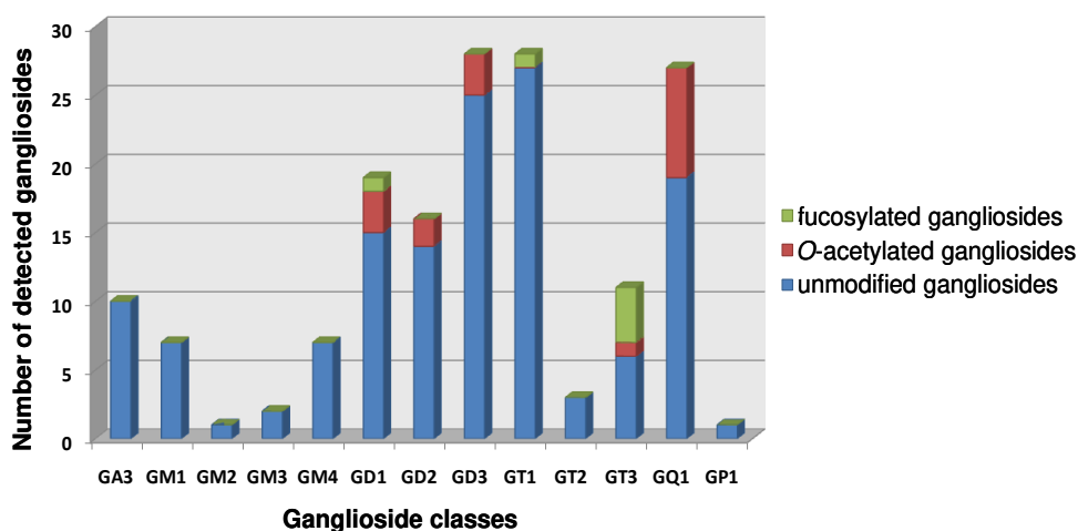
Chart 1. Chart plotting the number of the identified ganglioside species in GBM according to the composition of their glycan core and the sialylation degree. Reprinted permission from [139].
