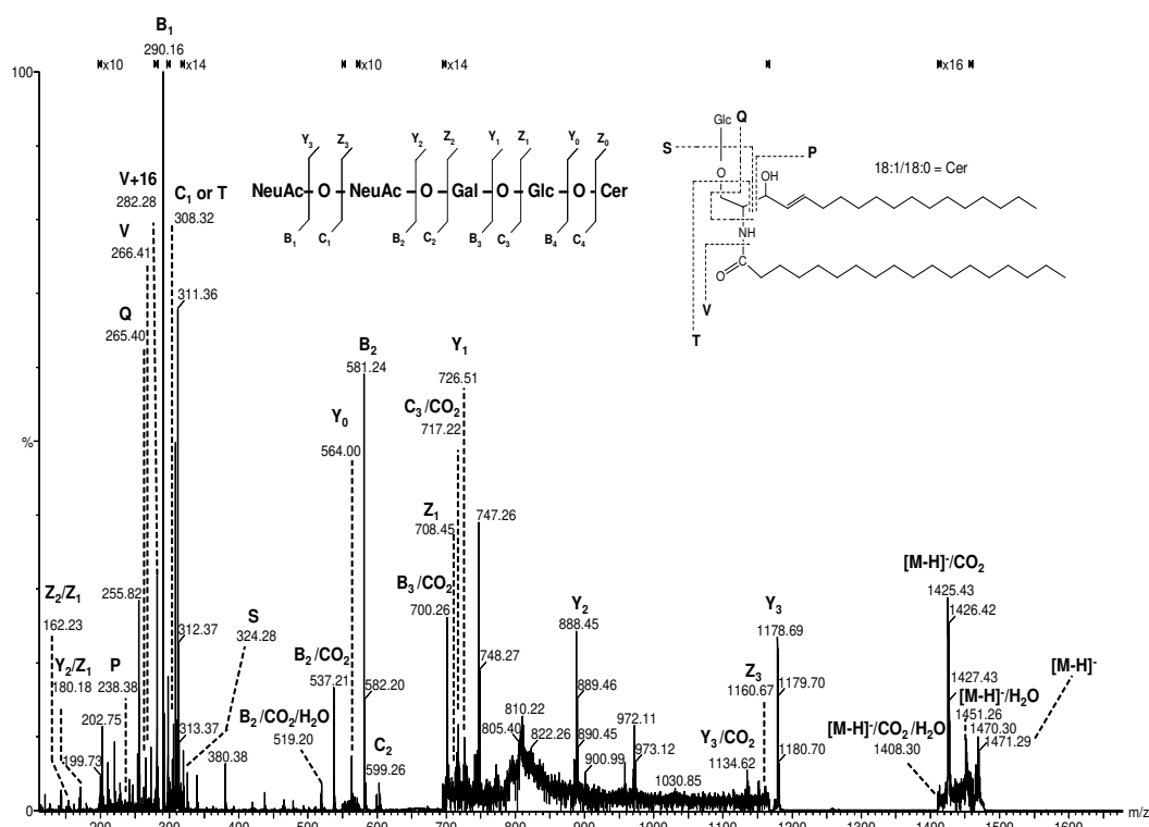
Figure 7. (-) Chip-nanoESI QTOF CID MS/MS of the singly charged ion at m/z 1471.29 corresponding to GD3 (d18:1/18:0) from BMLA. Acquisition time 1 min. Insets: fragmentation schemes of the oligosaccharide core and ceramide moiety. Reprinted permission from [164].
