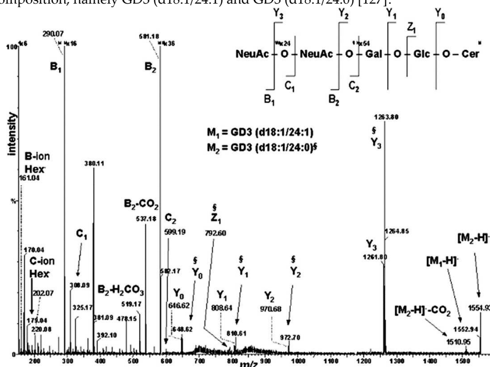
Figure 4. Negative ion mode nano-ESI-QTOF MS/MS of the [M-H]^{-2} ions at m/z 1552.94 and m/z 1554.93 corresponding to the GD3 (d18:1/24:1) and GD3 (d18:1/24:0), respectively. Solvent, methanol; ESI voltage; 1000–1250 V; for precursor ions isolation the LM and HM parameters were set to 3; collision energy; 30–45 eV; collision gas pressure: 15 psi; acquisition: 3 min; average sample consumption: 1 pmol. Inset, the fragmentation scheme of GD3. Reprinted with permission from [127].
