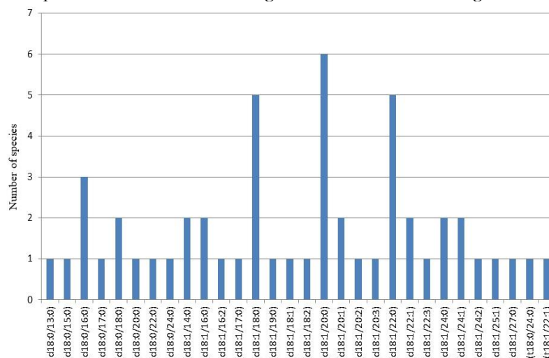
Figure 1. Plot of the number of gangliosides species in cavernous hemangioma vs. ceramide compositions. Reprinted with permission from [57].
