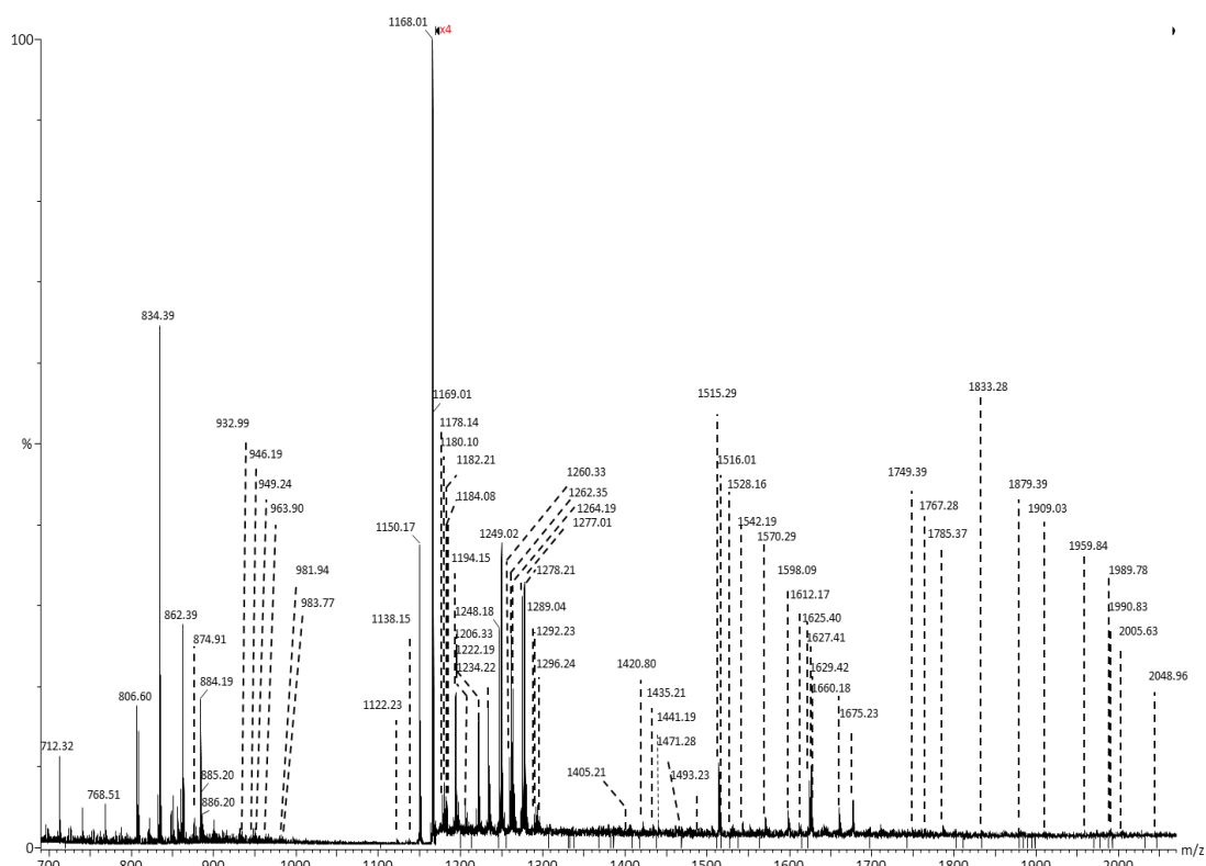
Figure 6. (-)Chip-nanoESI QTOF MS of the native ganglioside mixture extracted from BMLA. Solvent: MeOH; sample concentration 2.5 pmol/ \mu L; acquisition time 1min; Chip ESI: 1.5 kV; Cone voltage: 45 V. Reprinted permission from [164].
