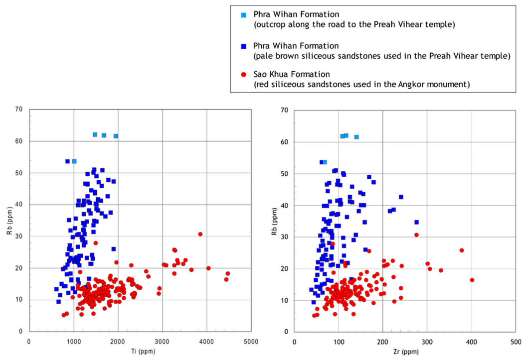
Figure 6. Relationships between minor element (Rb, Ti, and Zr) contents in sandstones from the Phra Wihan and Sao Khua formations, determined using pXRF.
