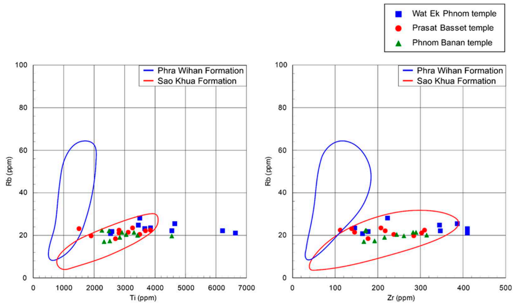
Figure 9. Relationships between minor element (Rb, Ti, and Zr) contents in red siliceous sandstones used in the investigated temples.
