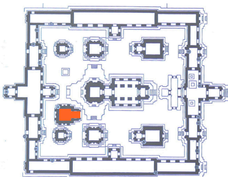
Figure 4. Plan of the Phnom Chisor temple. The shrine with gray sandstone blocks is colored red [13].
