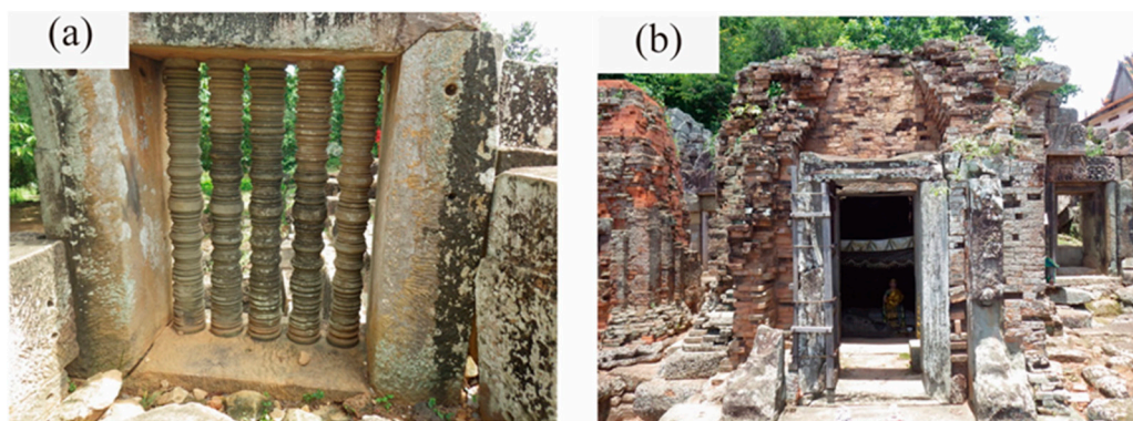
Figure 3. Gray sandstone used in (a) a lattice window in the Wat Ek Phnom temple, and (b) a door frame of the Phnom Chisor temple.
