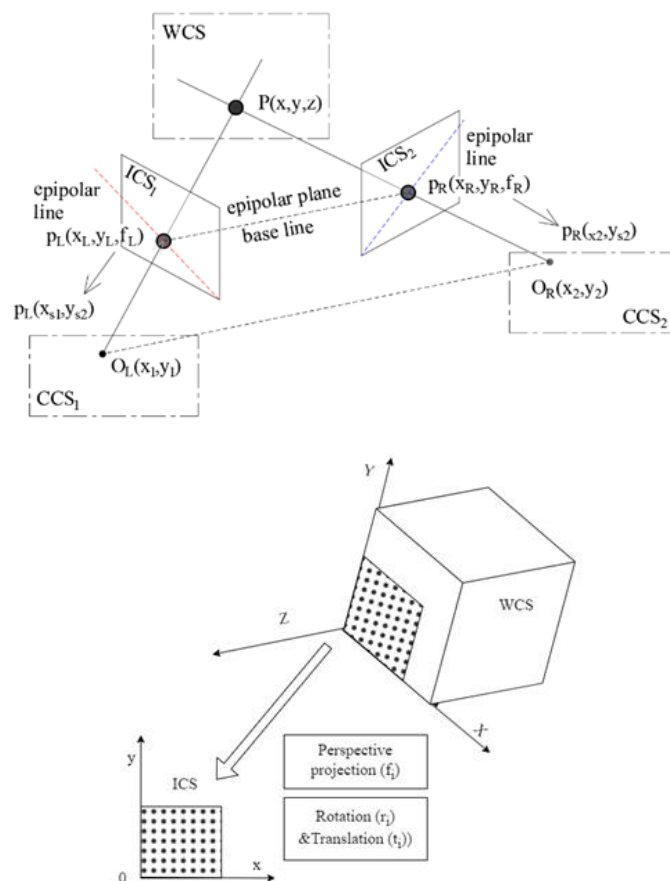
Figure 3. Scheme of image translation between coordinate systems in DIC approach: WCS-world coordinate system, ICS-image coordinate system, CCS-camera coordinate system, P- point in physical 3D-space, p_L(x_L, y_L, f_L) and p_R(x_R, y_R, f_R) -its projections for left and right camera, respectively; p_L(x_{s1}, y_{s1}) and p_R(x_{s2}, y_{s2}) -coordinates in sensor system of left and right camera; O_L and O_R - origins of left and right cameras; f_i -focal length (projection component), r_i , t_i -rotation and translation components of displacement.
