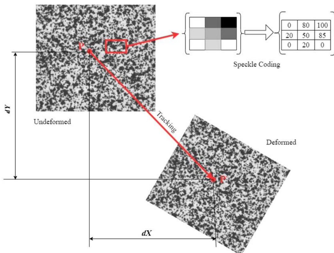
Figure 2. Principle of grey level coding and subset tracking in the DIC method: P-initial position of a point on the reference (undeformed image), P'-position after deformation; P-P'(dX, dY)- displacement of Point P.
