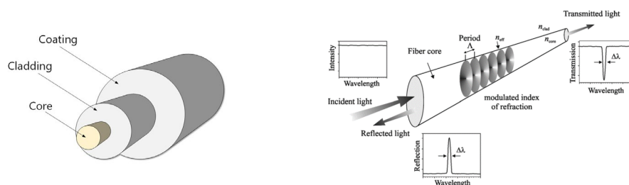
Figure 2. Schematic representation of a fiber and Fiber Bragg Grating inscribed into the core of an optical fiber.
