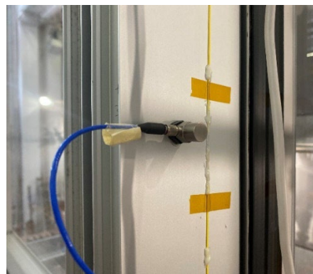
Figure 12. Accelerometer applied on aluminum mullion.
