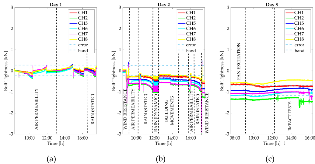
Figure 25. Strain gauge-based force washers data collected during the 3 days: day 1 (a); day 2 (b); day 3 (c).
