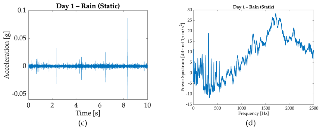
Figure 21. Day 1 tests: respectively story time and power spectrum for each test: air permeability acceleration/time (a); air permeability power spectrum /frequency (b); rain (static) acceleration/time (c); rain (static) power spectrum /frequency (d).
