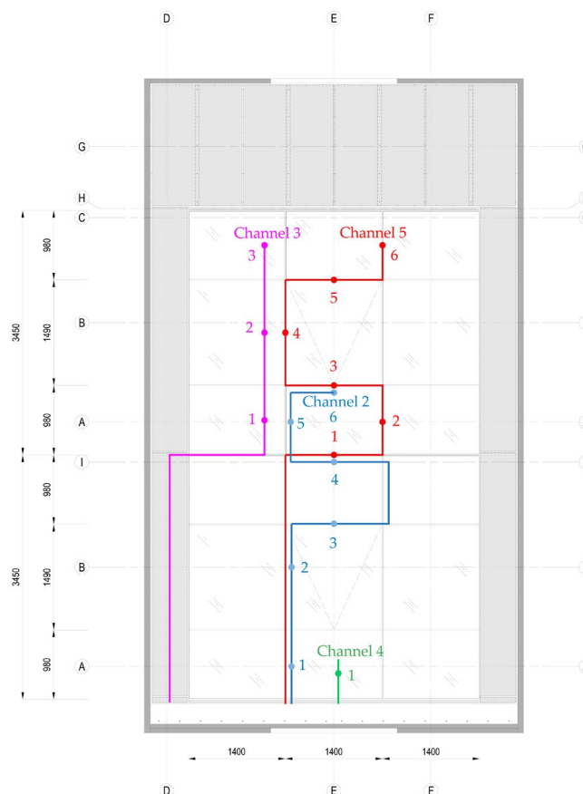
Figure 4. Scheme of FBGs channel position.
