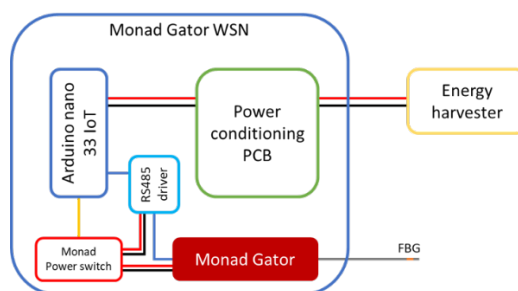
Figure 3. Scheme of InComEss architecture.
