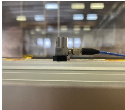
Figure 11. Accelerometer applied on aluminum transom.
