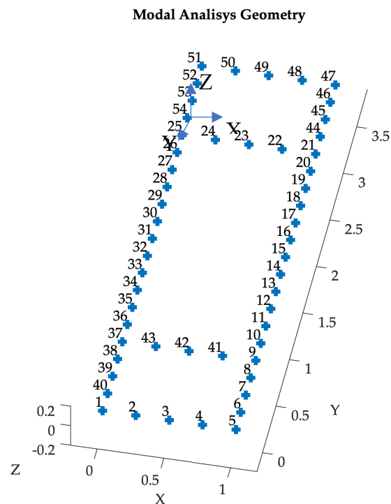
Figure 15. Modal analysis geometry.
