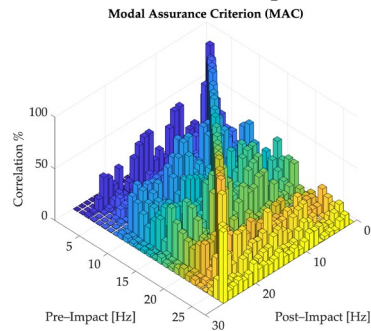
Figure 17. MAC (Modal Assurance Criterion) between the two performed modal analysis.
