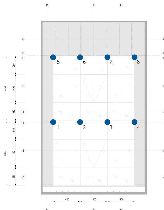
Figure 6. Force washers' positions.
