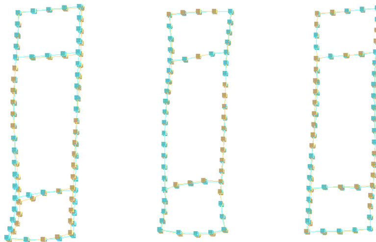
Figure 19. Three modal shapes comparison between pre-compliance test and post-compliance test.
