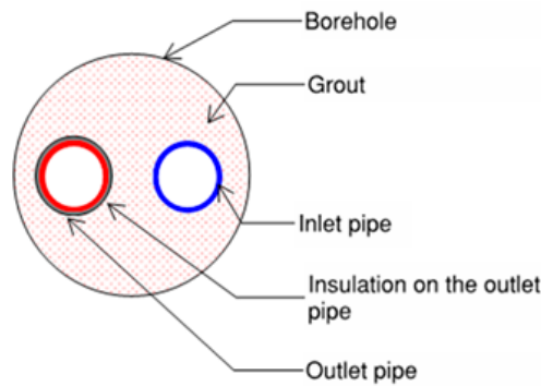
Figure 5. U-tube BHX with insulated outlet pipe
