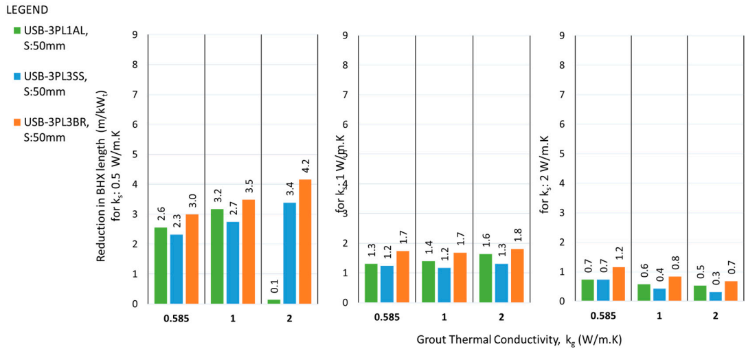
Figure 23. Reduction in the BHX length for various U- barriers; k_s : 0.5 W/m.K
