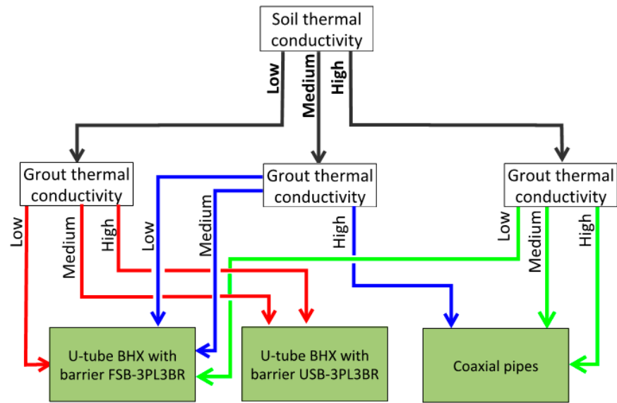
Figure 28. Decision tree for the type BHX for the minimum length.
