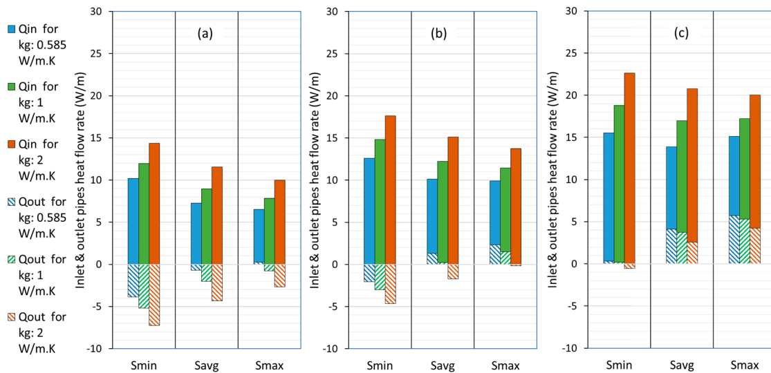
Figure 10. Heat transfer from U-tube BHX Inlet & Outlet legs; (a) for k_s : 0.5 W/m.K (b) for k_s : 1 W/m.K (c) for k_s : 2 W/m.K
