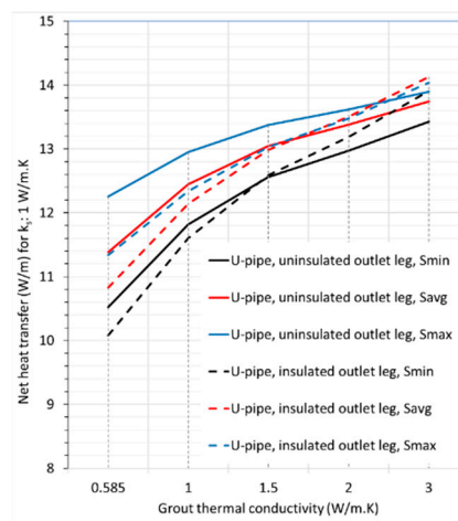
Figure 11. Comparison of Net heat transfer for uninsulated U-tube and U-tube with insulated outlet leg; k_s : 1 W/m.K
