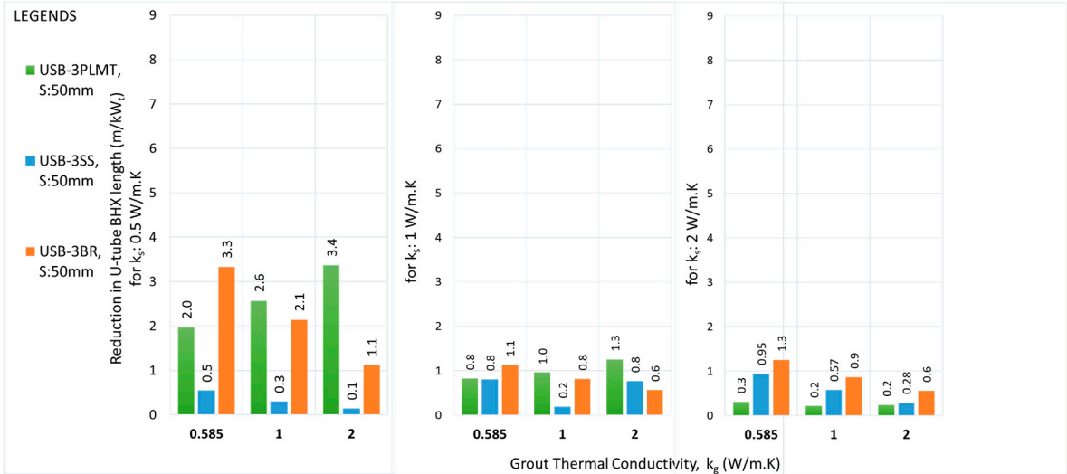
Figure 22. Reduction in the BHX length for various single U- barriers; k_s : 2 W/m.K.
