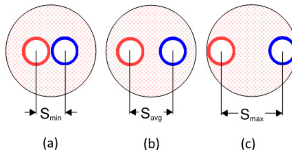
Figure 4. Various shank spacings of U-tube BHX model
