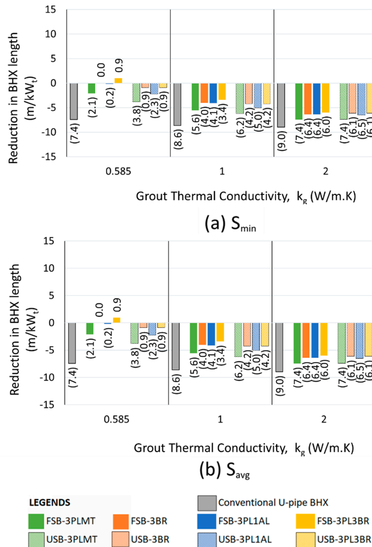
Figure 27. Reduction in length for various arrangements of U-tube BHX compared to coaxial pipes; k_s : 2 W/m.K, (a) S_{\min} (b) S_{\text{avg}}
