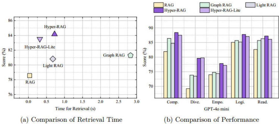
Figure 7. Efficiency Comparison of Different Augmentation Methods. a , Comparison of performance and time. The performance is obtained by scoring-based assessment on the NeurologyCrop dataset, where each method’s performance is the average of five indicators. The average retrieval time for RAG, Graph RAG, Light RAG, Hyper-RAG, and Hyper-RAG-Lite are 0.033s, 2.83s, 0.67s, 0.72s, and 0.31s respectively. b , Specific scores of the five indicators on the NeurologyCrop dataset.
