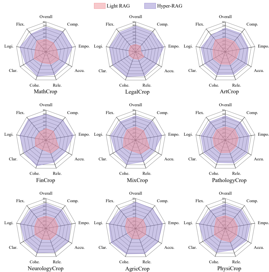
Figure 6. Experimental results across diverse domain datasets. This figure presents the experimental outcomes of two methods evaluated on datasets from various domains. We utilize a Selection-Based Assessment approach, employing eight distinct indicators to measure and compare the performance of the methods. The Overall score is calculated as the average of these eight evaluation metrics, providing a comprehensive assessment of each method’s effectiveness. The results illustrate how the two methods perform across different domain-specific challenges, highlighting their relative strengths and areas for improvement based on the aggregated evaluation criteria.
