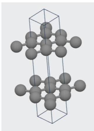
Figure 2. Primitive unit cell of hexagonal graphite obtained by Materials Project.[17].
