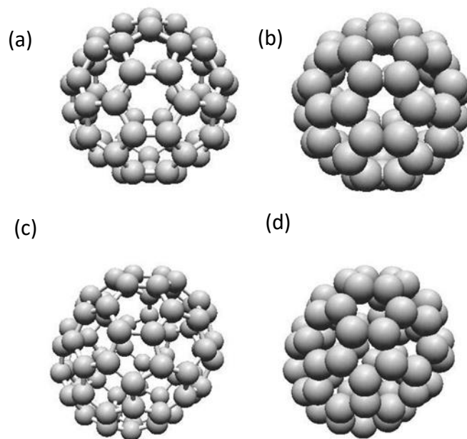
Figure 5. (a) Ball-and-stick model of fullerene C_{60} , (b) Sphere-in-contact model of fullerene C_{60} , (c) Ball-and-stick model of fullerene C_{70} D_{5h} and (d) Sphere-in-contact model of fullerene C_{70} D_{5h} . Image produced in Nanotube Modeler Software.
