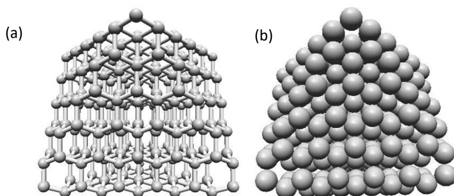
Figure 9. (a) Ball-and-stick model and (b) Sphere-in-contact model of nanodiamond. Image produced in Nanotube Modeler Software.
