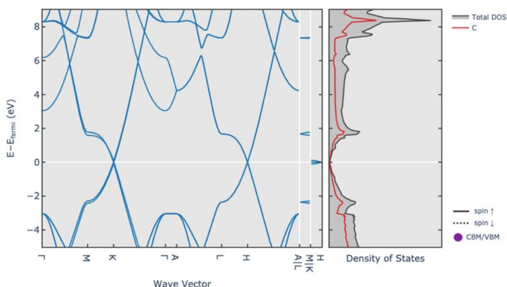
Figure 3. Band structure and density-of-states plot of hexagonal graphite using DFT calculations done by the Materials Project.[17,18].
