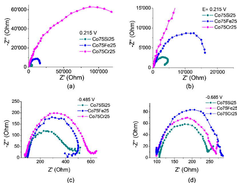
Figure 7. Nyquist curves for electrocatalyst samples Co75Si25, Co75Fe25, and Co75Cr25 in 12 mM \text{NaNO}_3 with 0.05 M \text{Na}_2\text{SO}_4 at the following potentials (vs. RHE): (a) 0.215 \text{ V} ; (b) 0.215 \text{ V} (for the enlarged fragment); (c) -0.485 \text{ V} ; (d) -0.685 \text{ V} .
