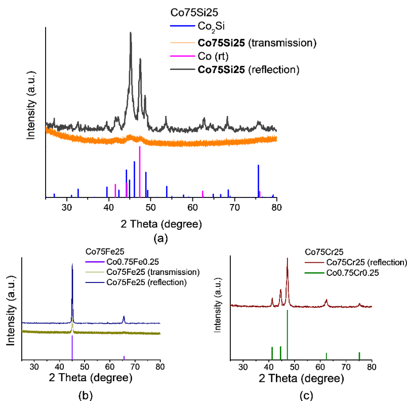
Figure 2. XRD patterns for electrocatalyst samples: (a) Co 75 Si 25 (eutectic alloy); (b) Co 75 Fe 25 (solid solution); (c) Co 75 Cr 25 (solid solution). Pictures for both transmission and reflection of X-rays are given.
