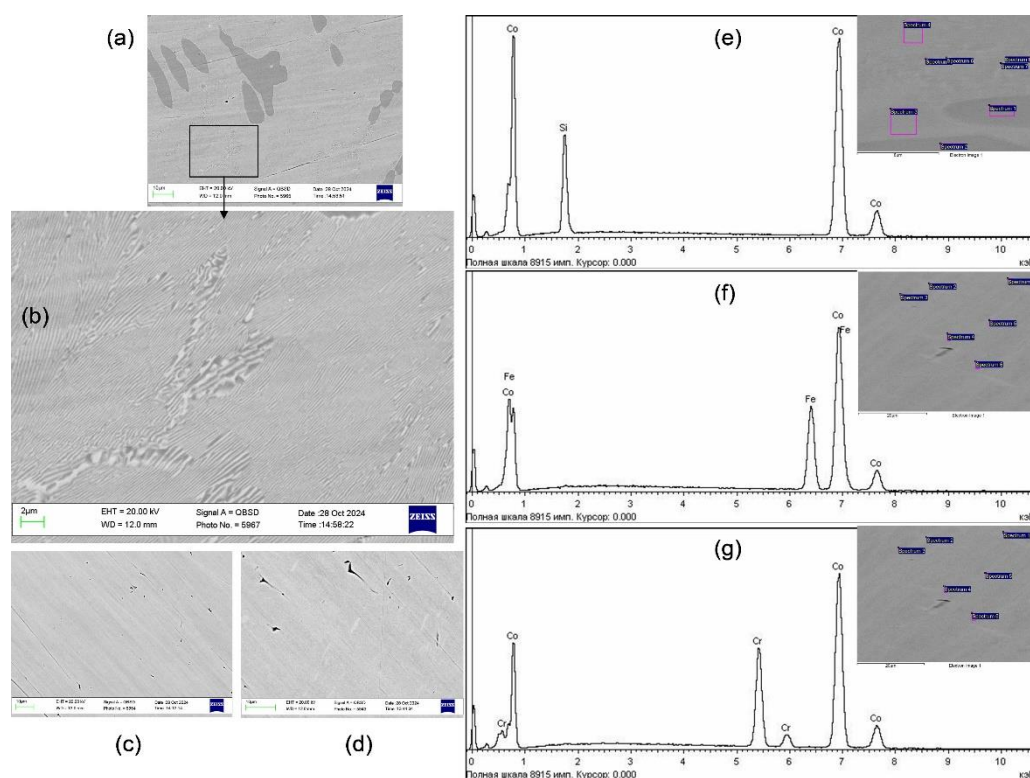
Figure 1. SEM images: (a) and (b) Co 75 Si 25 (eutectic alloy); (c) Co 75 Fe 25 (solid solution); (d) Co 75 Cr 25 (solid solution). EDX elements spectra for: (e) Co 75 Si 25 (eutectic alloy); (f) Co 75 Fe 25 (solid solution); (g) Co 75 Cr 25 (solid solution). Insertion on Fig. 1 e-g demonstrates various locations for the EDX probe.
