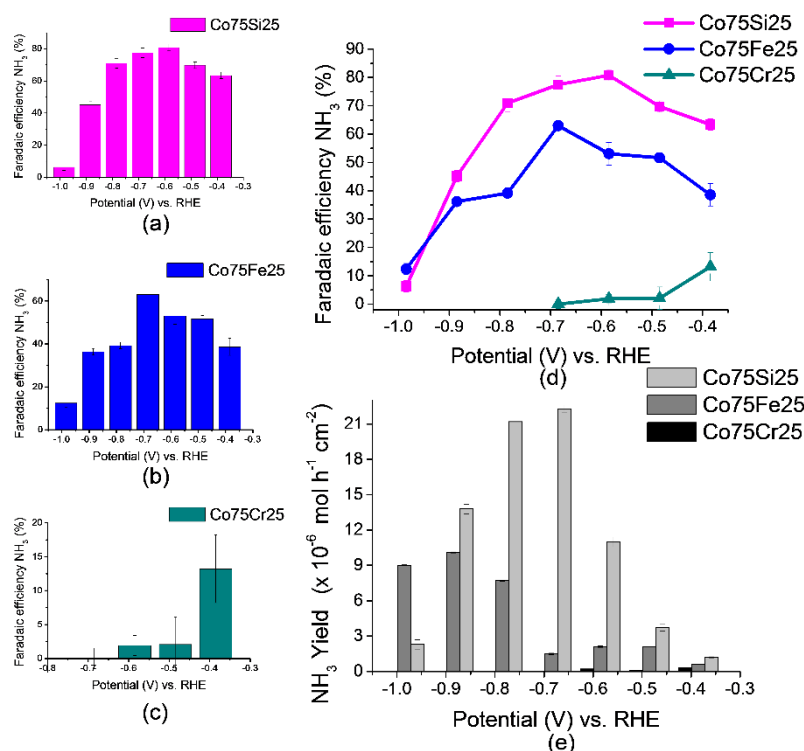
Figure 5. The results of the NO 3 RR study: (a) FE values for Co75Si25, (b) FE values for Co75Fe25, (c) FE values for Co75Cr25, (d) the resulting general FE-graph; and (e) ammonia yield rate of NO 3 RR.
