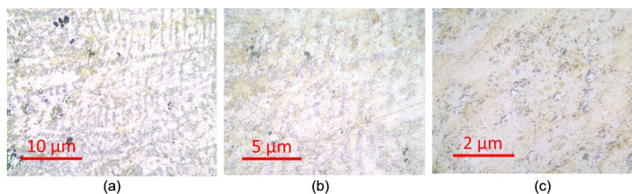
Figure 3. Optical images of the Co 75 Si 25 sample containing the eutectic phase at different magnifications: (a) 200 \times ; (b) 500 \times ; (c) 1000 \times .
