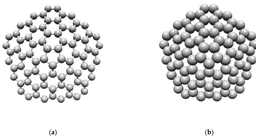
Figure 4. (a) Ball-and-stick model and (b) Sphere-in-contact model of C_{80} carbon nanocone with a cone height of 5 Angstroms and a disclination angle of 60 degrees. Image produced in Nanotube Modeler Software.
