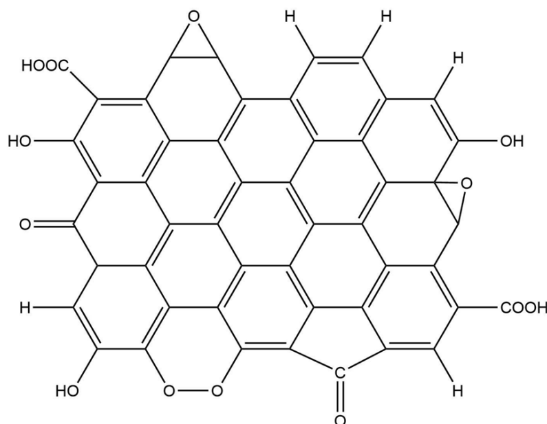
Figure 7. Structure of graphene oxides showing the various functional groups COOH, C=O, -O-O-, OH, =O and -H at the periphery of a carbon sheet. Image drawn in Chemdraw.
