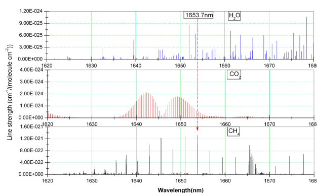
Figure 6. Absorption spectrum of the gases (H 2 O, CO 2 and CH 4 ) obtained from the HITRAN database.
