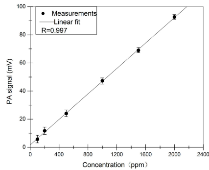
Figure 8. PA signals to different concentrations. Error bars give the range of the corresponding PA signals.
