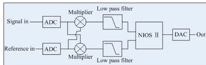
Figure 5. Schematic diagram of the FPGA based lock in amplifier.
