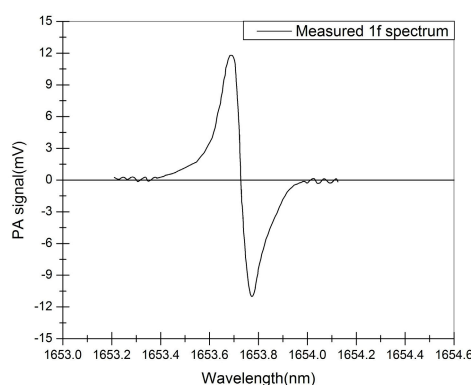
Figure 7. Measured 1f spectra of 200 ppm CH 4 .
