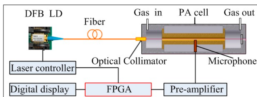
Figure 1. Schematic configuration of the PA methane sensor
