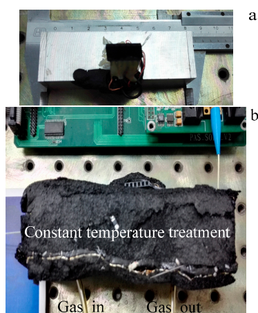
Figure 3. The PA cell and the constant temperature treatment device
