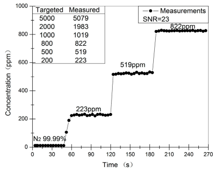
Figure 9. Measured dilution process of the 5000 ppm CH 4 reference concentration.
