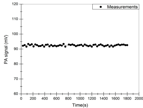
Figure 10. Continuous measurements of 2000 ppm CH 4 .
