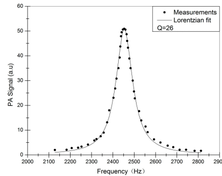
Figure 4. The resonance profiles showing the first longitude resonance frequency is 2450Hz.
