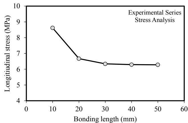
Figure 8. The variation of critical longitudinal stress for different bonding lengths (applied stress for all the specimens: 1000 MPa).
