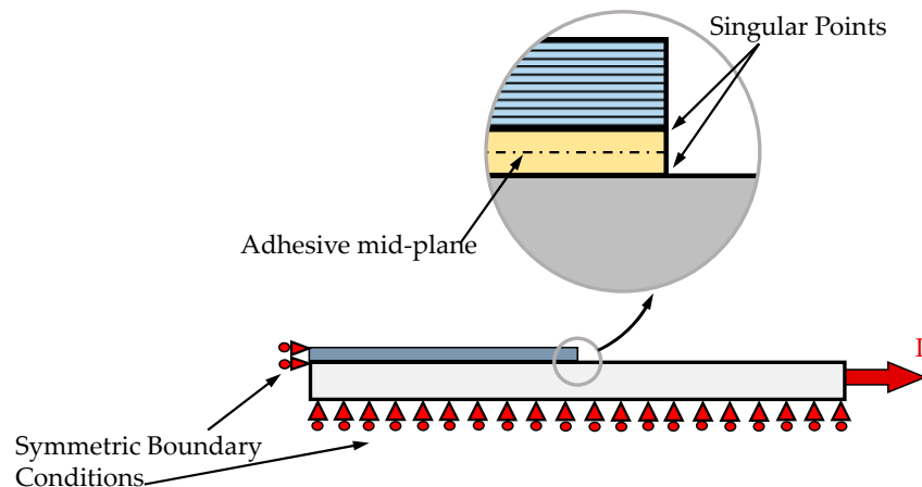
Figure 4. The applied boundary and loading conditions to the finite element model. ( P : applied load)
