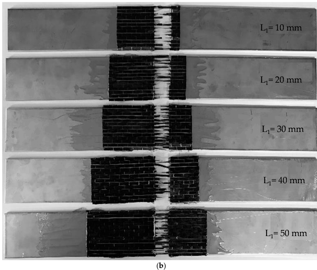
Figure 2. Double strap joints (DSJs) prepared for experiments (a) before the test; (b) after the test.
