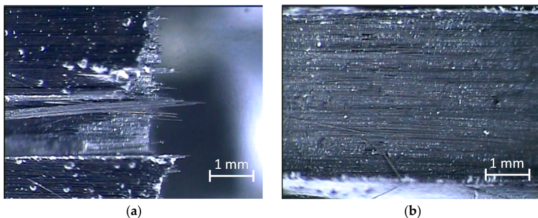
Figure 13. Typical failure mode of loaded steel/CFRP DSJs subjected to quasi-static tensile loading; (a) CFRP rupture; (b) CFRP delamination.
