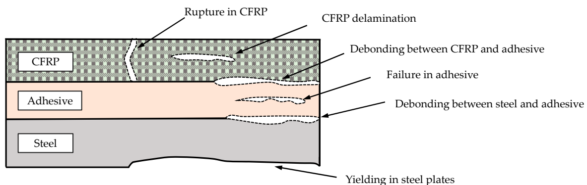
Figure 12. Different types of failure mechanisms in steel/CFRP bonded joint.
