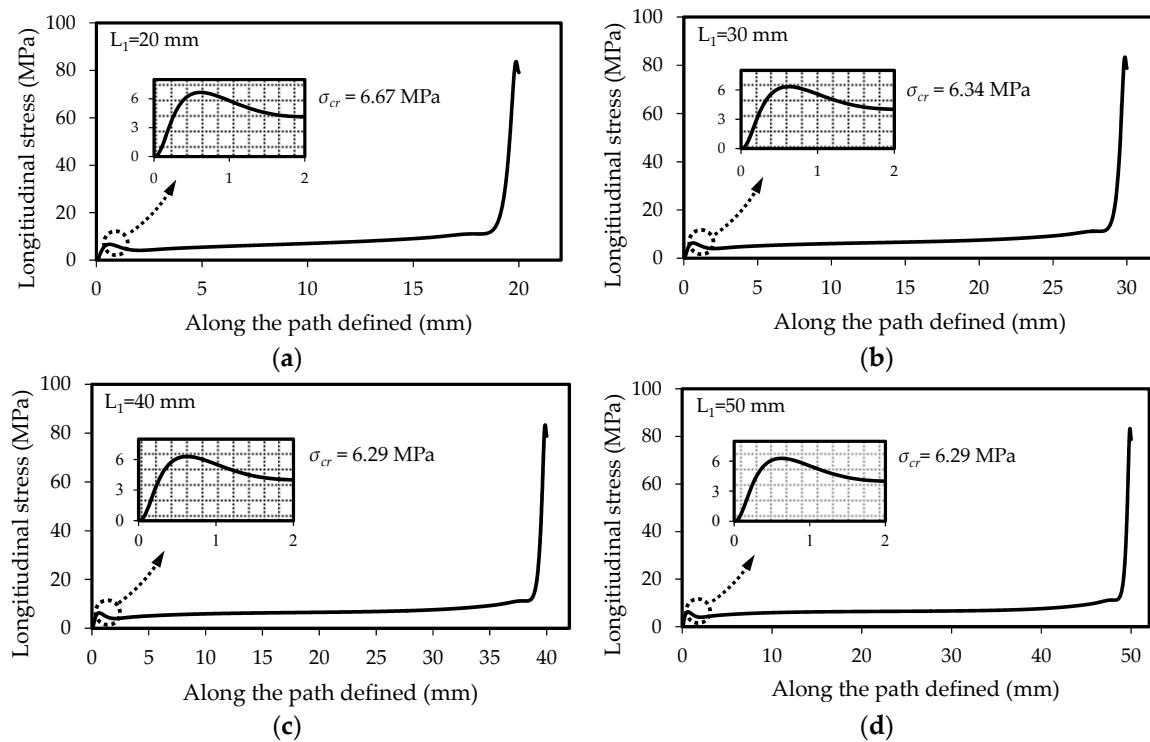
Figure 7. Longitudinal stress distribution along the path defined in the mid-plane of the adhesive layer for the present experimental series—(a) L_1 = 20 mm; (b) L_1 = 30 mm; (c) L_1 = 40 mm; (d) L_1 = 50 mm (applied stress for all the specimens: 1000 MPa).
