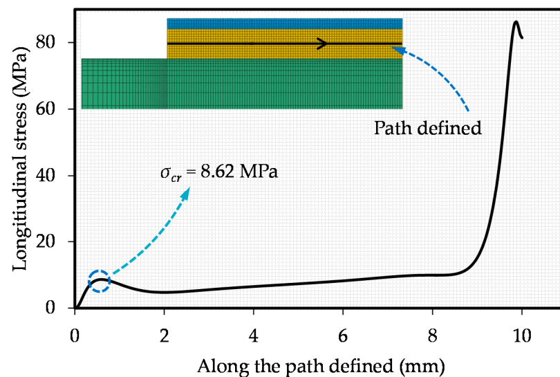
Figure 6. Longitudinal stress distribution along the path defined in the mid-plane of the adhesive layer for the present experimental series— L_1 = 10 mm.
