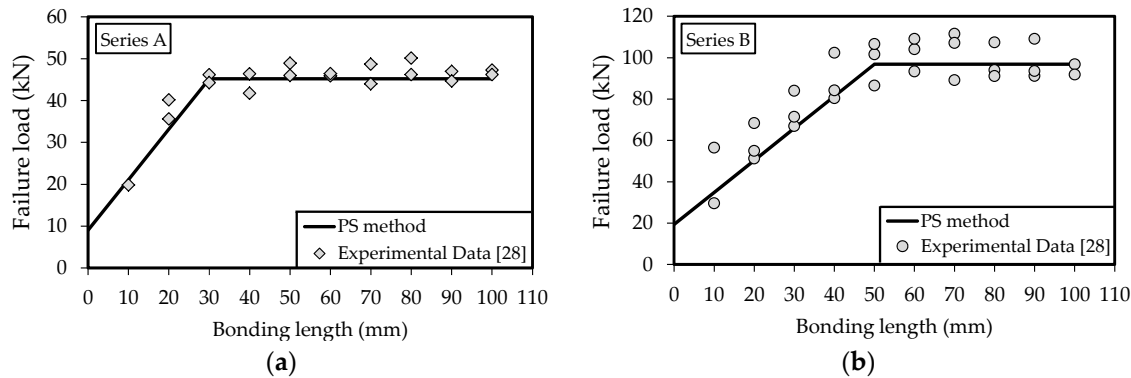
Figure 11. Comparison between the experimental failure loads of DSJs and the theoretical predictions obtained by means of PS method; (a) series A; (b) series B.
