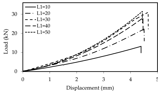
Figure 3. A sample load–displacement curve for the steel/CFRP DSJs under tensile quasi-static loading.
