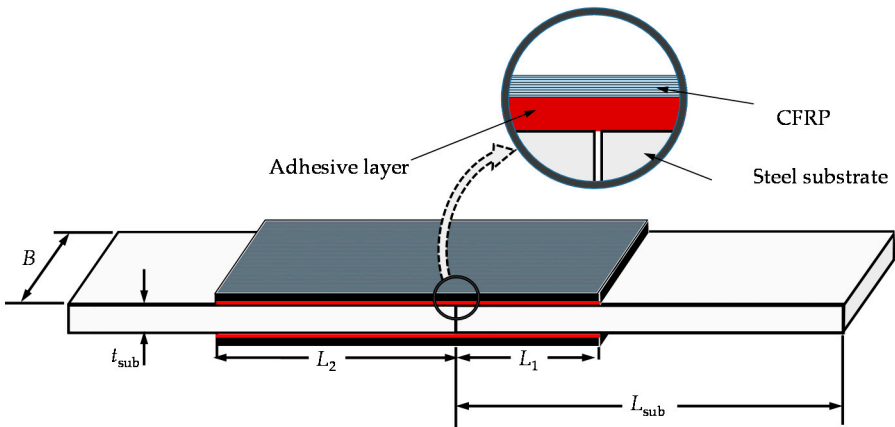
Figure 1. A schematic of steel/CFRP double strap joint.
