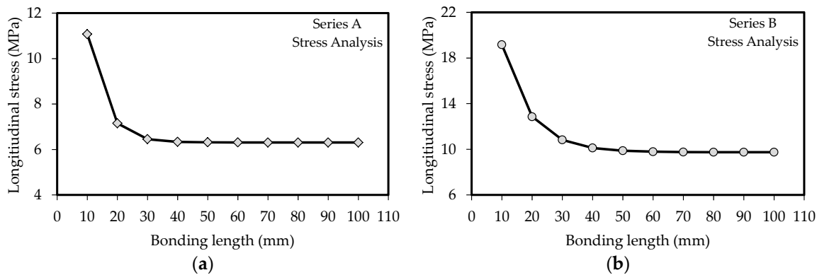
Figure 10. The variation of critical longitudinal stress for different bonding lengths (applied stress for all the specimens: 1000 MPa); (a) series A; (b) series B.
