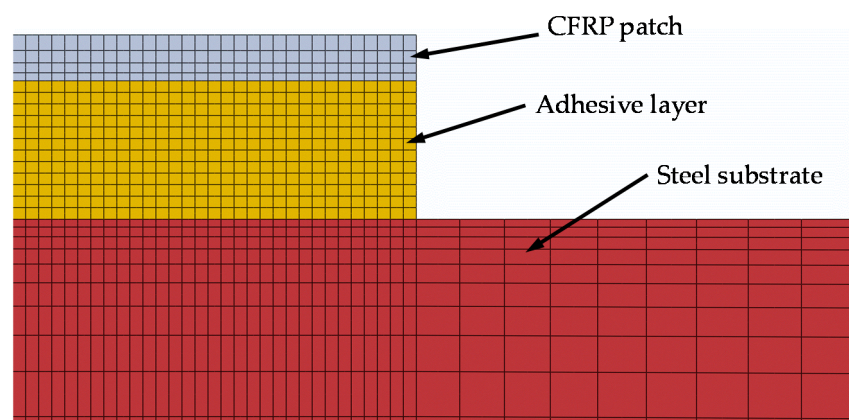
Figure 5. A typical mesh pattern used for DSJ models.
