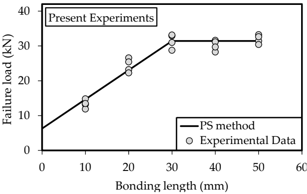
Figure 9. Comparison between the experimental failure loads of DSJs and the theoretical predictions obtained by means of point stress (PS) method.
