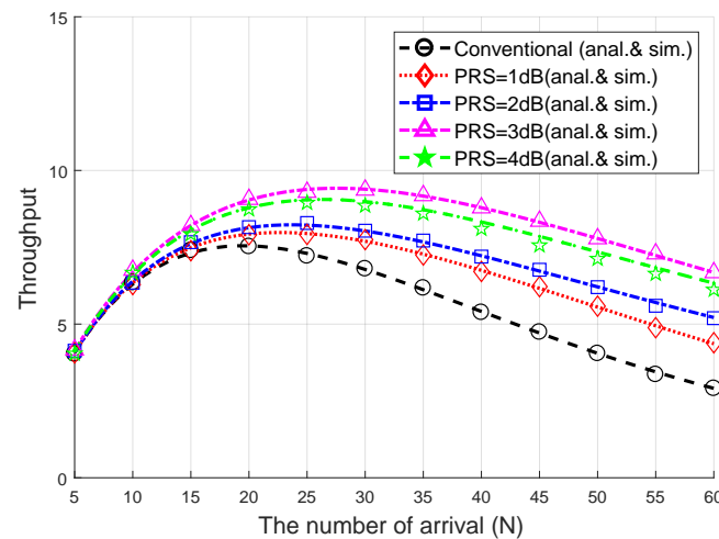
Figure 6. Steady-state RA throughput in terms of PRS
