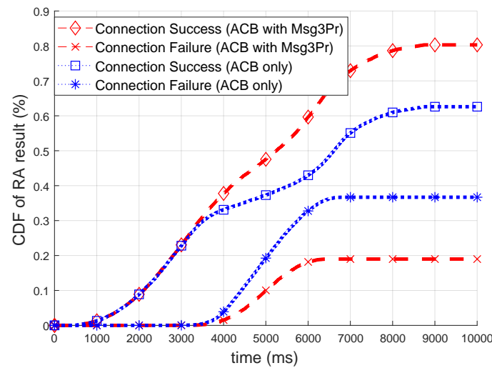
Figure 11. CDF of RA results when optimal ACB is used.
