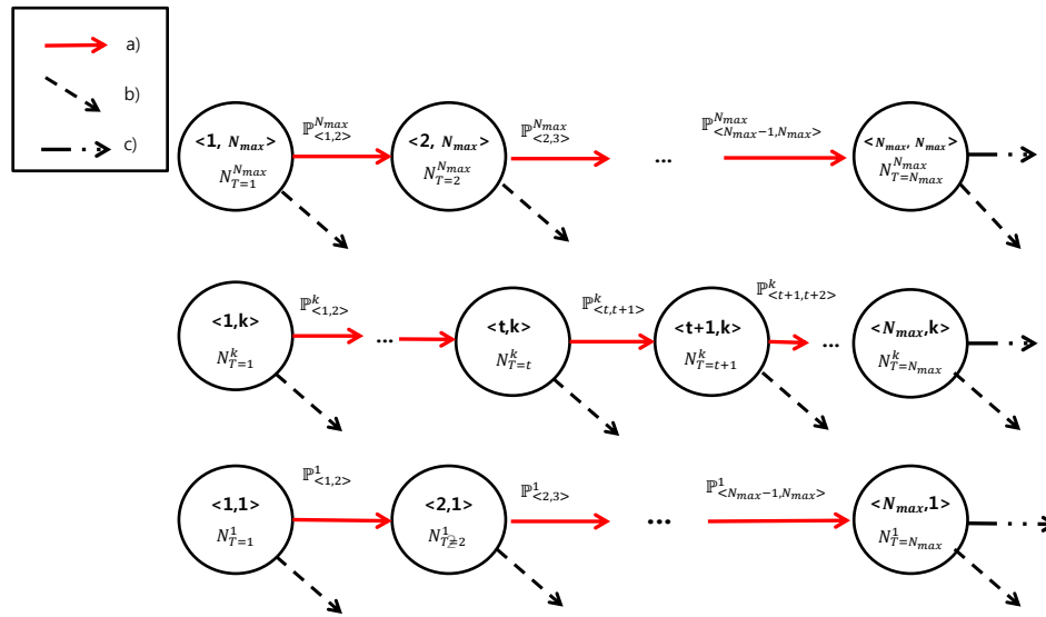
Figure 2. Markov chain model of the devices. State \langle t, k \rangle indicates that the devices with the trial number T_u = t and Z_u = k . Note that state transitions occur when a) RA failure, b) RA success, and c) connection failure occurs, respectively.
