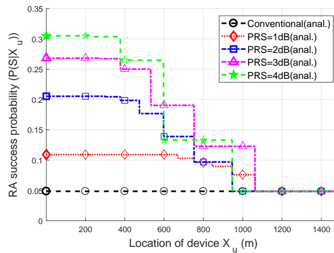
Figure 5. RA success probability according to the location of the device with N = 60 . i.e., \mathbb{P}(S_u|N = 60, X_u = x) .
