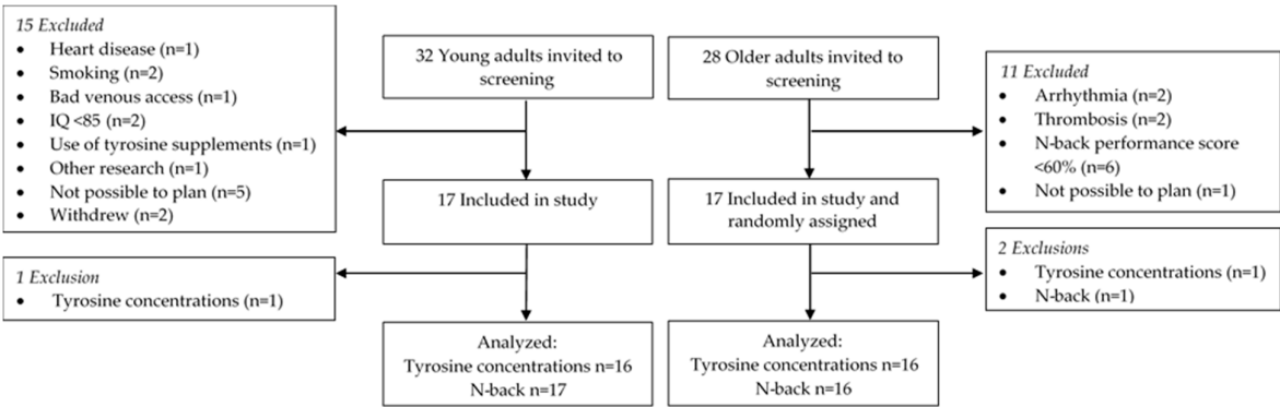
Figure 3. Flowchart of participants through the study
