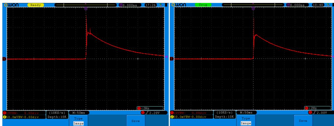
Figure 7. Peak amplitude after 1 hour (642 cycles) and after 100,000 cycles. Vertical 10V per cm, Horizontal 50ms per cm
