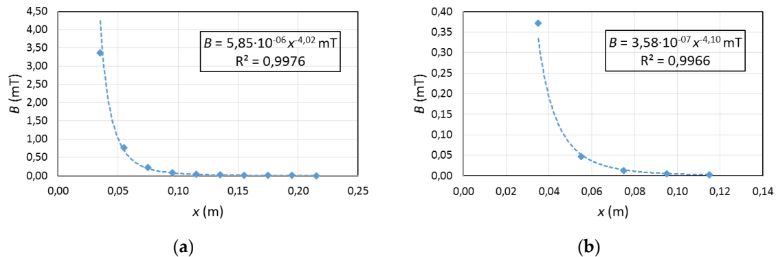
Figure 5. (•) Experimental measures of the magnetic field and (--) potential adjustment of the experimental measures for: a) magnetic quadrupole composed of two neodymium rings; b) magnetic quadrupole composed of two ceramic magnets
