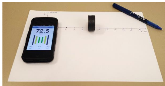
Figure 4. Experimental assembly: a smartphone, a sheet of paper and two identical magnets pasted by their two north poles.
