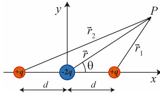
Figure A.1. Linear electric quadrupole: geometry necessary for the calculation of the electric potential at a distance \vec{r} from the center of the quadrupole. The angle \theta is the one that forms the vector \vec{r} with the x -axis and is the one that appears as an argument of the Legendre polynomials in the series development.
