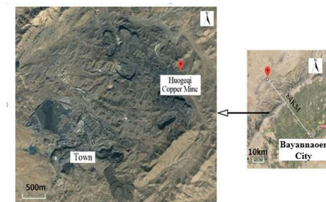
(a) Location of the Huogeqi Copper Mine
