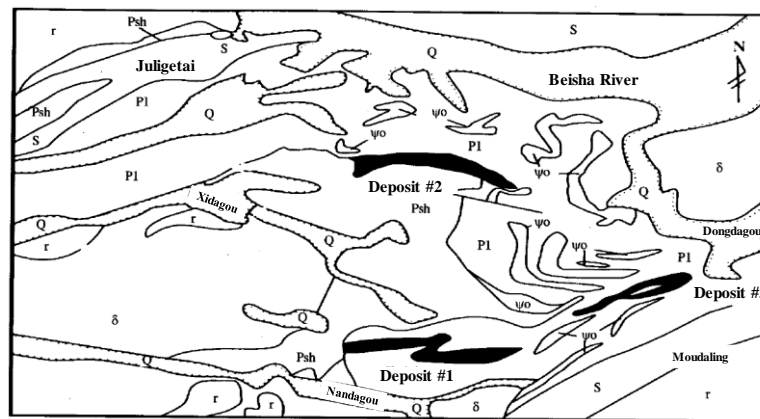
Psh-biotite quartz schist; P1-Chlorite schist; S-quartz sandstone; Psi-Gabbro; delta-Diorite; r-Granite; Q-Quaternary
