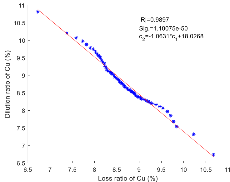
Figure 9. Linear fit of dilution ratio and loss ratio of Cu.
