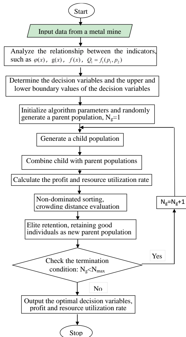
Figure 2. Flowchart of production process optimization of metal mines using the Non-Dominated Sorting Genetic Algorithm (NSGA-II).
