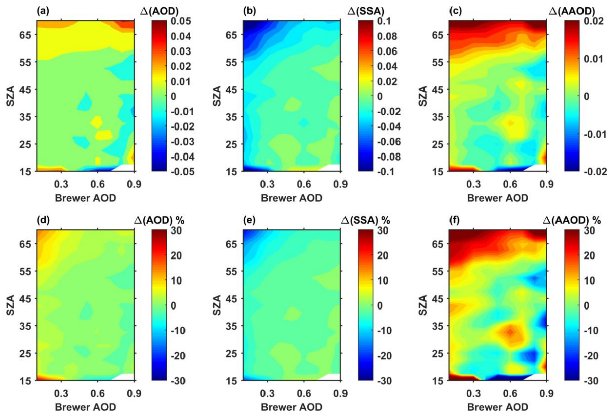
Figure 1. (a) absolute differences in AOD at 340 nm between Brewer#086 and CIMEL, (b) the corresponding differences in the calculated SSA and (c) the corresponding differences in the calculated AAOD. The same differences in % are presented in panels (d), (e), and (f) respectively.
