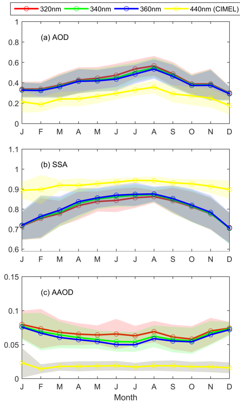
Figure 3. Long-term monthly averages of (a) AOD, (b) SSA, and (c) AAOD for the period 2003–2017. Data from Brewer#086 are shown for 320, 340, and 360 nm, and from CIMEL for 440 nm. The shaded areas represent the standard deviation envelope around the monthly averages.
