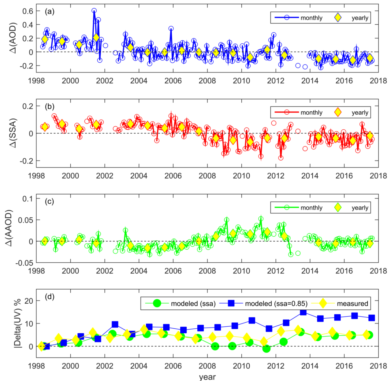
Figure 6. Monthly and annual mean anomalies for (a) AOD, (b) SSA, and (c) AAOD at 320 nm. Panel (d) depicts the difference of the annual average anomalies of the global UV irradiance at 320 nm relative to 1998 from the measurements (yellow), as well as from the simulations using the measured SSA (green) and a default SSA of 0.85 (blue).
