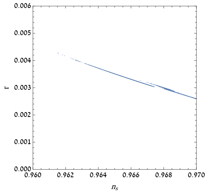
Figure 8. The relation between the scalar to tensor ratio r and the scalar spectral index n_s via sampled initial conditions with a normal distribution \Lambda_0 = 50 \pm 10 , M_1 = 20 \pm 10 . All of the sampled values fall well inside the Planck data constraint (67).
