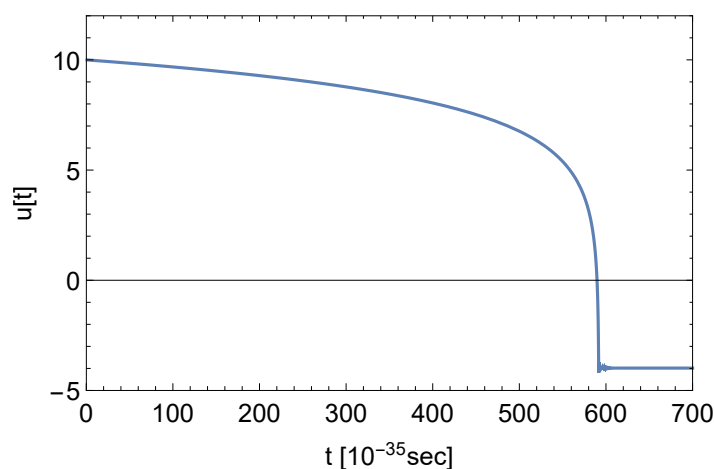
Figure 2. Numerical shape of the evolution of u(t) . The physical unit for u is M_{Pl}/\sqrt{2} .
