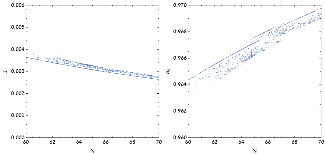
Figure 7. The scalar to tensor ratio r and the scalar spectral index n_s vs. the number of e -folds for different values of the initial conditions. The sampling of the latter is done with a normal distribution \Lambda_0 = 50 \pm 10 , M_1 = 20 \pm 10 .
