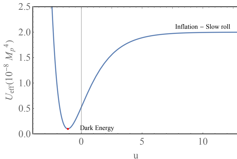
Figure 1. Shape of the effective potential U_{\text{eff}}(u) in the Einstein-frame (37). The physical unit for u is M_{\text{Pl}} / \sqrt{2} .
