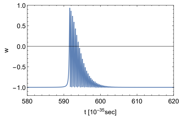
Figure 6. Evolution of w parameter of the equation of state with sharp growth above w \approx -1 for a short time interval after end of inflation – matter domination.
