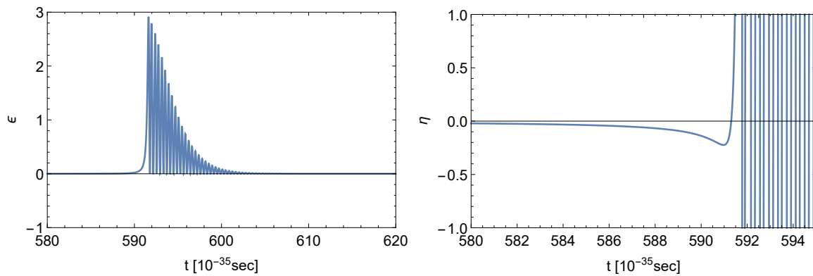
Figure 3. Slow-roll parameters \epsilon and \eta before and around end of inflation. When \epsilon = 1 the inflation ends.
