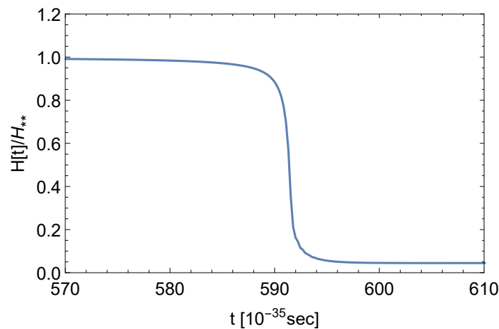
Figure 4. Numerical shape of the evolution of H(t) . Here H_{**} \equiv \sqrt{\Lambda_0/3} as in (58).
