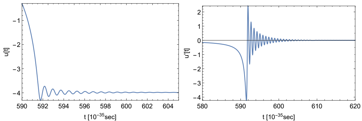
Figure 5. On the left panel – blown-up portion of the plot on Fig.2 around and after end of inflation depicting the oscillations of u(t) after end of inflation. On the right panel – oscillations of \dot{u}(t) after end of inflation.
