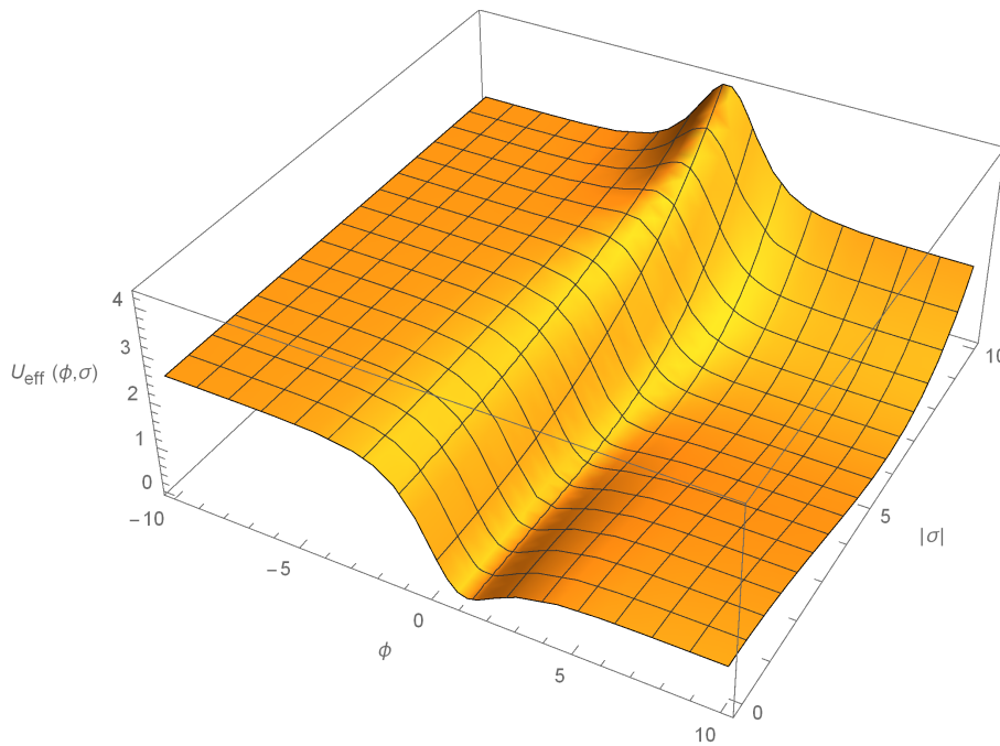
Figure 1. Qualitative shape of the two-dimensional plot for the effective scalar potential U_{\text{eff}}(\phi, \sigma) (26).
