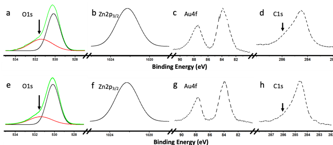
Figure 5. XPS spectra of Zn 2p 3/2 , O 1s, Au 4f and C 1s taken from as-grown Au@ZnO NWs-graphene (a - d), and Au@ZnO NPs-graphene (e - h).
