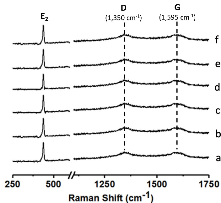
Figure 3. Raman spectra of 5%Au@commercial ZnO-graphene (a); 10%Au@commercial ZnO-graphene (b); 5%Au@ZnO NPs-graphene (c); 10%Au@ZnO NPs-graphene (d); 5%Au@ZnO NWs-graphene (e); and 10%Au@ZnO NWs-graphene (f).
