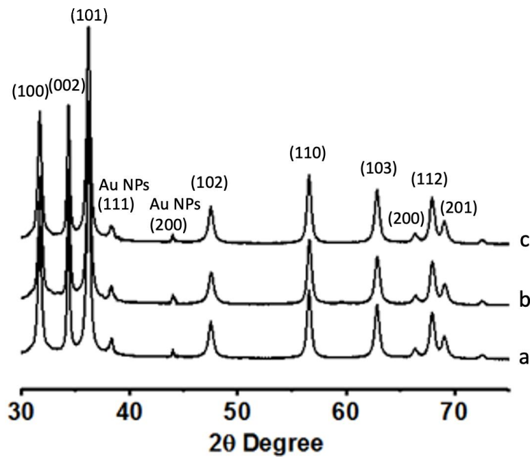
Figure 2. XRD diffraction patterns for 10% Au@commercial ZnO-graphene (a); 10%Au@ZnO NPs-graphene (b); and 10%Au@ZnO NWs-graphene (c).
