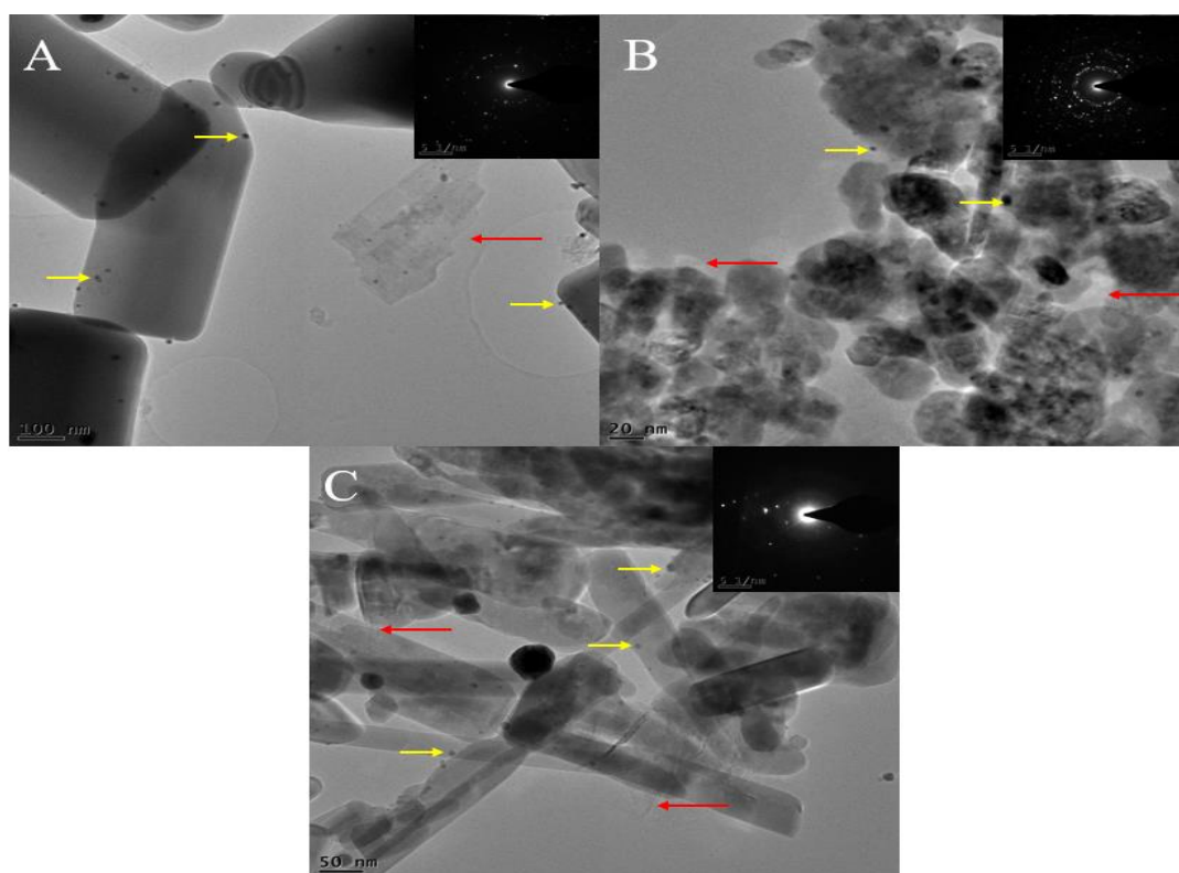
Figure 1. HRTEM images of 10%Au@commercial ZnO-graphene (A), 10%Au@ZnO NPs-graphene (B), and 10%Au@ZnO NWs-graphene (C). The red and yellow arrows indicate the presence of graphene and gold, respectively, and the insets correspond to the SAED patterns.
