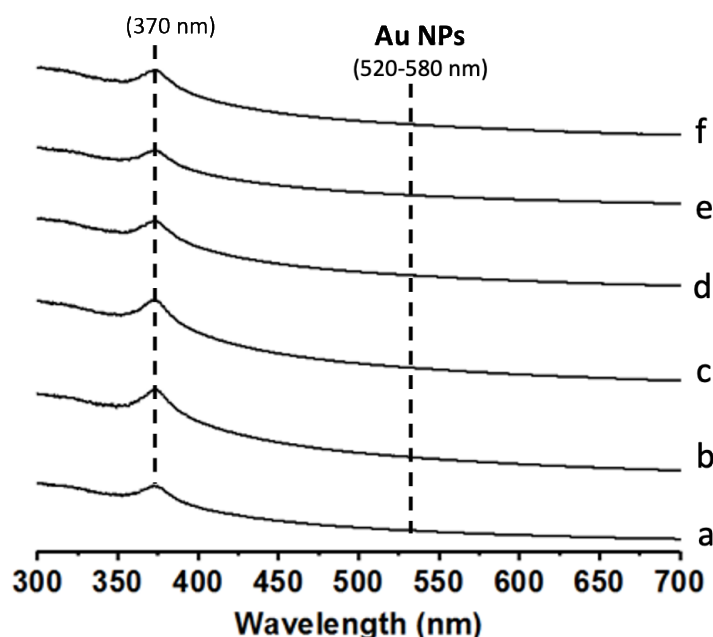
Figure 4. UV-vis spectra of different composites: 5%Au@commercial ZnO-graphene (a); 10%Au@commercial ZnO-graphene (b); 5%Au@ZnO NPs-graphene (c); 10%Au@ZnO NPs-graphene (d); 5%Au@ZnO NWs-graphene (e); and 10%Au@ZnO NWs-graphene (f).
