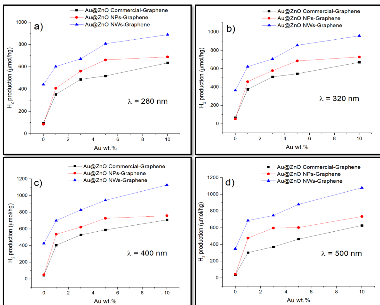
Figure 6. Photocatalytic hydrogen production of the different Au@ZnO-graphene catalysts under irradiation at 280 nm (a), 320 nm (b), 400 nm (c) and 500 nm (d).
