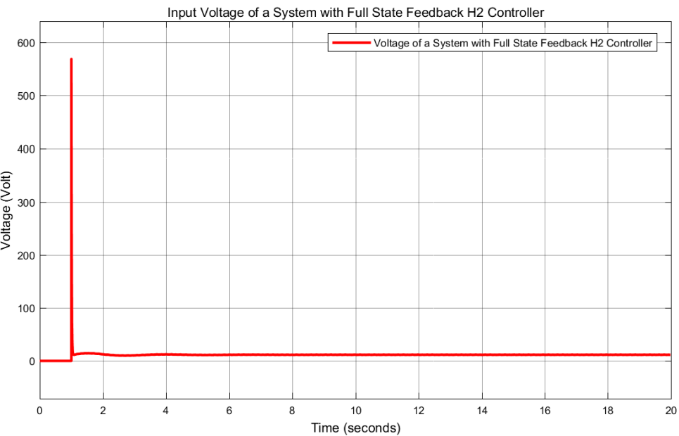
Figure 8 Input voltage to the system with full state feedback controller
