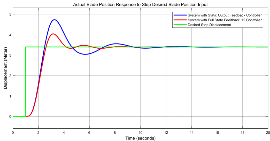
Figure 6 Step response of the comparison
