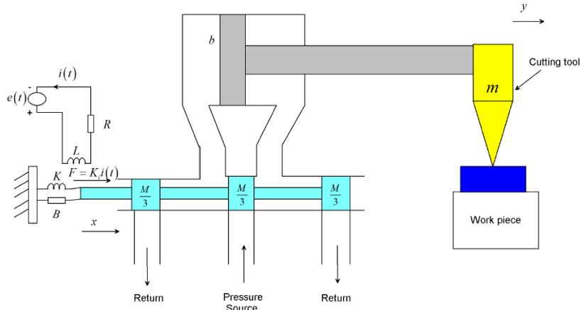
Figure 1 Metal Cutter Machine
