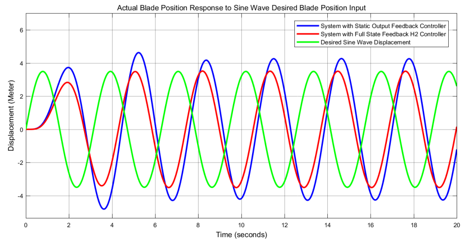
Figure 10 Sine wave response of the comparison
