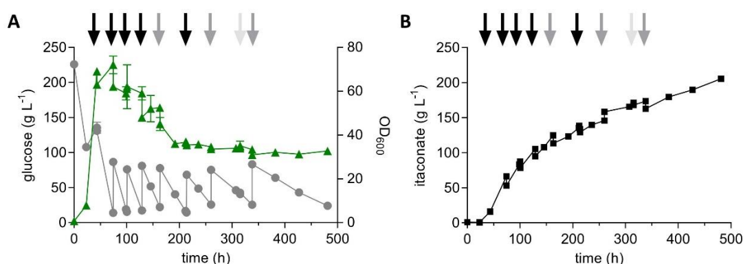
Figure 5. High-density pulsed fed-batch fermentation of U. maydis strain K14. (A) concentration of glucose (●) and OD 600 values (▲) and (B) concentration of itaconate (■) during fermentation in a bioreactor containing batch medium (200 g L -1 glucose, 4 g L -1 NH 4 Cl, CaCO 3 as buffering agent, 30 °C, 1000 rpm, top pitched blade impeller, bottom Rushton impeller). Arrows indicate the addition of 80 g glucose + 50 g CaCO 3 (black arrow), 80 g glucose (grey arrow), or 50 g CaCO 3 (light grey arrow). Error bars indicate the deviation from the mean (n = 2).
