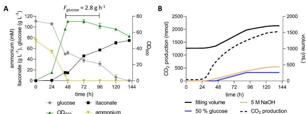
Figure 6. High-density fed-batch fermentation with continuous feed of U. maydis strain K14. (A) concentration of glucose, itaconate and ammonium, and OD 600 values and (B) filling volume, CO 2 production and the added volumes of 5 M NaOH and 50% glucose during fermentation in a bioreactor containing batch medium with 120 g L -1 glucose and 4 g L -1 NH 4 Cl. The pH was kept at 6.5 by automatic titration with NaOH. Cultures were fed with an additional 130 g glucose at a rate of 2.8 g h -1 during the indicated time interval. Error bars indicate the deviation from the mean (n = 2).
