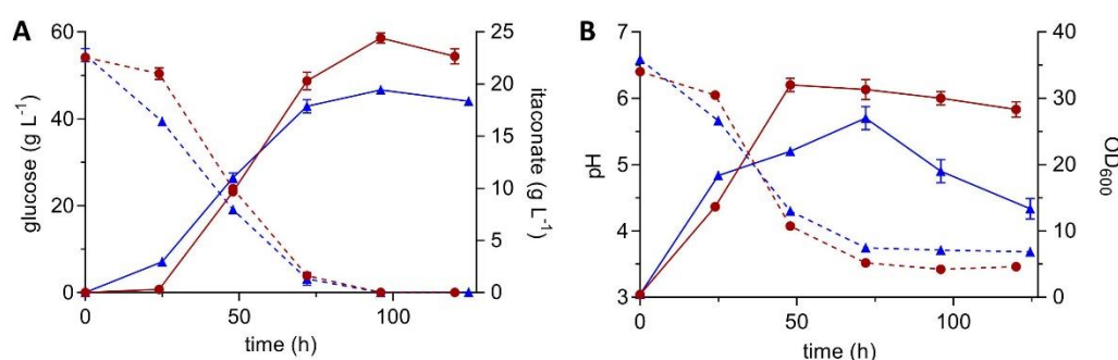
Figure 1. System Duetz® cultivation of morphology-engineered U. maydis MB215 strains in MTM with 50 g L -1 glucose and 100 mM MES, incubated in 24-well plates with a filling volume of 1.5 ml (shaking diameter = 50 mm, n = 300 rpm, T = 30 °C and Φ = 80%). (A) Concentrations of itaconate (continuous lines) and glucose (dotted lines), (B) OD 600 (continuous lines) and pH (dotted lines) of U. maydis MB215 \Delta cyp3 \Delta MEL \Delta UA \Delta dgat \Delta P_{ria1::P_{etef}} (▲) and the same strain with additional fuz7 deletion (●). Error bars indicate the standard error of the mean (n = 3).
