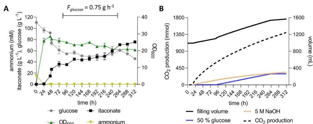
Figure 7. Low-density fed-batch fermentation with continuous feed of U. maydis strain K14. (A) concentration of glucose, itaconate and ammonium, and OD 600 values and (B) filling volume, CO 2 production and the added volumes of 5 M NaOH and 50% glucose during fermentation in a bioreactor containing batch medium with 120 g L -1 glucose, 0.8 g L -1 NH 4 Cl. The pH was kept at 6.5 by automatic titration with NaOH. Cultures were fed with an additional 130 g glucose at a rate of 0.75 g h -1 during the indicated time interval. Error bars indicate the deviation from the mean (n = 2).
