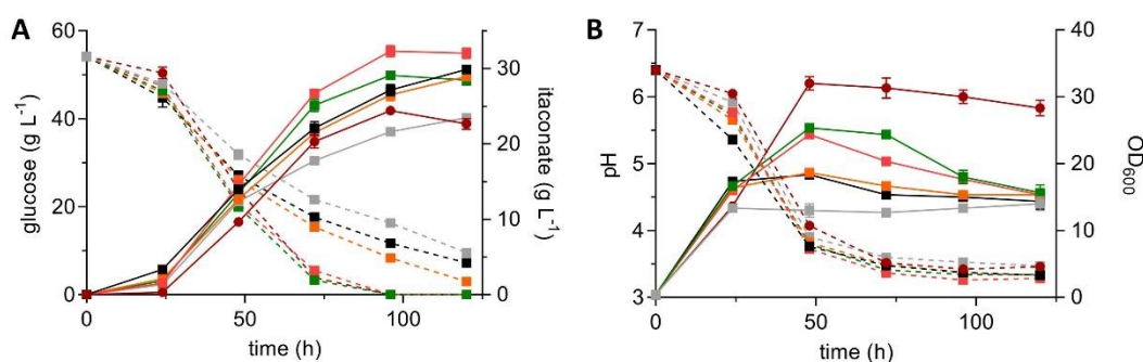
Figure 2. System Duetz® cultivation of U. maydis MB215 strains expressing mttA in MTM with 50 g L -1 glucose and 100 mM MES, incubated in 24-well plates with a filling volume of 1.5 ml (shaking diameter = 50 mm, n = 300 rpm, T = 30 °C and Φ = 80%). Itaconate production (continuous lines) and glucose consumption (dotted lines) (A) are shown, as well as OD 600 (continuous lines) and pH (dotted lines) (B) of U. maydis MB215 \Delta cyp3 \Delta MEL \Delta UA \Delta dgat \Delta P_{ria1::P_{etef}} \Delta fuz7 (red) and five P_{etef}mttA transformants named K3 (grey), K8 (green), K9 (orange), K10 (pink), and K14 (black). Error bars indicate the standard error of the mean (n = 3).
