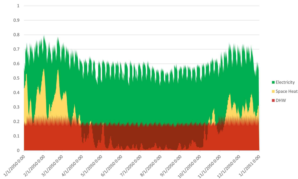
Figure 6. Normalized demand profiles of SH in 2050
