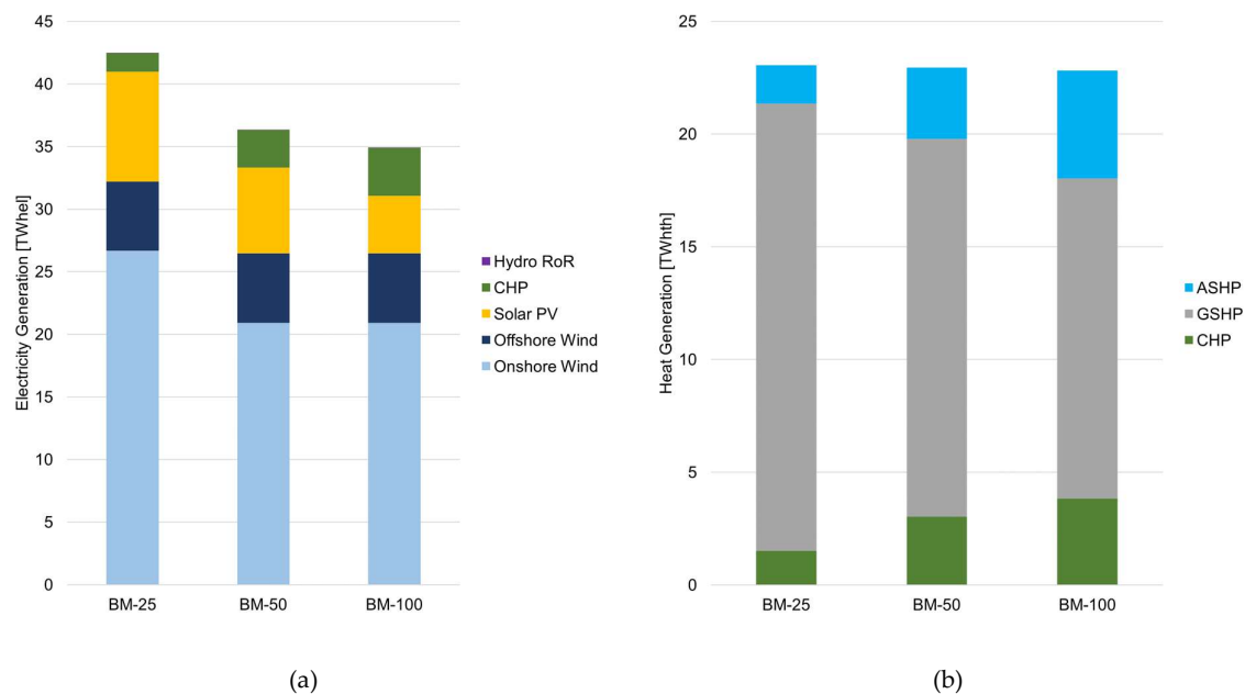
Figure 12. Energy mix for different scenarios in SH (a) electricity mix (b) heat mix
