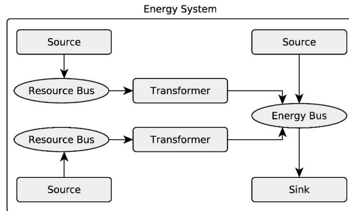
Figure 1. Schematic illustration of an energy system represented as an oemof network. Source: [16].
