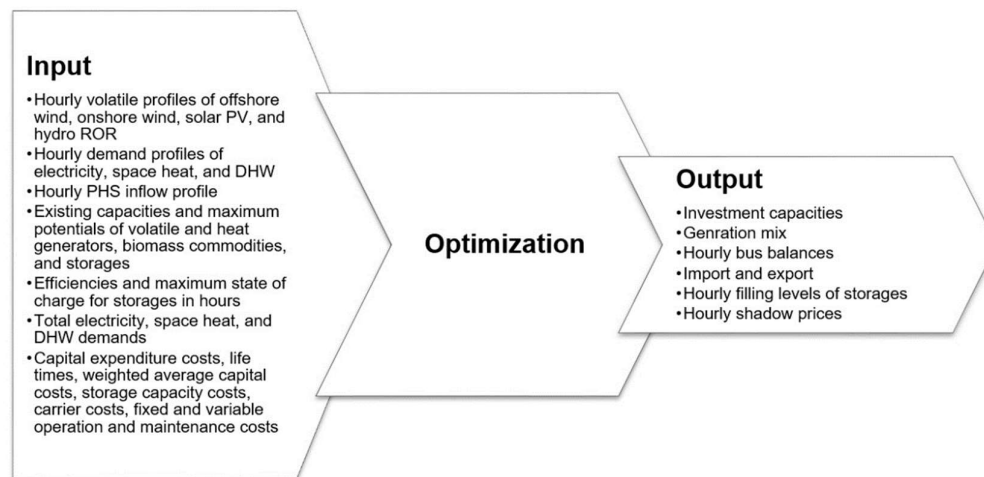
Figure 4. OSeEM-SN Input and Output
