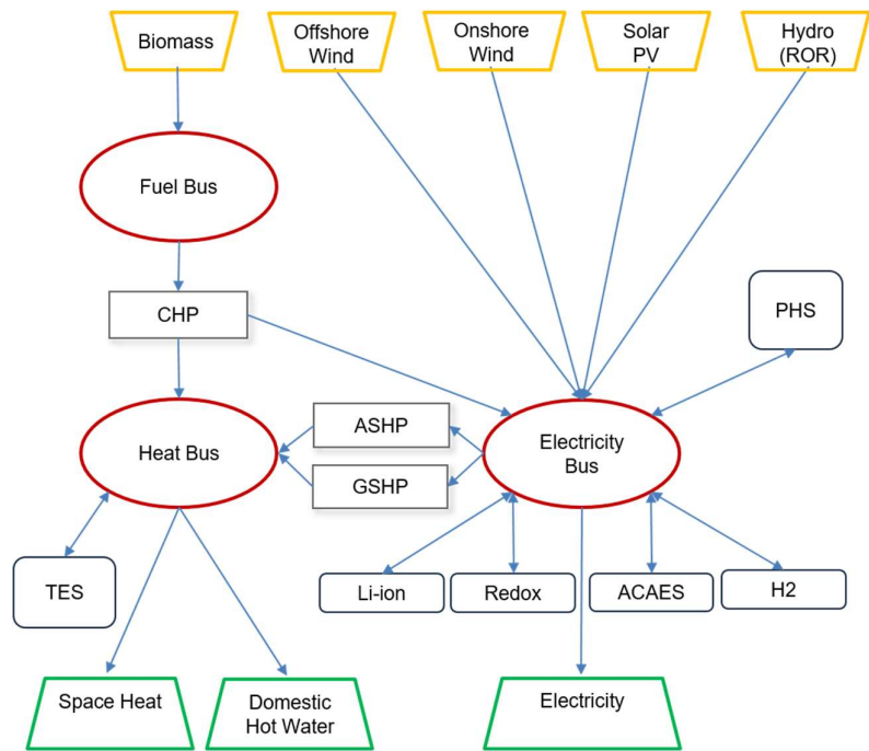
Figure 3. Simplified block diagram of the OSeEM-SN model
