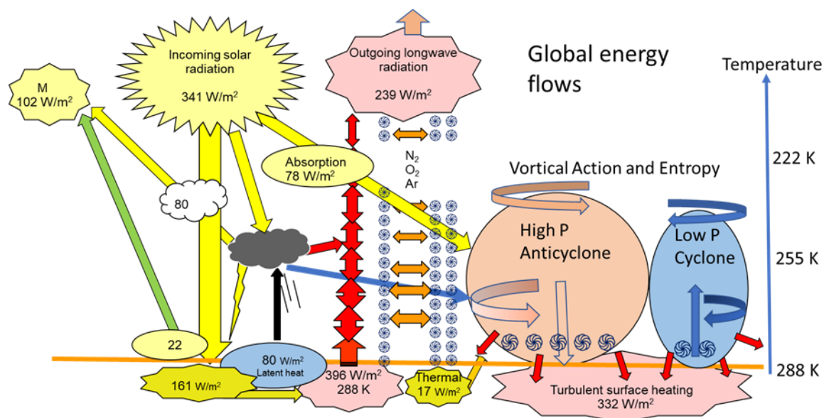
Figure 6. Coupling of Earth's heat budget [18] to vortical friction in anticyclones and cyclones. The downwelling radiation is regarded as a product of turbulent surface heating from friction. This is consistent with declining wind speed closer to the surface.
