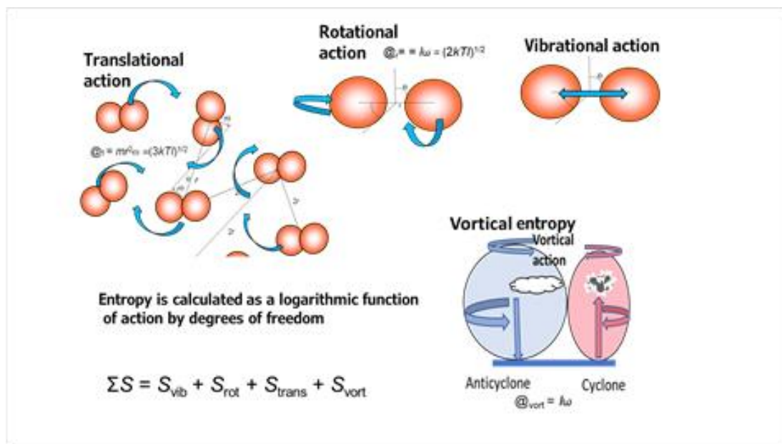
Figure 5. By analogy with translational, rotational and vibrational relative action and entropy of N_2 (see equations (6), (7) and (9) respectively) shown here we introduce vortical relative action in rotating air masses of anticyclones and cyclones, further increasing the action and entropy of masses of air and its heat capacity ST . Vortical action is modelled here simply as 1-dimensional, but it would also contain a smaller fraction of second dimensional action but no third locally.
