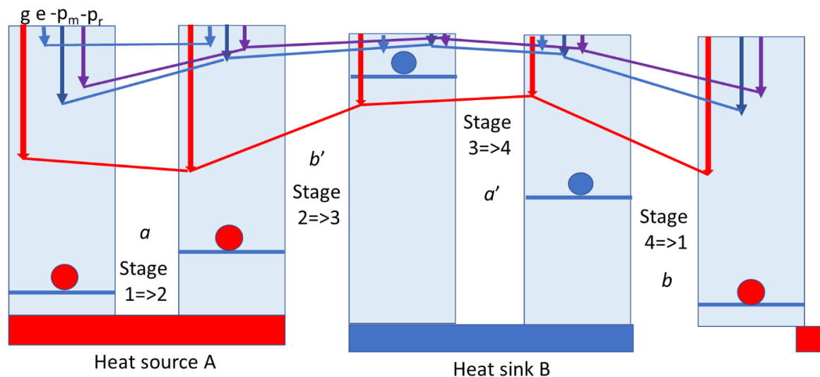
Figure 4. Carnot cycle for argon showing changes in mean molecular energy ( e ), Gibbs potential ( g ), pressure ( p_m ) and quantum field intensity ( p_g ). While the energy is stationary in stages 1=>2 and 3=>4 the Gibbs potential varies ( a=>b'=>a'=>b in Carnot's model) and the maximum work possible is thus equal to (a-a') = (b-b') .
