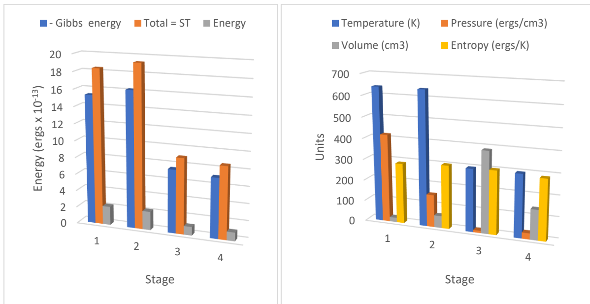
Figure 3. Action revision Carnot cycle for nitrogen showing thermodynamic energy in each stage; action is initiated in stage 1 at 40 atmospheres pressure and 640 K source temperature, declining to 298 K in stage 2. All values for negative Gibbs energy ( -g ), entropic energy ( sT ) and internal energy ( e ) are \times 10^{-13} ergs per molecule. Heat Q_f of kT is added from the heat source in the isothermal transition stage 1 \Rightarrow 2 shown in the increased values of sT and -g and heat Q_r is removed to the sink in the isothermal stage 3 \Rightarrow 4 , showing markedly decreased value of sT , and -g . The value of the entropy per molecule is \times 10^{-17} ergs/K, for temperature degrees Kelvin, pressure in Pascals and volume per molecule \times 10^{-22} cm 3 . Pressure, volume and temperature conform to pa^3 = kT . The small increase in entropy in stage 1 \Rightarrow 2 of k \ln(V_2/V_1) is equal to the decline in entropy in stage 3 \Rightarrow 4 , k \ln(V_3/V_4) .
