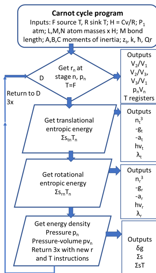
Figure 1. Carnot cycle flow sheet to estimate thermodynamic outputs
