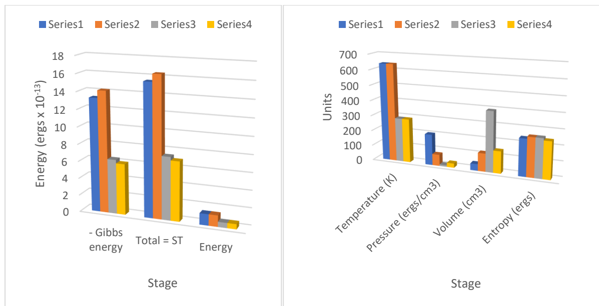
Figure 2. Action revision Carnot cycle for argon showing thermodynamic energy in each stage commencing at 20 atmospheres pressure and 640 K temperature, with kT equal to Q_f initiating changes in action. All values for negative Gibbs energy ( -g_i ), entropic energy ( sT ) and internal energy ( e ) are \times 10^{-13} ergs per molecule. Heat Q_f is added from the heat source in the isothermal transition stage 1 \Rightarrow 2 shown in the increased values of sT and -g and heat Q_r is removed to the sink in the isothermal stage 3 \Rightarrow 4, showing markedly decreased value of sT , and -g . The value of the entropy per molecule is \times 10^{-17} ergs/K, for temperature degrees Kelvin, pressure in Pascals and volume per molecule \times 10^{-22} cm 3 . Pressure, volume and temperature conform to \text{pa}^3 = kT . The small increase in entropy in stage 1 \Rightarrow 2 of k \ln(V_2/V_1) is equal to the decline in entropy in stage 3 \Rightarrow 4, k \ln(V_3/V_4) .
