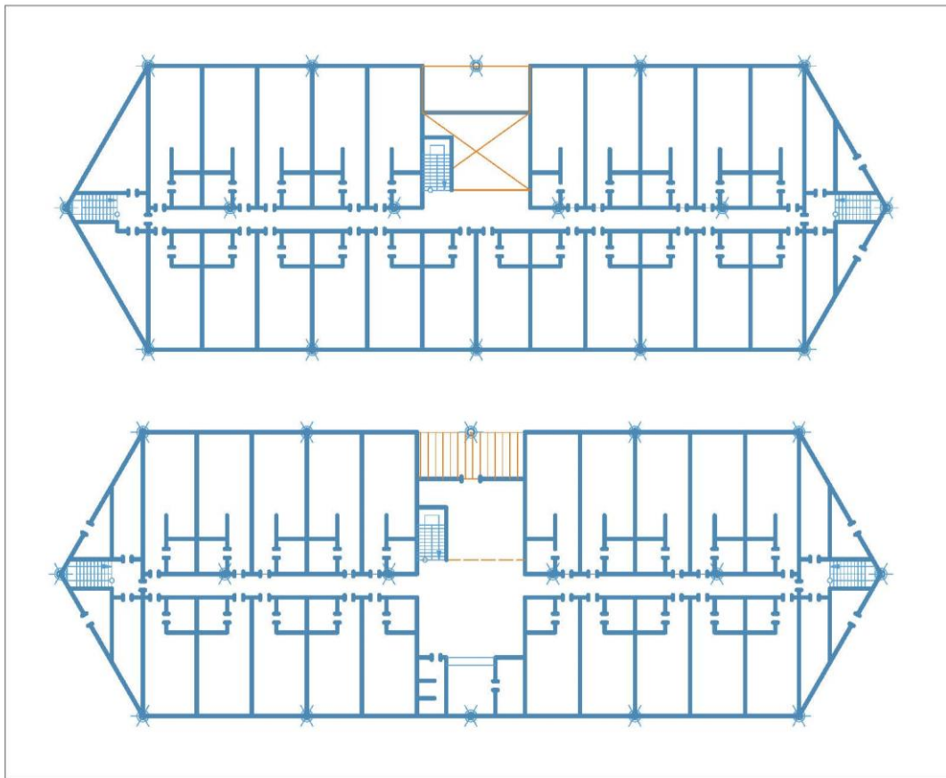
Fig. 12. Planning solutions: the Ordinary Motel (24 rooms) – 1 st , 2 nd floors.
