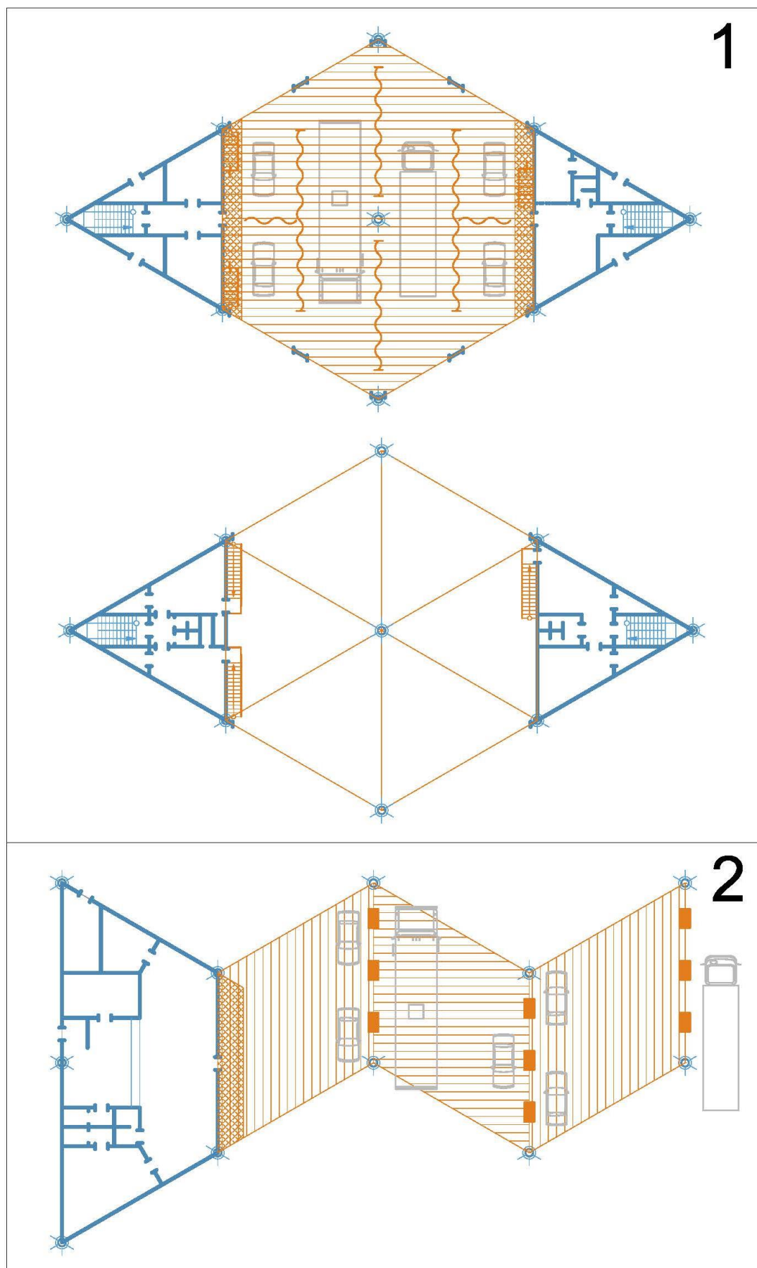
Fig. 8. Planning solutions: 1 – the Car wash (6 posts) - 1 st , 2 nd floors; 2 – the Car refueling (petrol-diesel).
