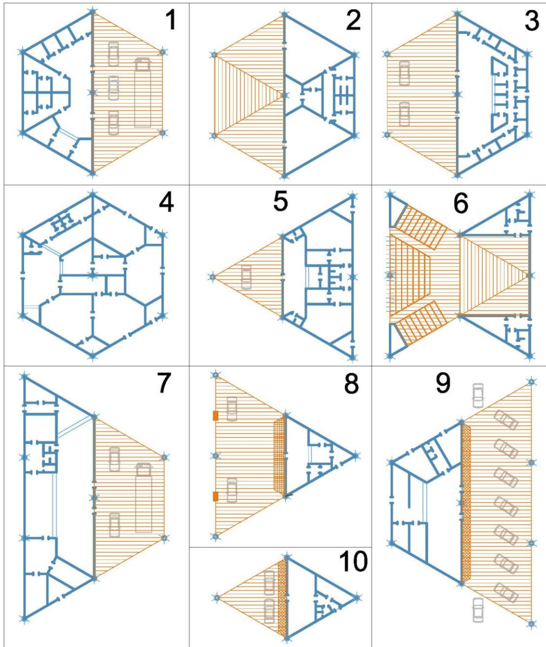
Fig. 6. Planning solutions: 1 – the Heating point; 2 – the Children's play area; 3 – the Post office; 4 – the Laundry; 5 – the First aid post; 6 – the Auditorium; 7 – the Retail and catering point; 8 – the Car refueling (gas); 9 – the Car refueling (electric); 10 – the Retail point.
