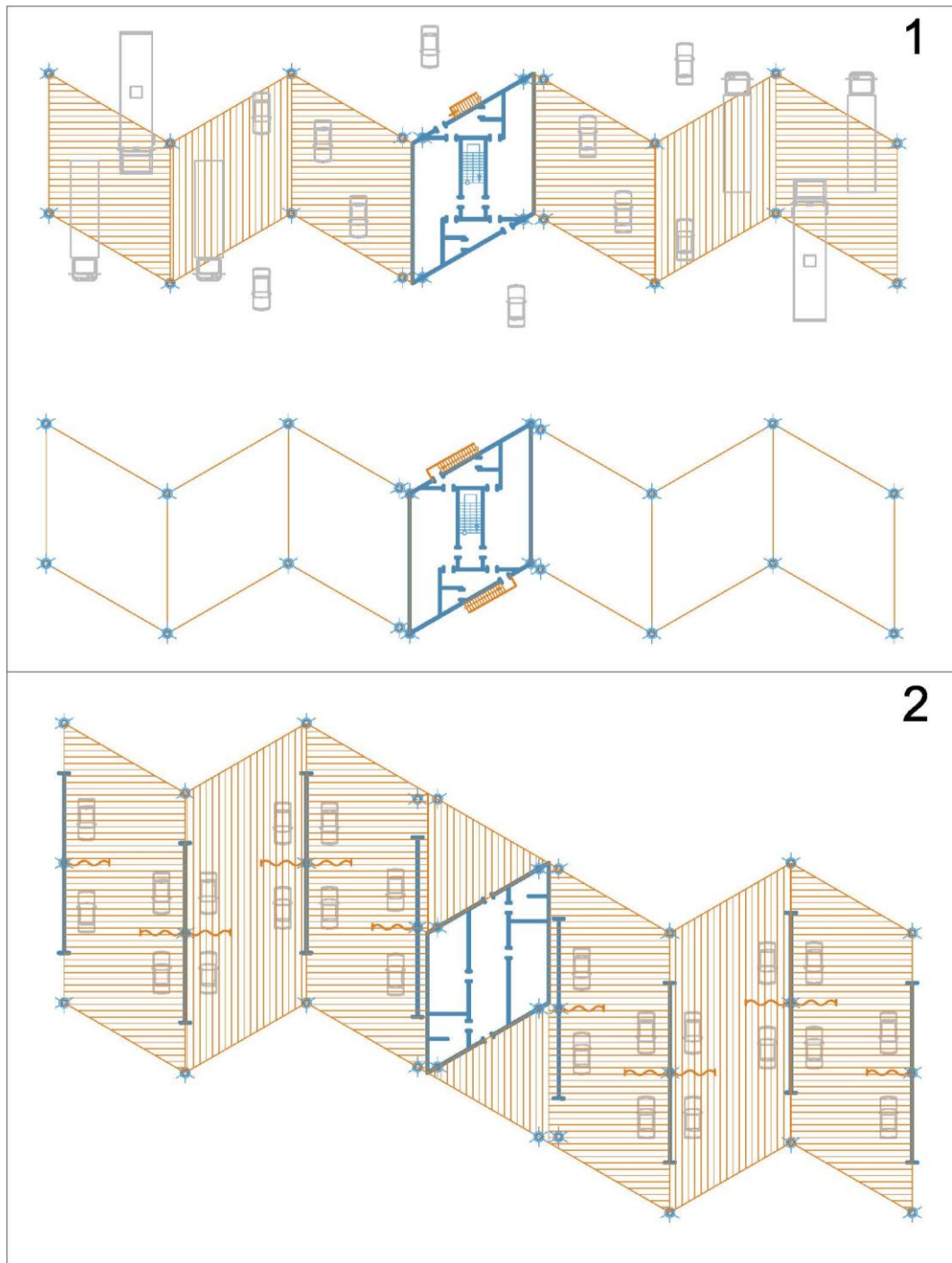
Fig. 9. Planning solutions: 1 – the Checkpoint (6+6 posts) - 1 st , 2 nd floors; 2 – the Self-service car wash (24 posts).
