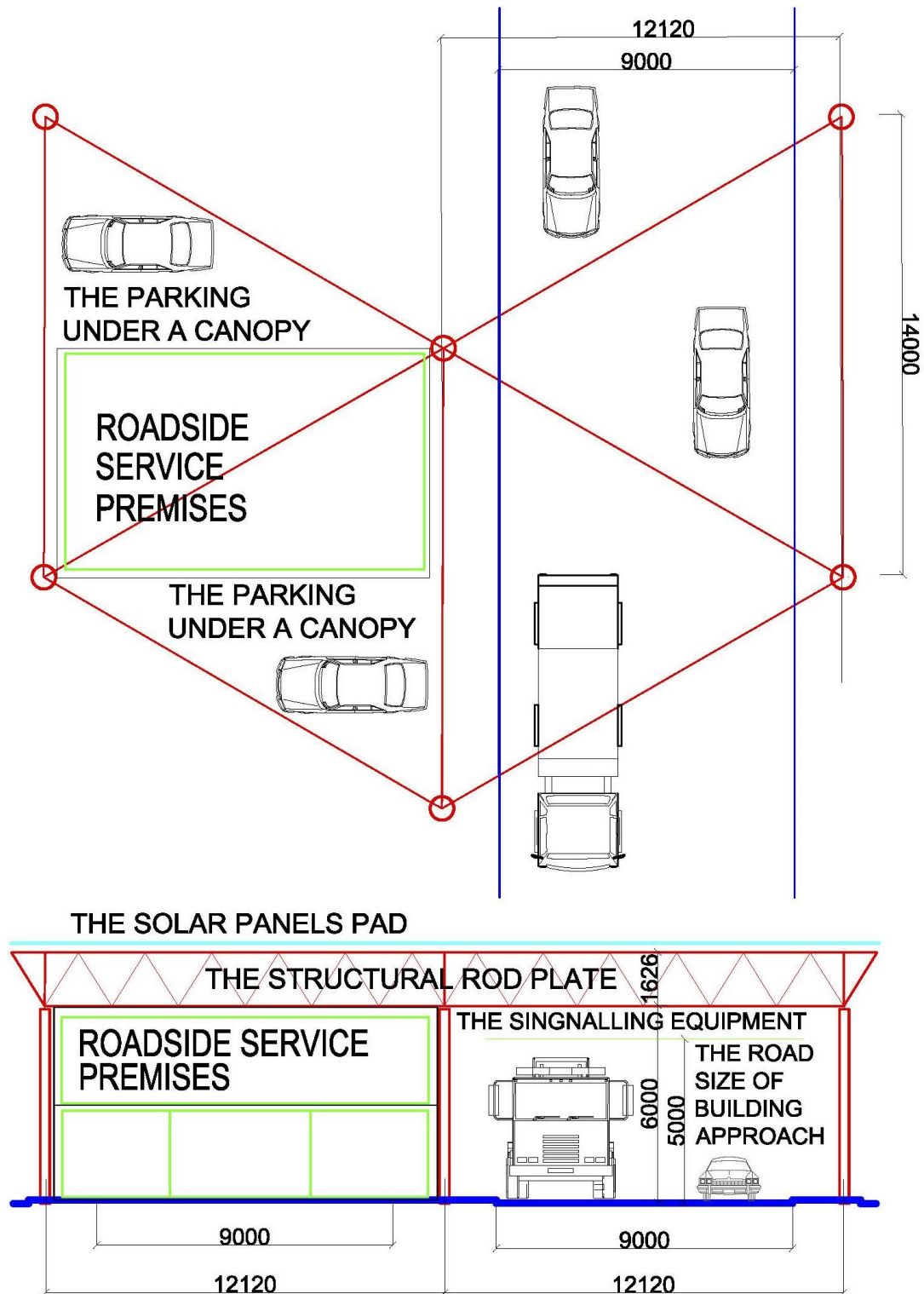
Fig. 2. Module parameters: a plan, a section.
