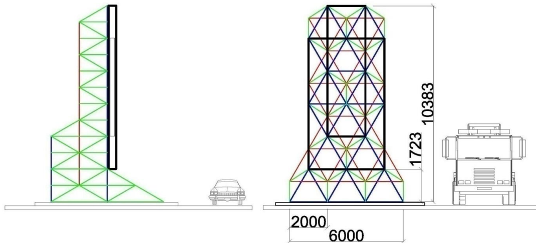
Fig. 16. The Diagram (side view, front view) of the rod structure as a support for the information board.
