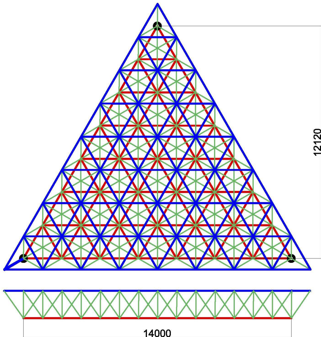
Fig. 1. The scheme of the modular structural plate: a plan, a section.
