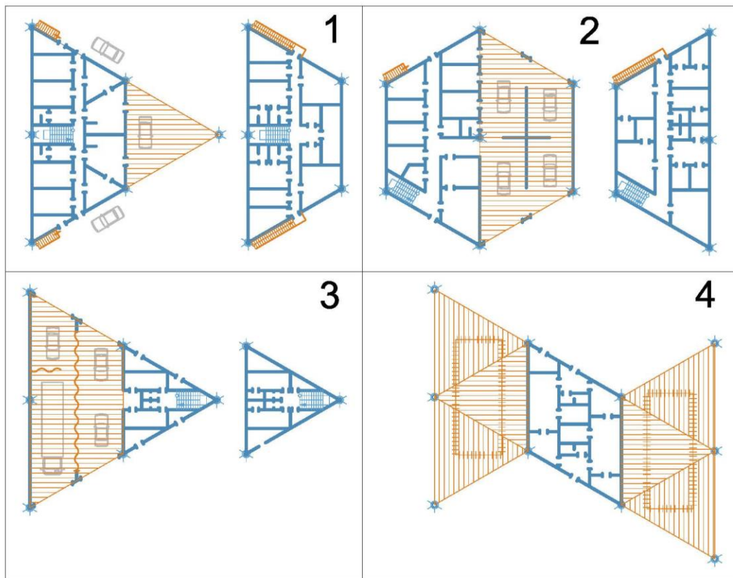
Fig. 5. Planning solutions: 1 – the Point of medical and rescue service - 1 st , 2 nd floors; 2 – the Car Service station - 1 st , 2 nd floors; 3 – the Car wash (4 posts) - 1 st , 2 nd floors; 4 – the Point of weight and dimensional control.
