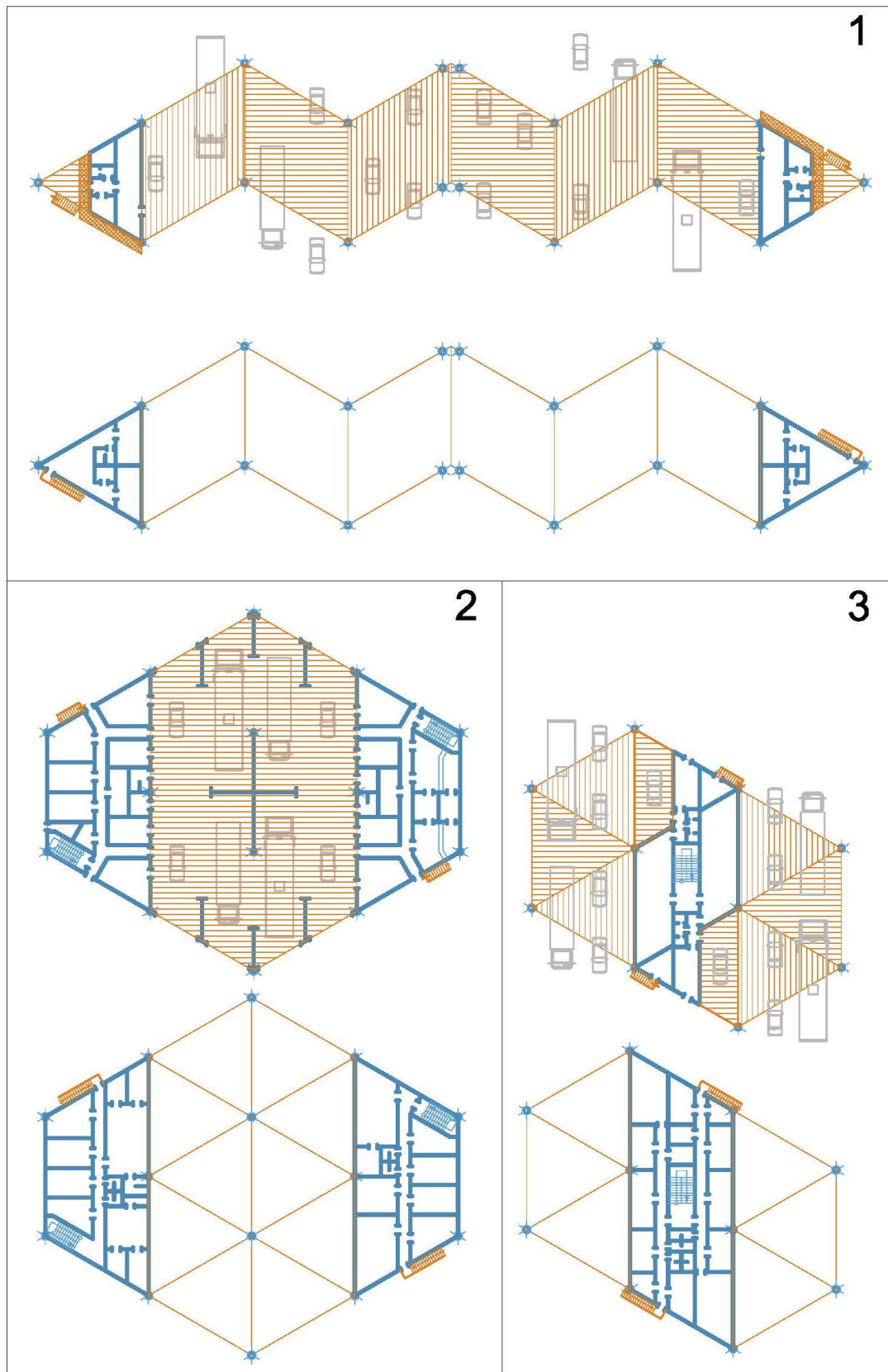
Fig. 7. Planning solutions: 1 – the Checkpoint (6+6 posts) - 1 st , 2 nd floors; 2 – the Service station (8 posts) - 1 st , 2 nd floors; 3 – the Traffic control point - 1 st , 2 nd floors.
