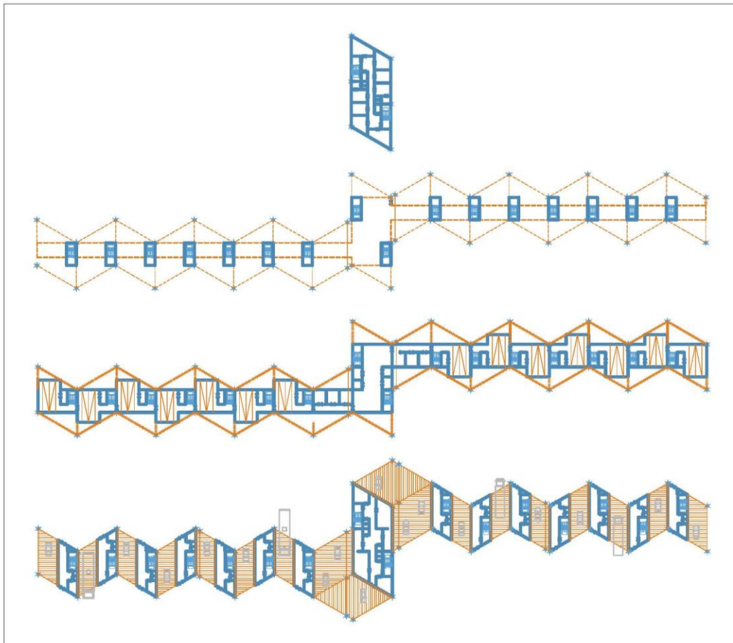
Fig. 13. Planning solutions: the Special vehicle control point (levels 1, 2, 3, 4).
