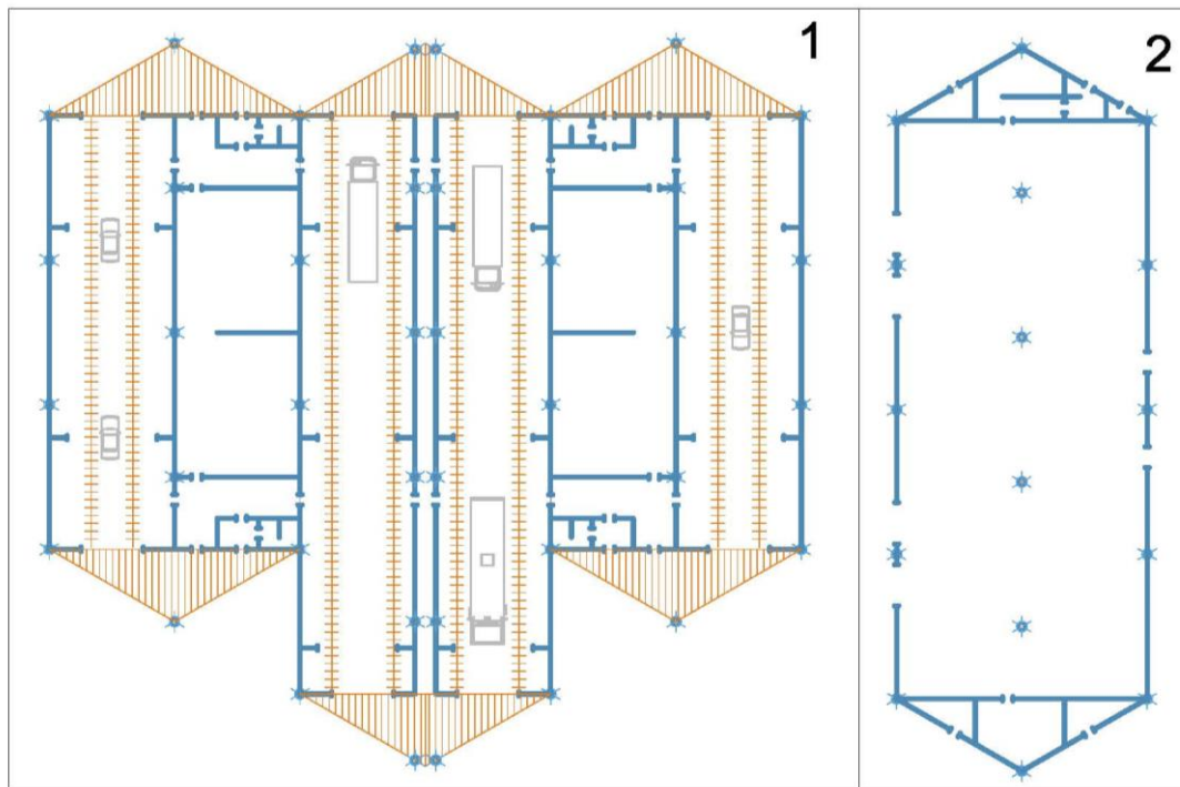
Fig. 10. Planning solutions: 1 – the Contactless car wash (4 posts); 2 – the Warehouse.
