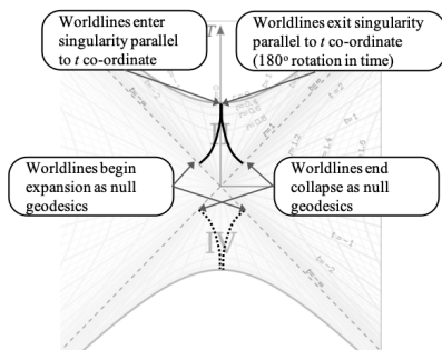
FIG. 9. Example Internal Worldline
