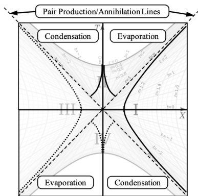
FIG. 10. Full Symmetry of the Schwarzschild Metric
