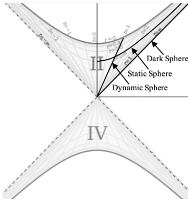
FIG. 1. Celestial Sphere Types on Kruskal-Szekeres Coordinate Chart
