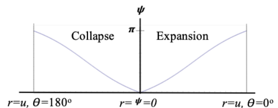
FIG. 12. Local light cone angles over time
