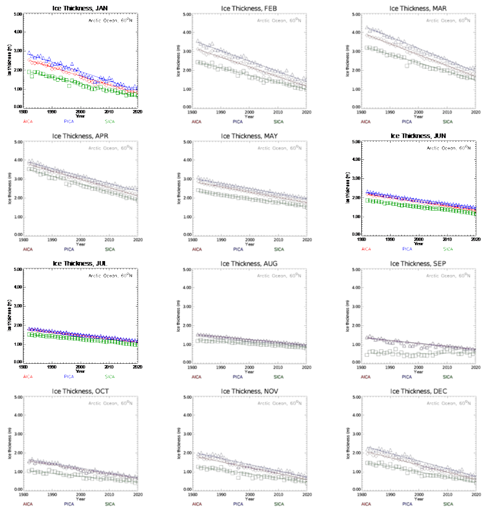
Figure 10. SIT time series for the Arctic area north of 60°N over 1982–2020 for the months of January through December. PICA (blue) stands for perennial ice-covered area, SICA (green) denotes seasonal ice-covered area, and AICA (red) designates all ice (PICA + SICA) covered areas.
