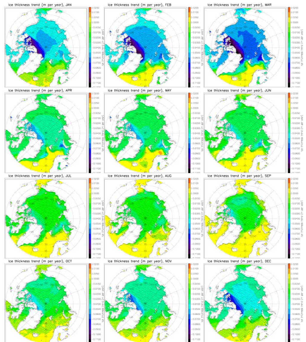
Figure 9. Spatial distributions of Arctic monthly mean SIT trends over 1982-2020 for the months of January through December over 1982-2020.
