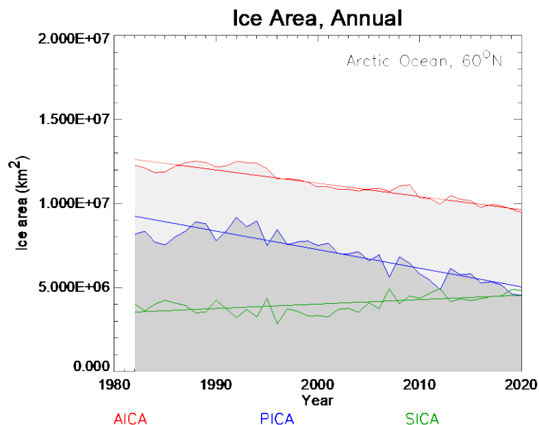
Figure 2. Time series of Arctic seasonal, perennial, and all ice-covered areas on the yearly basis within the Arctic area north of 60°N degree. SICA (green) stands for seasonal ice-covered area, PICA (blue) denotes perennial ice-covered area, and AICA (red) is the sum of SICA and PICA.
