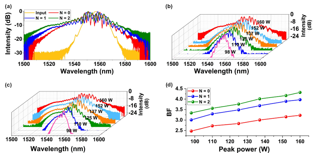
Figure 4. SPM experimental results. (a) Normalized spectra of optical pulses before and after propagation through the GO-coated SOI nanowires with 1 and 2 layers of GO at an input peak power of ~160 W. (b) – (c) Optical spectra measured at different input peak powers for the hybrid waveguides with 1 and 2 layers of GO, respectively. (d) BF of the measured output spectra versus input peak power for the hybrid waveguides with 1 and 2 layers of GO. In (a) – (d), the corresponding results for the uncoated SOI nanowires ( N = 0 ) are also shown for comparison.
