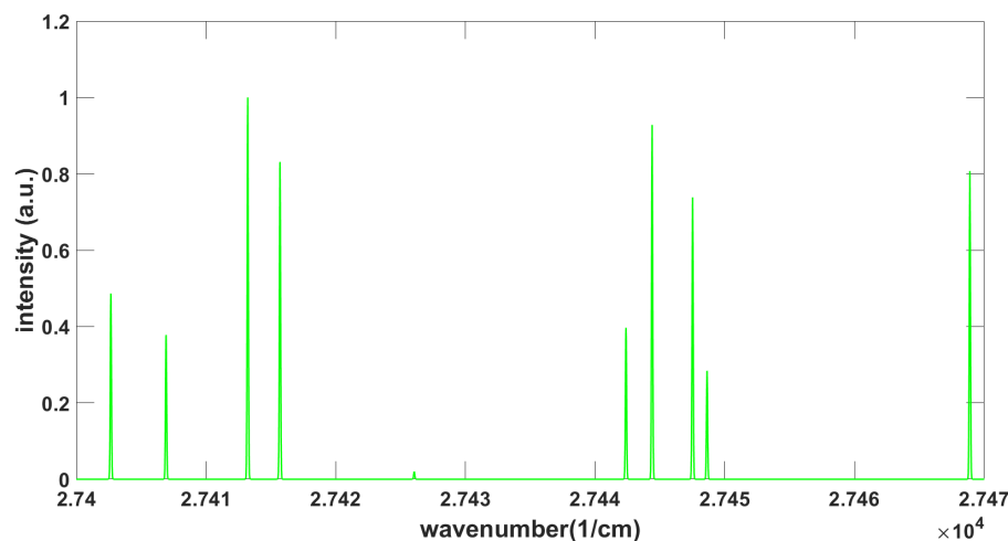
Figure 7. Computed CH B-X emission spectrum, \delta\tilde{\nu} = 0.1 \text{ cm}^{-1} , T = 1.5 \text{ kK} .
