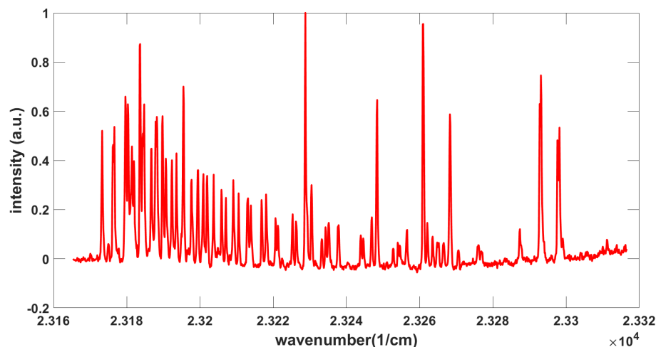
Figure 4. Originally recorded CH A-X spectrum using CRDS.
