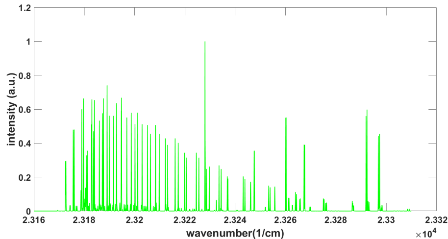
Figure 5. Computed CH A-X emission spectrum, \delta\tilde{\nu} = 0.1\text{ cm}^{-1} , T = 1.5\text{ kK} .
