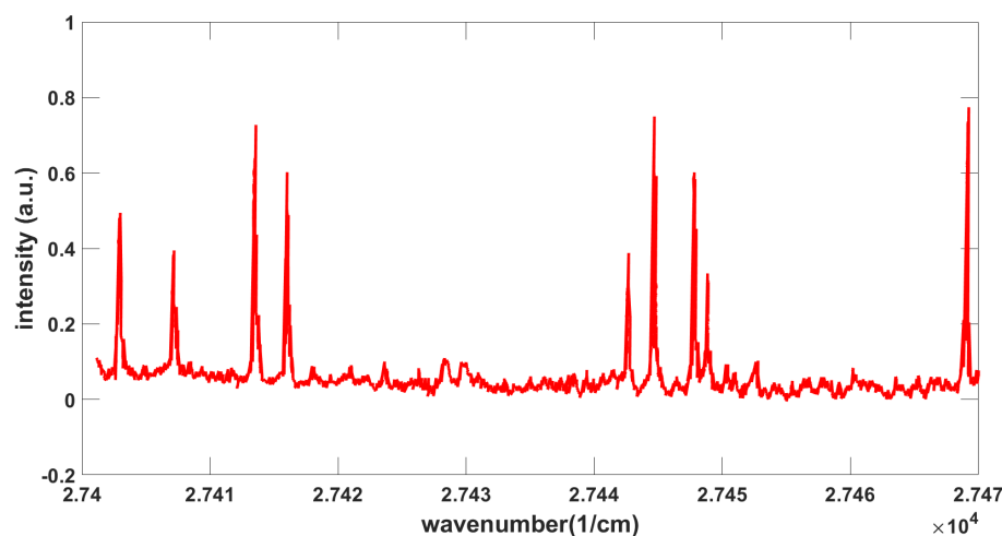
Figure 6. Originally recorded CH B-X spectrum using CRDS.
