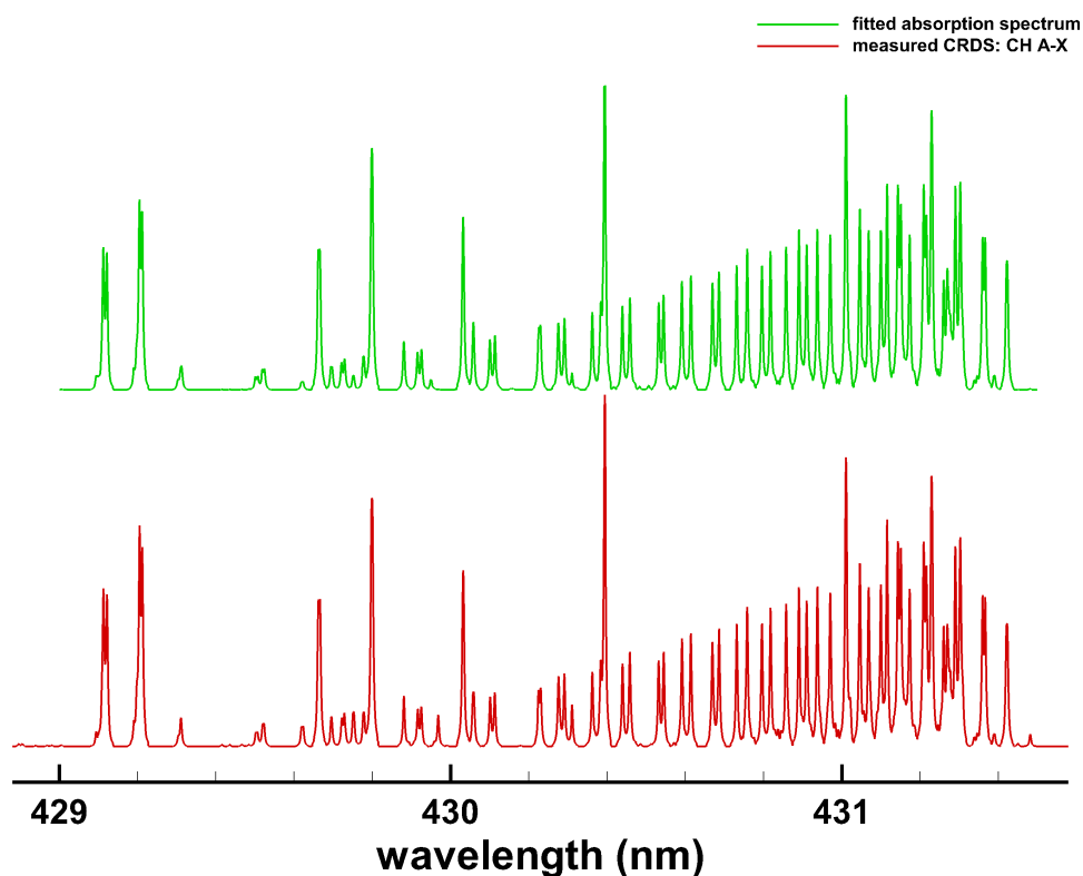
Figure 3. Comparison of measured and fitted CH A-X spectra, \delta\lambda = 0.005 nm, T = 1.47 kK.
