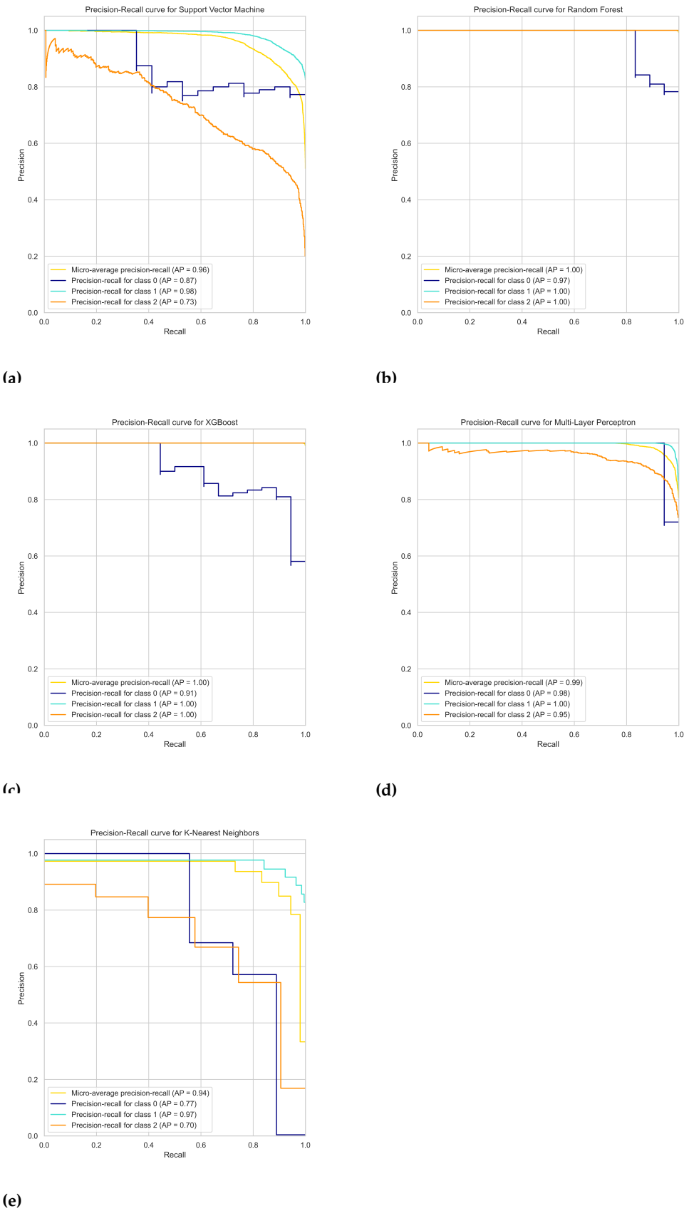
(e) Figure 2. Precision-Recall Curves for the models.
