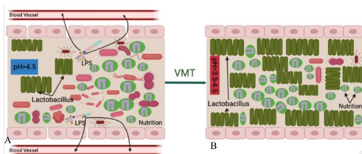
Figure 4. Potential mechanism of VMT; increased competition for nutrition(A: before VMT; B: after VMT). (Created with BioRender.com).
