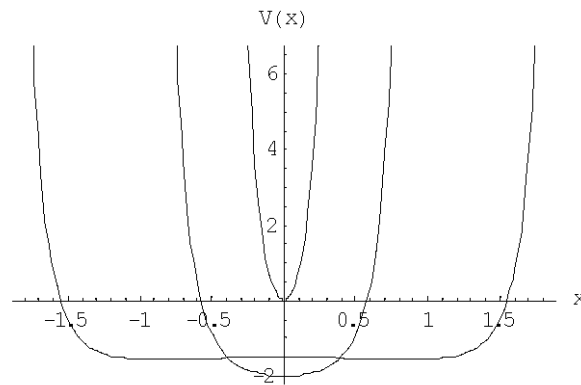
Figure 4. The potential energy of the muon's center of mass as a function of spacing between the poles. The stable ground state of the muon occurs at maximum binding energy ( V(x) = -2 ; d' = 1 ). The binding energy is lost for spacing d' = 0.5 .
