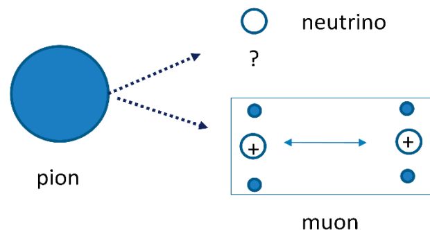
Figure 2. The decay of the pion's atypical dual dipole moment configuration into two typical single dipole moment configurations.
