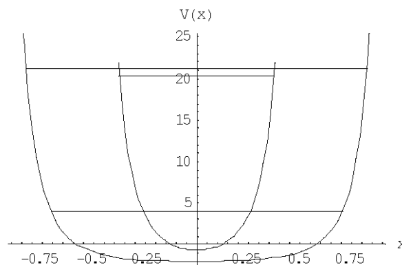
Figure 5. The jump from the muon state to the tauon state is a jump from the first excitation level of the muon state to the ground state of the heavier tauon. It happens at a spacing d' = 0.54 , where the energy constants (not to be confused with the massive energies) match, under preservation of a slight amount of binding energy.
