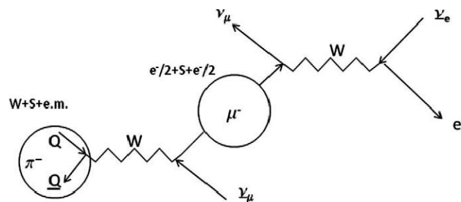
Figure 3. A charged pion decays into a charged lepton (muon) and its associated neutrino because of emission of the vector weakinteraction boson. Subsequently, the muon and the neutrino recoils into a weak interaction boson that subsequently decays into a (Pauli) shower of electrons and antineutrinos.
