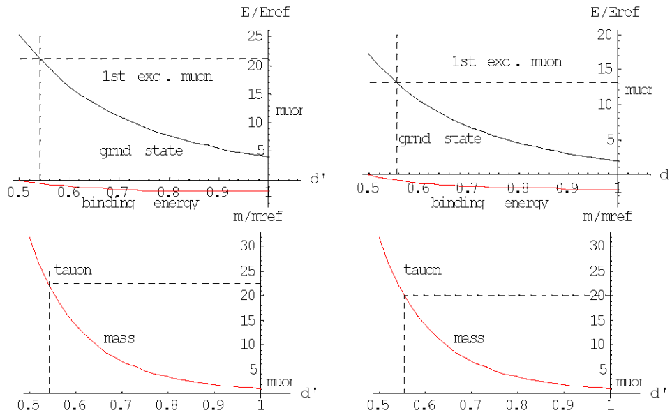
Figure 6. The lower curves show the dependence of the lepton's physical mass on the pole spacing. The upper graphs show that the pole spacing of the tau particle is determined by the equality in vibration energy of the muon's first excitation level and the ground state vibration energy of the heavier tau particle. Note that the binding energy of the tau particle is just slightly negative. The right-hand figures are a first-order correction on the left-hand part ones.
