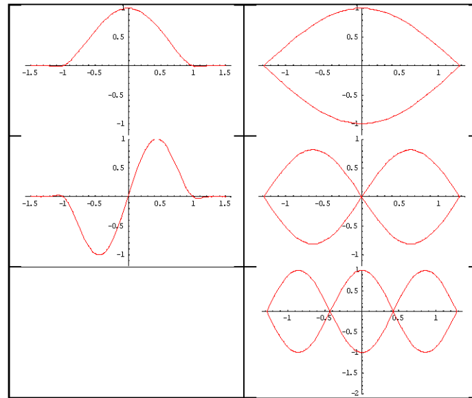
Figure 10. Comparison of the wave function formats between the charged lepton and the neutrinos. Whereas the wave function of the charged lepton is close to the one of an harmonic quantum mechanical oscillator, the wave function of a neutrino is a non-electromagnetic standing wave packet. .
