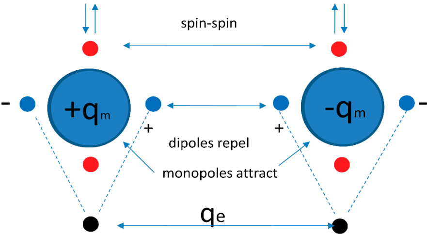
Figure 1. Hypothetical equivalence of the quark’s polarisable linear dipole moment with the magnetic dipole moment of its electric charge attribute.
