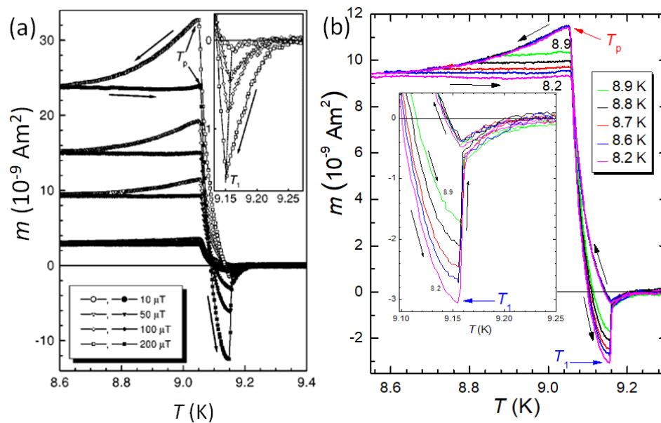
Figure 5. Details of m(T) transitions measured on a punched Nb disk. Measurements performed at Detroit. (a). Superconducting transitions measured in small applied magnetic fields (10, 50, 100, 200 \mu\text{T} ) generated by the Cu coil (low-field option). The arrows indicate the direction of the measurement (FC-C and FC-W). The temperature T_p is defined here as the temperature of the maximum m . The inset shows the definition of the temperature T_1 as the lowest m recorded on the diamagnetic side. Figure reprinted with permission from Ref. [114]. (b). FC-C and FC-W curves recorded to various lowest temperatures as indicated in the graph, ranging between 8.2 K and 8.9 K. The characteristic temperatures T_p and T_1 are indicated by red and blue arrows, respectively. The inset gives the details around T_1 .
