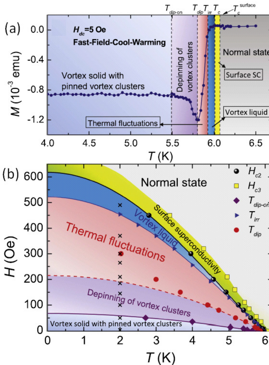
Figure 23. (a). Temperature dependence of the magnetization in the FFCW mode at 0.5 mT (5 Oe). (b). Phase diagram for the PME in FFCW mode. The third critical field H_{c3} is defined from the onset of DPE in the in-phase ac susceptibility measurements; H_{c2} is defined from the intersection of two linear fits of the M(T) curves above and below the onset; T_{irr} is derived as the onset of a diamagnetic signal on the in-phase ac susceptibility curve. The solid and dashed lines are plots of the empirical formula H(T) = H_0[1 - (T/T_c)^2]^n . The crosses show the field locations where the magnetic relaxation curves are measured. Image reproduced with permission from Ref. [37].
