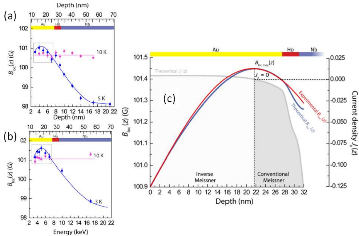
Figure 21. Average local magnetic field in Au/Ho/Nb trilayers as a function of the muon implantation energy and mean stopping distance. (a). \vec{B}_{loc} values from single-energy asymmetry fits versus implantation energy (bottom x -axis) and mean stopping distance (top x -axis) in the normal state ( \bullet , T = 10 K) and superconducting state ( \bullet , T = 5 K). (b). Data showing the inverse Meissner state in Au. The continuous lines are a guide to the eye. (c). Magnetization and screening current profile from the Ho/Nb interface in Au/Ho/Nb. Local magnetic field \vec{B}_{loc}(z) determined as global-energy fit of the LE- \mu SR measurement data (—, left y -axis) and theoretical model (—, left y -axis); calculated dimensionless screening current density, J_x(z) flowing parallel to the x -axis in (a) inside the plane of the thin film heterostructure (gray curve, right side y -axis). Dashed lines show that the position of the maximum in \vec{B}_{loc}(z) coincides with that of the null in J_x(z) . Image reproduced with permission from Ref. [56].
