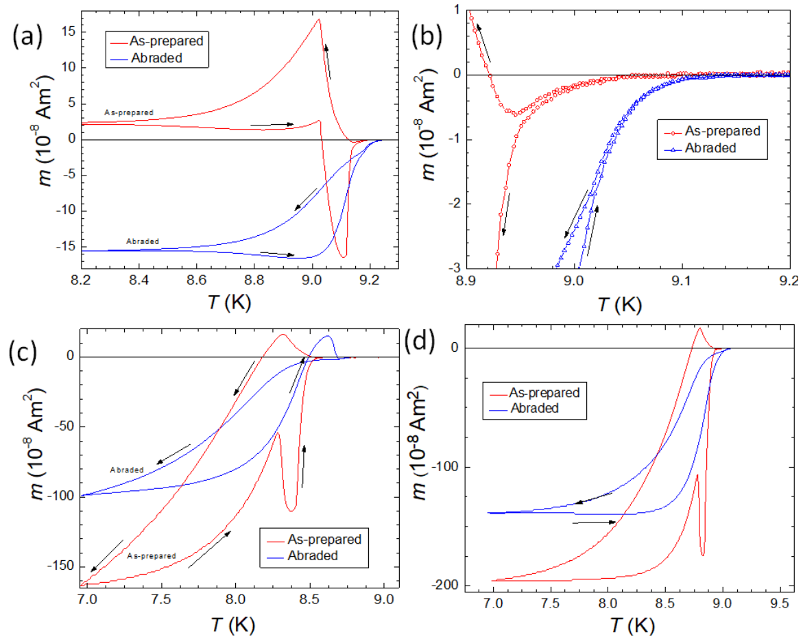
Figure 14. Abrading the surface of the Nb disks. Two samples punched from the same Nb sheet were studied, Nb1 left as is, and Nb2 was mechanically abraded on both top and bottom surface (the sample amount was reduced by 10 %). (a). FCC and FCW curves in an applied field of 2 mT. Sample Nb1 (as-prepared, —), and sample Nb2 (abraded, —). (b). Details around T_c of the data shown in (a). (c). FCC and FCW curves in an applied field of 20 mT. (d). FCC and FCW curves in an applied field of 60 mT. The abraded sample does not show any feature of the PME at any temperature/field as compared to the as-prepared sample Nb1.
