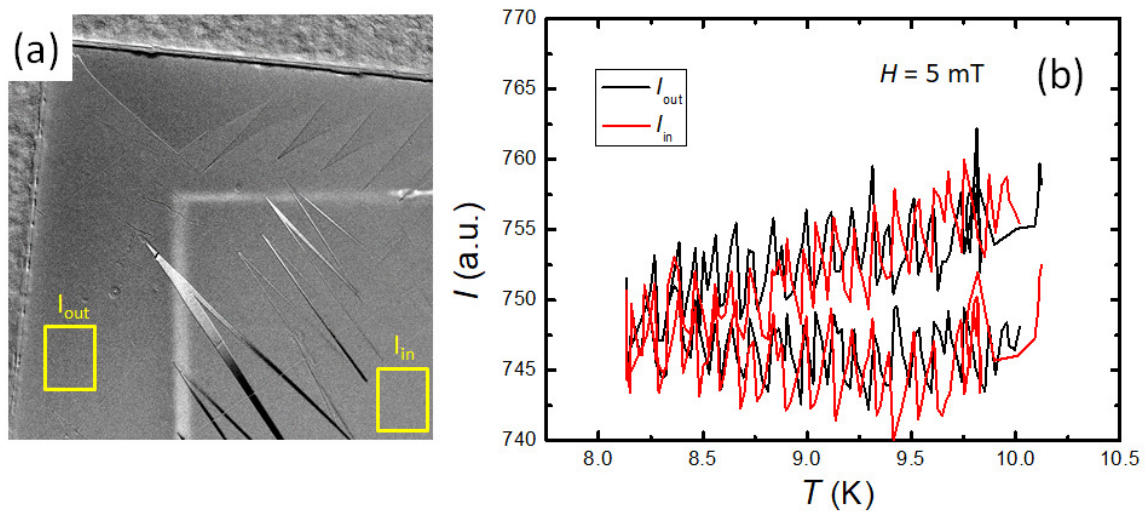
Figure 19. MO images obtained at University of Liège of an Nb disk from Detroit.
