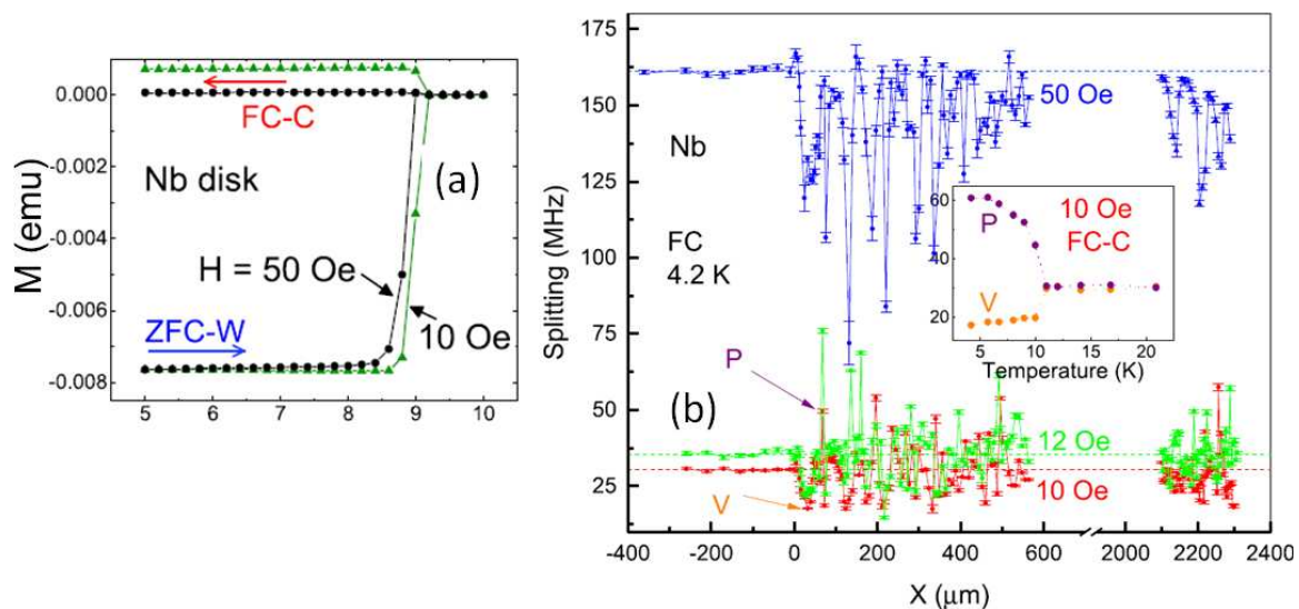
Figure 20. Diamond center imaging by AMES on an Nb sample with PME. (a). Temperature-dependent total magnetic moment measured using Quantum Design MPMS. Shown are ZFC-W and FC-C curves measured in Nb. (b). FC profiles of the magnetic induction for applied magnetic fields of 1.0, 1.2, and 5 mT (10, 12, and 50 Oe) recorded for an Nb disk-shaped crystal. Measurement performed at T = 4.2 K. The signatures of the paramagnetic Meissner effect (PME) are observed in various random regions for low magnetic fields. Cooling in 1 mT (10 Oe, red datapoints) and 1.2 mT (12 Oe, green datapoints) applied magnetic fields results in very similar profiles. The inset to (b) presents a temperature-resolved measurement in a 1 mT (10 Oe) magnetic field upon FC-C. The peak ('P') and valley positions ('V') of the inset are indicated by arrows in the main panel. Image reproduced with permission from Ref. [150].
