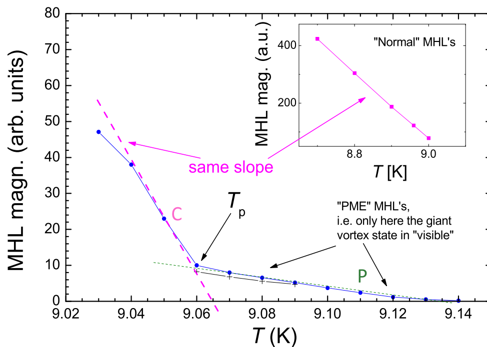
Figure 13. Evaluated details of the hysteresis measurements. The graph gives the MHL magnitude (maximum induced magnetic moment) as a function of temperature. The blue datapoints (●) give the data obtained from the MHLs, the black crosses (+) represent the data from a second run. The slope from the archtypal MHLs as shown in the inset (—) and the slope of the component C in the main panel (---) are the same. It is obvious from this graph that at T_p an abrupt change in the MHL shape takes place, and the normal flux pinning vanishes. At T > 9.06 K, the component P is measured following a completely different slope (---).
