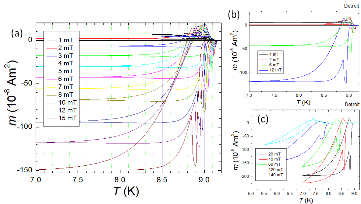
Figure 6. PME on a bulk Nb disk (from sheet D4S2, 127 \mu\text{m} thick, 3.2 mm radius). (a). FC-C and FC-W curves on the Nb disk in various applied magnetic fields ranging between 1 and 15 mT. (b). Figure shows the FC-C and FC-W curves only at 1, 2, 6 and 12 mT for clarity. (c). High-field (20, 40, 60, 120 and 140 mT) FC-C and FC-W curves on the same Nb sample. Note that a paramagnetic peak is reached in the FC-C curves at T_{pc} , and the FC-W curves show a peak ( T_{pw} ) and minimum ( T_{lw} ) in all applied magnetic fields. T_{pc} and T_{pw} correspond very well, whereas T_{lc} and T_{lw} show a distinct difference (see also Figure 9 below).
