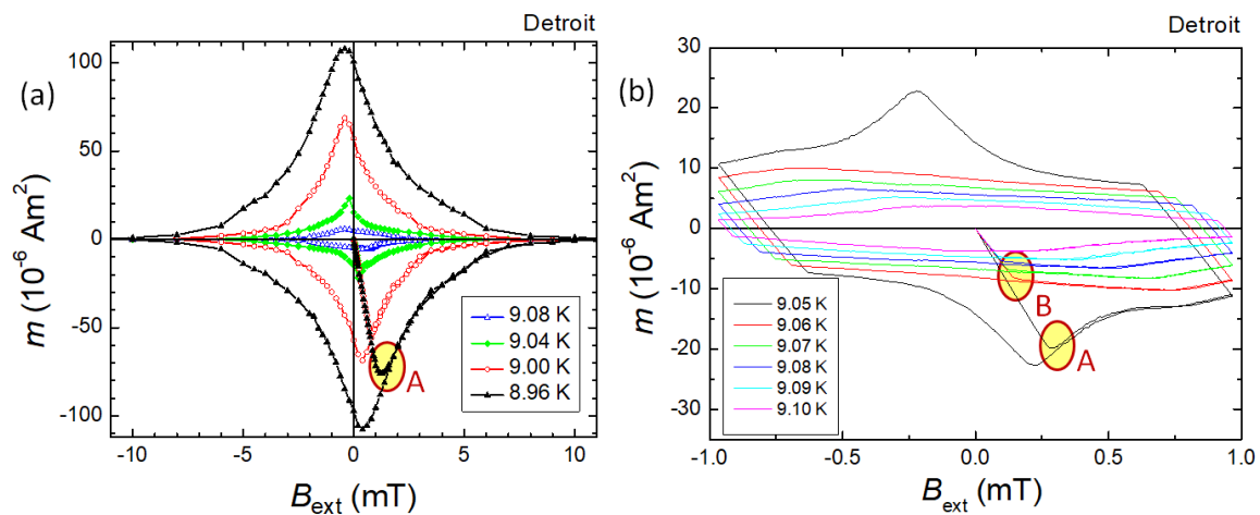
Figure 11. Magnetic measurements performed in Detroit on Nb disks with H \perp sample surface.
