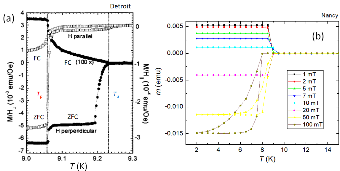
Figure 10. PME on Nb disks with perpendicular or parallel magnetic field. (a). M/H recorded in ZFC and FC modes with the magnetic field applied parallel ( \square ) and perpendicular ( \bullet ) to the Nb disk. The dashed vertical lines indicate the temperatures T_u \leq T_1 and T_p , see text. Reprinted with permission from Ref. [116]. (b). PME on a Nb disk with the applied magnetic field parallel to the sample surface, measured in the year 2023 in Nancy using a QD PPMS-VSM system [134]. The lines serve as guides for the eye.
