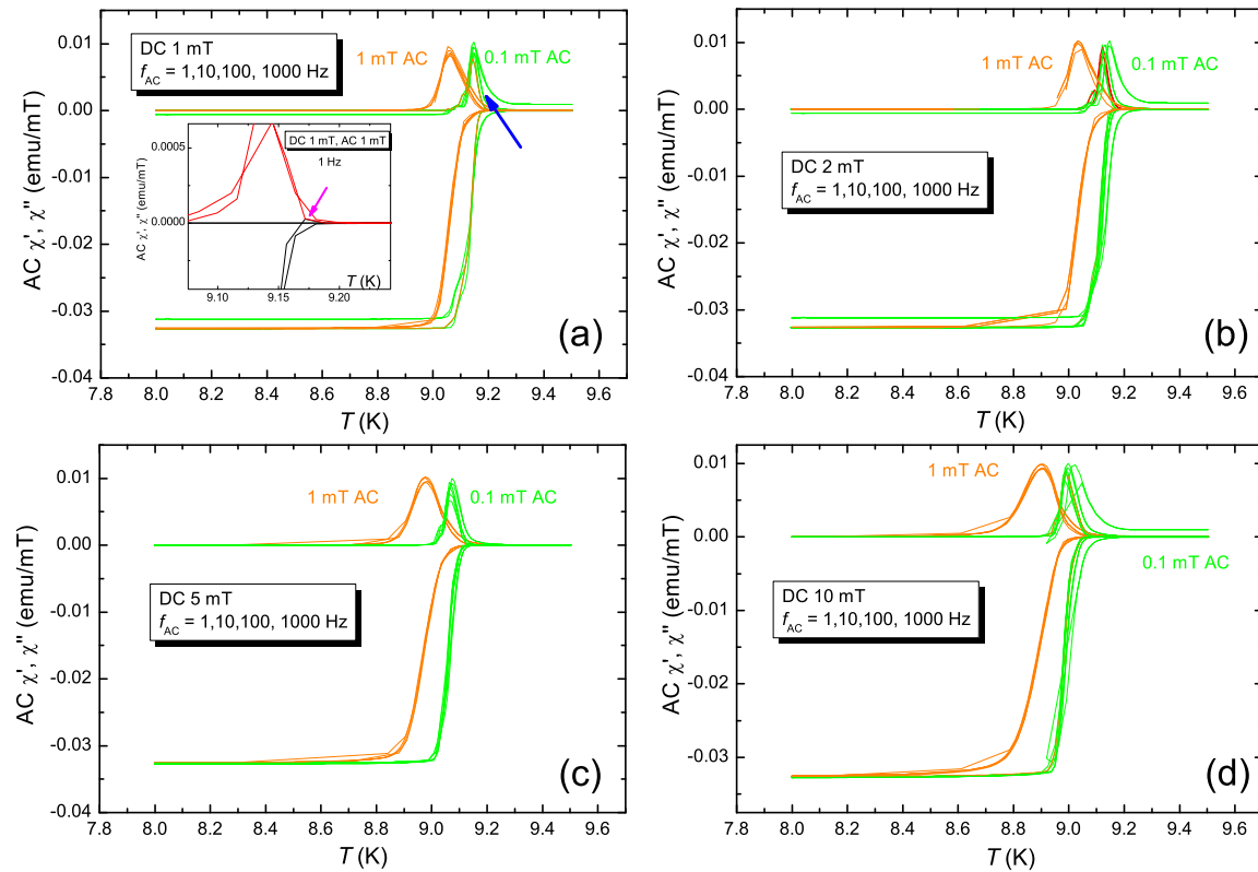
Figure 17. AC measurements on an Nb disk performed at IJL Nancy. The AC frequencies were varied between 1, 10, 100 and 1000 Hz, and two AC amplitudes of 0.1 mT (—) and 1 mT (—) were applied. (a). Measurement with an applied DC field of 1 mT. The blue arrow points to a secondary loss peak when warming up. The inset presents the superconducting transition for 1 Hz, DC field 1 mT, AC amplitude 1 mT. The imaginary part, \chi'' , is given by —, and the real part \chi' by —. The magenta arrow indicates a tiny positive signal in \chi' . (b). Measurement with an applied DC field of 2 mT. (c). Measurement with an applied DC field of 5 mT. (d). Measurement with an applied DC field of 10 mT.
