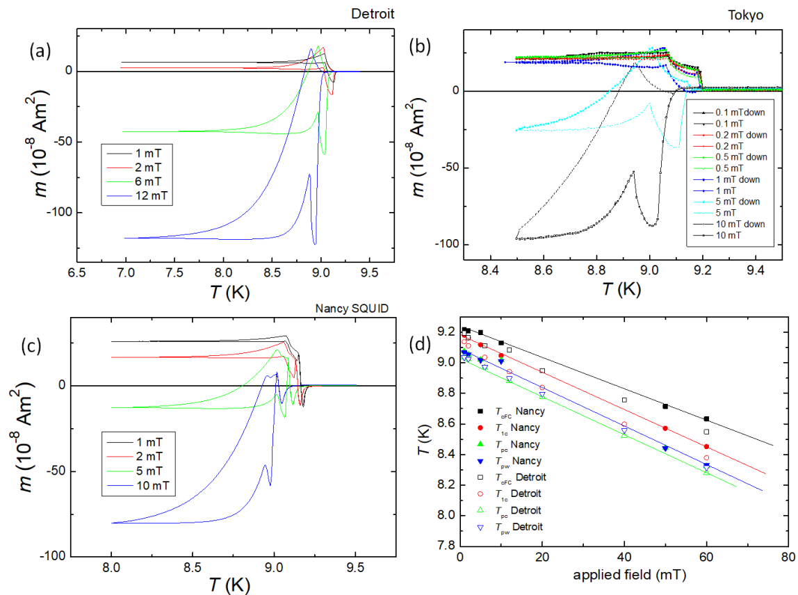
Figure 16. FC-C and FC-W measurements of m(T) performed using the same sample (Nb002) in 3 places on Earth with more than 20 years difference between the experiments. (a). Original measurement in Detroit, 1997. SQUID with stationary sample. (b). Measurement performed at SRL/ISTEC, Tokyo, 1999, using a 5T-SQUID with ultra-low field option. (c). Measurement performed at IJL Nancy, 2019, using an MPMS3 SQUID system with small scan length. (d). Comparison of the Detroit and Nancy data concerning the characteristic temperatures T_1 , T_p , and T_{cFC} (i.e., T_c obtained from FC data).
