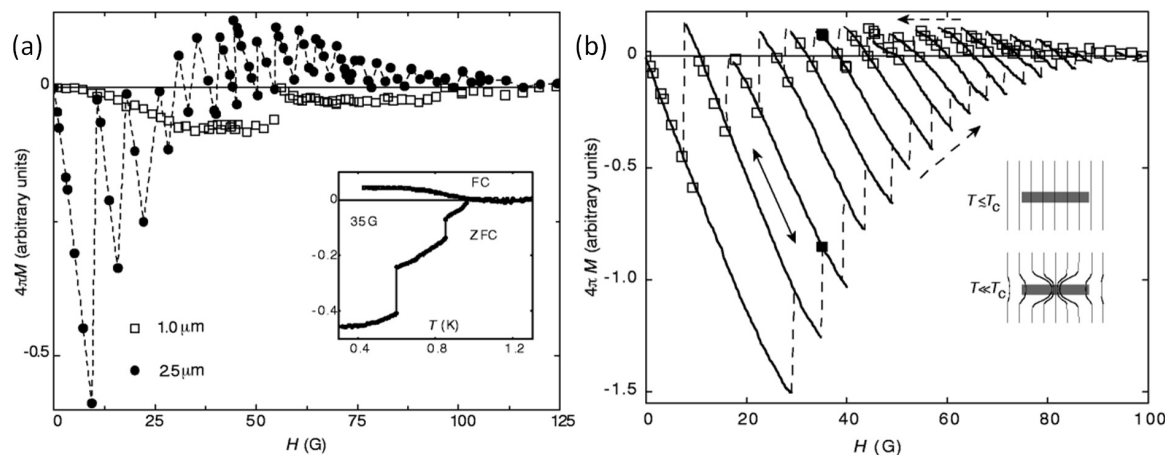
Figure 22. Magnetic susceptibility, \chi , of mesoscopic Al disks, see also Figure 2f. (a). Field dependence of the Meissner response for a Al disk with 1.0 \mu\text{m} diameter ( \square ) and for one with 2.5 \mu\text{m} diameter ( \bullet ). The thickness is for both disks 0.1 \mu\text{m} . The strongly oscillating behaviour clearly seen (the dashed line is a guide to the eye) for the larger sample is due to size quantization. Each jump corresponds to a change in the number of vortices inside the disk, which can either form an array of single quantum vortices or assemble into a single giant vortex. The inset to (a) compares the field-cooling (FC) and zero-field-cooling (ZFC) magnetization for the 2.5-mm disk at the field where the paramagnetic response is close to its maximum value. The ZFC response is always diamagnetic, and the jumps in the ZFC curve correspond to entry of individual vortices into the disk interior. (b). Comparison of the magnetization states reached by cooling in a field and by sweeping the field at a constant temperature (arrows) at T = 0.4 K. The field-cooling (FC-C) data shown by \square are for the 2.5- \mu\text{m} disk shown in (a). The filled boxes ( \blacksquare ) indicate the low-temperature states as shown in the inset to (a), ZFC and FC. The inset to (b) illustrates the compression of a giant vortex ( T close but below T_c ) into a smaller volume ( T further away from T_c ), which enables extra flux to enter the sample at the surface. Image reproduced with permission from Ref. [63].
