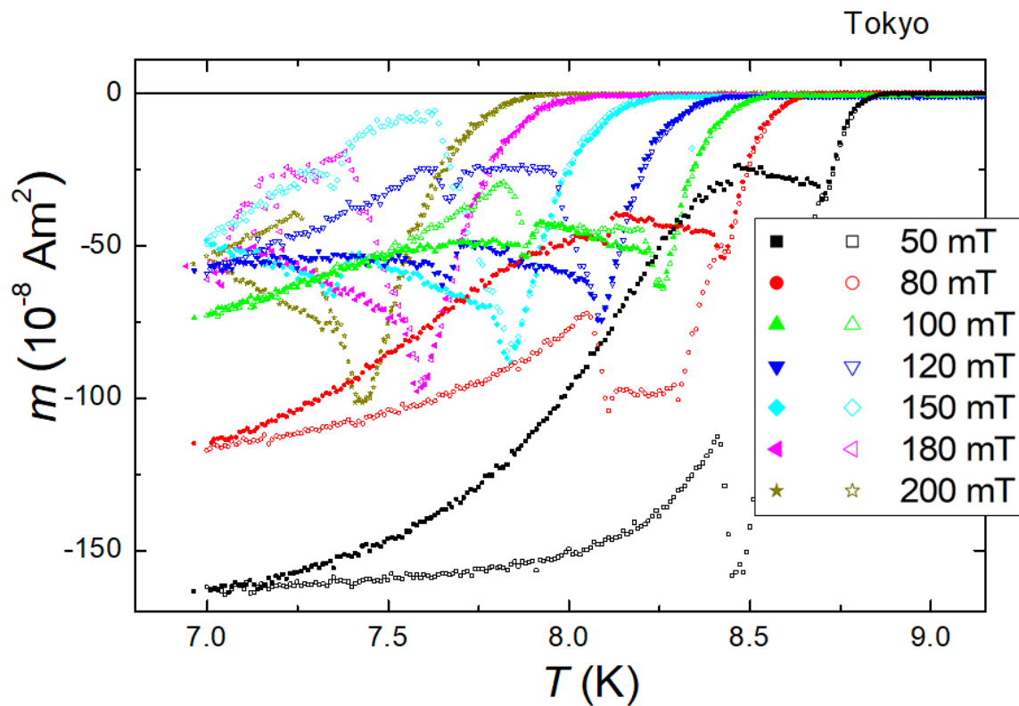
Figure 7. High-field measurements of the superconducting transition performed in Tokyo (sample Nb002) using a 7T-XL-SQUID [134]. The data were measured in FC-C (field-cooled cooling, filled symbols) and FC-W (field-cooled warming, open symbols) with a constant temperature sweep rate ( |dT/dt| = 0.01 K/min). m(T) is always negative, but we must note here the characteristic steps on the FC-W curves indicating the PME.
