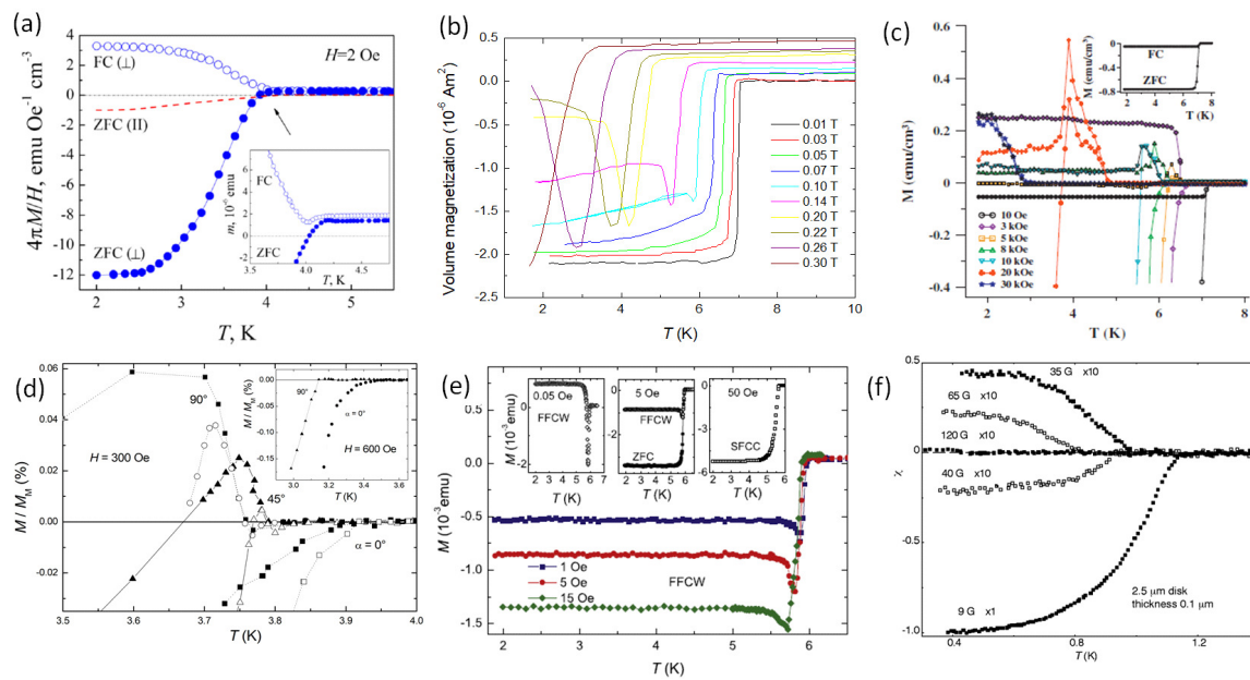
Figure 2. PME observed on various metallic superconducting samples I. (a) Rings of In-Sn, measured in FC and ZFC modes (applied field H = 0.2 mT (2 Oe) with the field applied parallel and perpendicular to the sample surface (ZFC ( \perp ) ●, ZFC ( \parallel ) - - - - -, FC ( \perp ) ○). The inset shows details of the superconducting transition. Reprinted with permission from Ref. [49]. (b) Pb-films on PEEK, rolled up into cylinders. Data shown are FC curves in various applied fields (0.01 T – 0.3 T). Graph redrawn from the data presented in Ref. [50]. (c) Pb porous. FC and ZFC data are shown for various applied fields. The inset gives the standard measurement at low applied field. Reprinted with permission from Ref. [33]. (d) Ta foil. Shown are the superconducting transitions at H = 30 mT (300 Oe) and for 3 different angles ( 0^\circ , 45^\circ and 90^\circ of the field to the sample surface). Reprinted with permission from Ref. [35]. (e) ZrB 12 crystals, measured at 0.1 mT (1 Oe), 0.5 mT (5 Oe), and 1.5 mT (15 Oe) applied field. The insets give details of the transition at 5 \mu T (0.05 Oe) (FFC-W), 0.5 mT (5 Oe) (FFC-W and ZFC) and 5 mT (50 Oe) (SFC-C), where the F stands for ‘fast’ and S for ‘slow’. Reprinted with permission from Ref. [37]. (f) Susceptibility of an Al mesoscopic disk (2.5 \mu m dia., thickness 0.1 \mu m) at applied fields of 0.9, 3.5, 4.0, 6.5 and 12 mT (9, 35, 40, 65 and 120 G). The last 4 curves were multiplied by a factor of 10. The authors point out that there is no hysteresis when cooling/warming. Reprinted with permission from Ref. [63].
