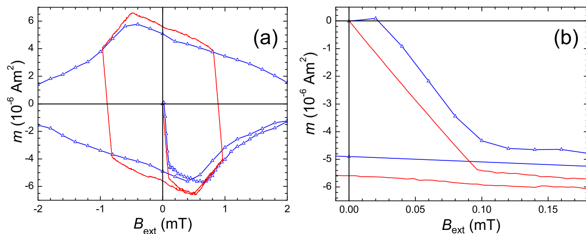
Figure 4. Comparison of m(H) data achieved using the stationary sample technique versus the moving sample in standard SQUID. The data were measured at Detroit at a temperature T = 9.08 K. (—) Conventional QD SQUID measurement with moving sample and field generated by the superconducting magnet. (—) The magnetic moment is evaluated directly from the SQUID voltage, whereas the field was generated by a copper coil. More details on such magnetization loops will be discussed in Section 3.3 below. (a) Comparison of hysteresis loops measured by the two methods, sample Nb1. (b) Comparison of the virgin curves and their merging to the main hysteresis loops, sample Nb1.
