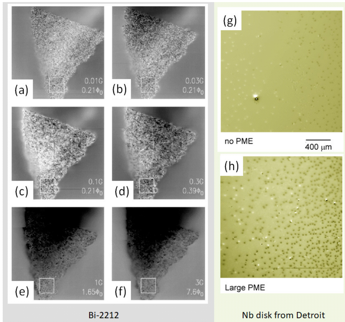
Figure 18. Scanning SQUID microscope images. (a–f) present images of a granular Bi-2212 sample, cooled and imaged in various applied magnetic fields. Each image comprises 512 \times 512 pixels, and each pixel represents a distance of 6 \mu\text{m} . The individual images are labelled by the cooling field, and by the maximal range of variation of the flux (in units of the flux quantum, \Phi_0 ) in each case. The small rectangles indicate where profiles were taken in Ref. [104], which are not shown here. All images were taken at T = 4.2 \text{ K} . (a). Cooling field 1 \mu\text{T} (0.01 G), 0.21 \Phi_0 . (b). Cooling field 3 \mu\text{T} (0.03 G), 0.21 \Phi_0 . (c). Cooling field 10 \mu\text{T} (0.1 G), 0.21 \Phi_0 . (d). Cooling field 30 \mu\text{T} (0.3 G), 0.39 \Phi_0 . (e). Cooling field 100 \mu\text{T} (1 G), 1.65 \Phi_0 . (f). Cooling field 300 \mu\text{T} (3 G), 7.6 \Phi_0 . (g)–(h) give images obtained on a Nb disk from Detroit at T = 4.2 \text{ K} . (g). Sample with no PME, applied field of \sim 1.6 \mu\text{T} (1.6 mG). (h) sample with strong PME, applied field \sim 2.8 \mu\text{T} (2.8 mG). Images (a)–(f) reproduced with permission from Ref. [104], images (g) and (h): Courtesy of J.R. Kirtley.
