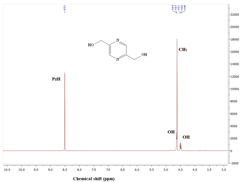
Figure S3. 1 H NMR spectra of pyrazine-2,5-diyl dimethanol (pzydmH2)
