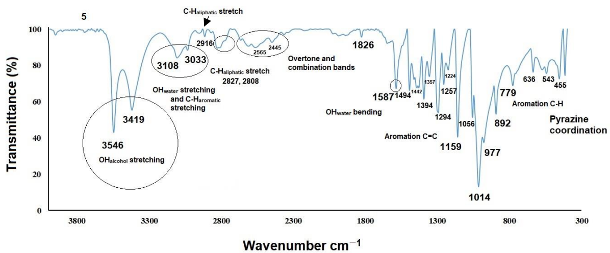
Figure S13. IR spectrum of 5.
