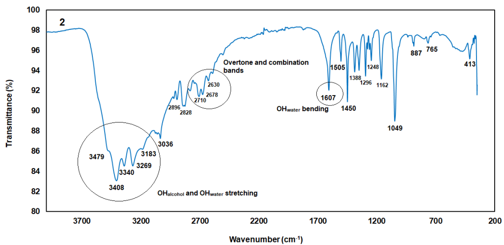
Figure S11. IR spectrum of 2.
