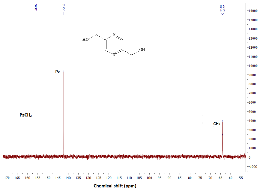
Figure S4. 13 C NMR spectra of pyrazine-2,5-diyl dimethanol (pzydmH2)
