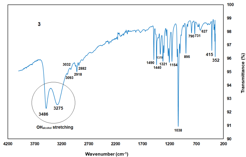
Figure S12. IR spectrum of 3.
