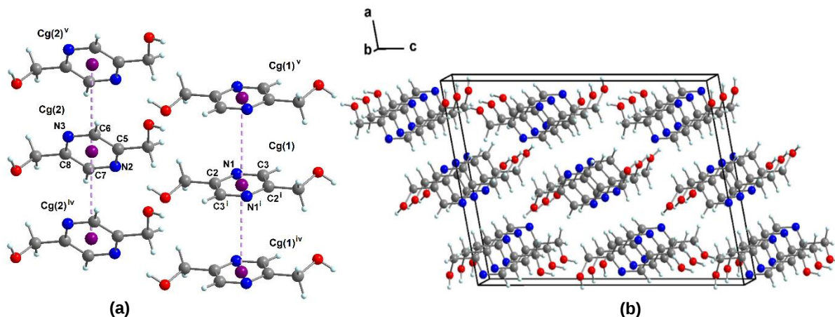
Figure S5. (a) \pi - \pi interactions between the pyrazine rings are depicted by the dashed bonds in light purple color. (b) A view of the cell packing diagram of pzydmH2 .
