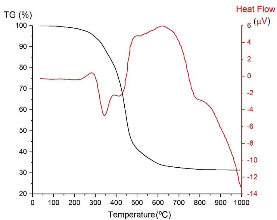
ESI Figure 2 TG-DSC of the of the Zr-loaded thiourea-functionalized styrene-divinylbenzene copolymer under N 2 atmosphere.
