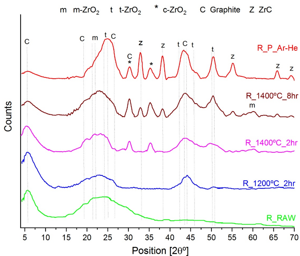
ESI Figure 5 XRD pattern of the samples produced by calcination of the Zr-loaded thiourea-functionalized styrene-divinylbenzene copolymer
