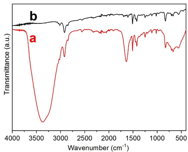
ESI Figure 1 FT-IR spectra of the unloaded and Zr-loaded thiourea-functionalized styrene-divinylbenzene copolymer
