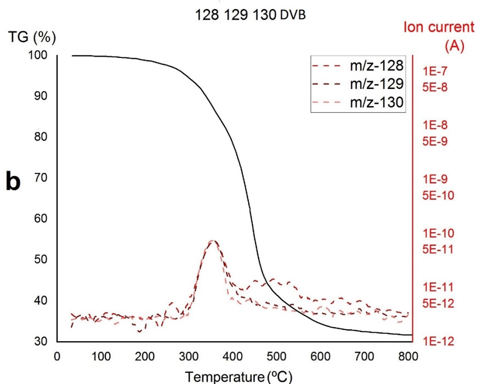
ESI Figure 3 TG-MS of the Zr-loaded thiourea-functionalized styrene-divinylbenzene copolymer: Ph-CHCH^+ ( m/z=103 ), PhCH^+ ( m/z=91 ), C_6H_x^+ ( x=3,4,5 , m/z=63,64,65 ) (a) , and DVB fragments ( m/z=130,129,128 ) (b)
