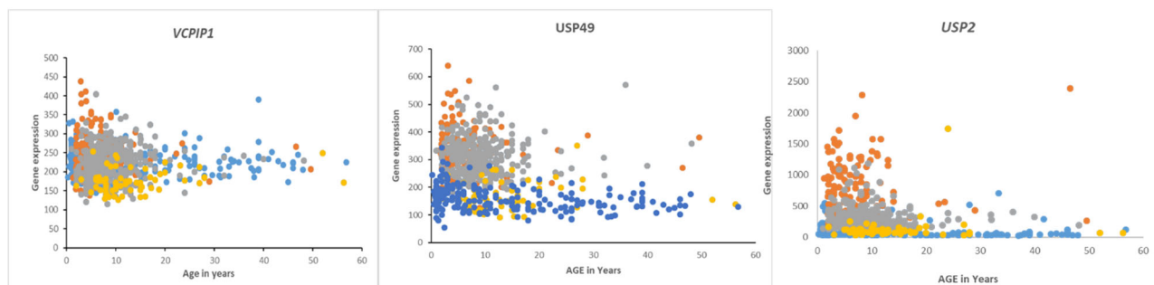
Figure 10. Gene expression of VCPIP1 , USP49 and USP2 in medulloblastoma by age and subgroups. Orange – Group 3, Gray – Group 4, Blue – SHH, Yellow – Wnt. Of these genes USP2 expression was most specifically elevated in Group 3 MB infants and children compared to the other groups (Cavalli dataset) and compared to a non-tumor group (Swartling dataset).
