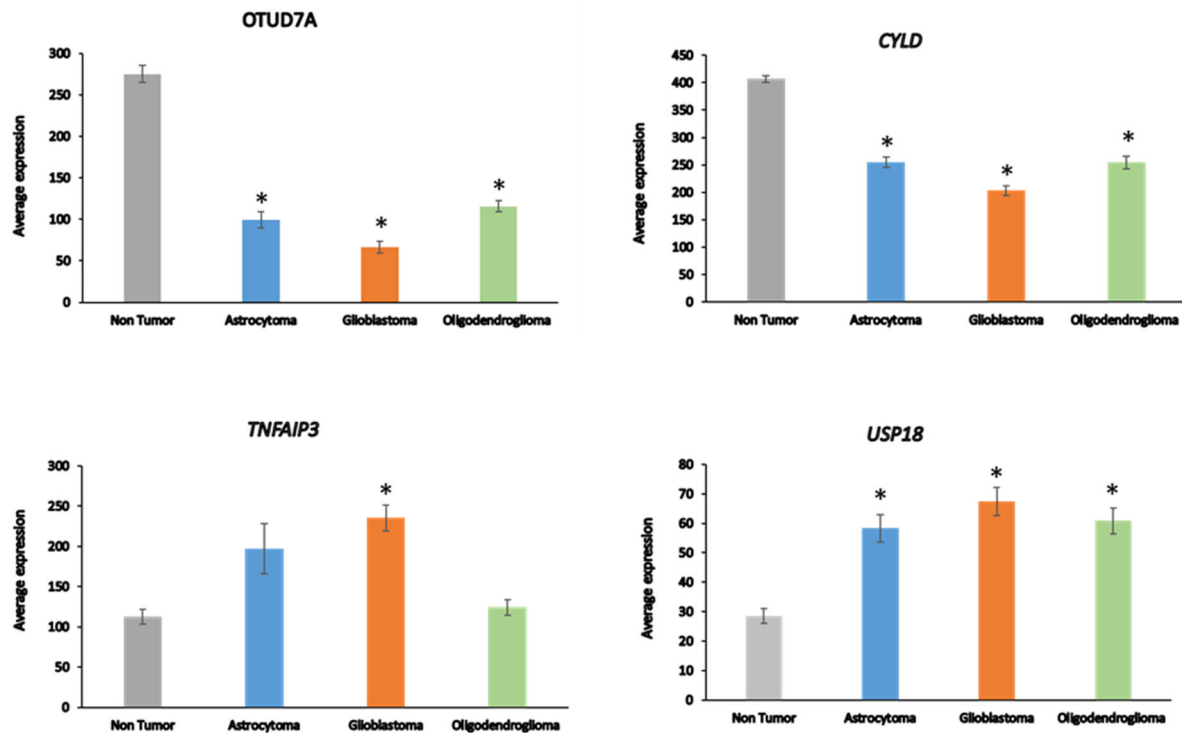
Figure 4. Differentially expressed DUBs identified under the GO category of Regulation of immune response in different glioma and non-tumor brain. * p < 0.001 compared to non-tumor group.
