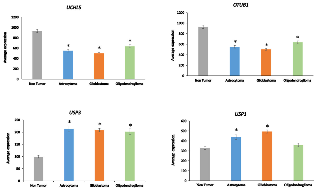
Figure 5. Differentially expressed DUB genes in the GO category of DNA repair. UCHL5 , F = 21.83 , p = 4.97\text{e-}120 ; OTUB1 , F = 42.71 , p = 1.12\text{E-}20 ; USP3 , F = 19.33 , p = 7.56\text{e-}11 ; USP1 , F = 16.99 , p = 1.04\text{e-}09 . * p < 0.001 compared to Non tumor group by t-test.
