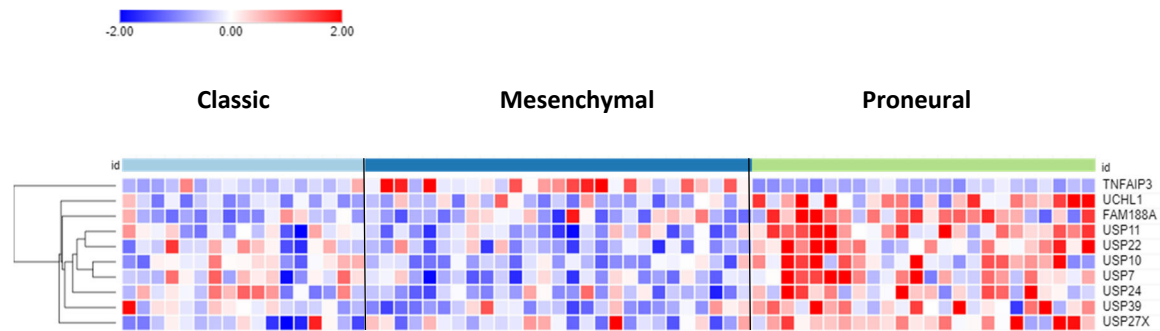
Figure 3. Heatmap and cluster analysis of DUB genes differentially expressed in GBM subtypes. On average, TNFAIP3 expression was higher in the GBM mesenchymal group, whereas the expression of the other 9 genes was greater in the proneural group. Classic, N = 17; Mesenchymal, N = 27; Proneural, N = 24).
