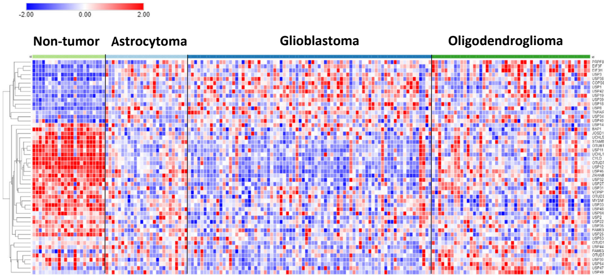
Figure 1. Heatmap and cluster analysis of differentially expressed DUBs in gliomas. Non-tumor, N = 23; Astrocytoma, N = 26; Glioblastoma, N = 77; Oligodendroglioma, N = 50).
