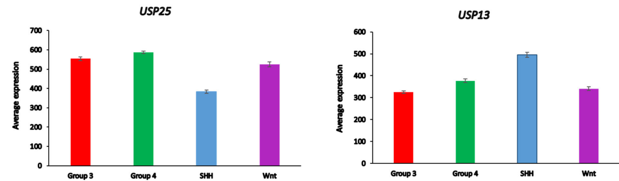
Figure 11. Differential expression of ERAD-associated DUBs in different medulloblastoma subgroups (Cavalli dataset). USP25 , F = 138.98, p = 9.08\text{e-}72 ; USP 13 , F = 49.90, p = 1.93\text{e-}29 .
