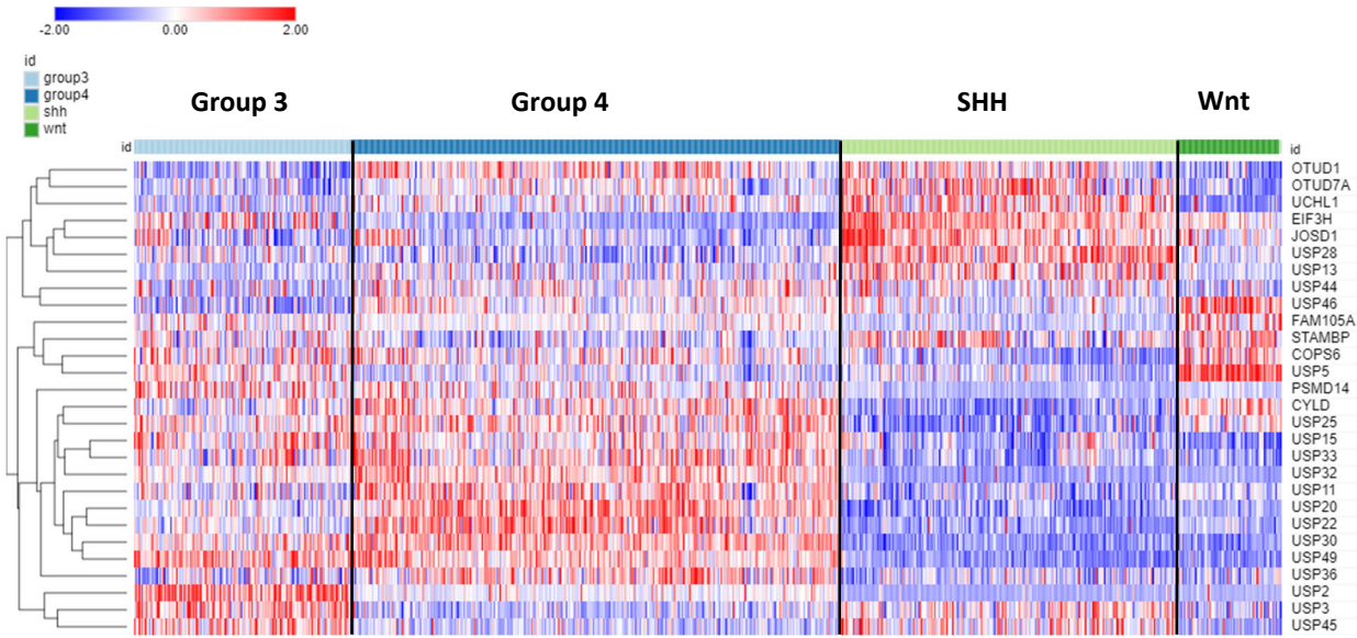
Figure 9. Heatmap and cluster analysis of the top 12 differentially expressed DUB genes for each of the four MB subgroups compared to non-tumor brain (Note that due to overlap the total is less than 48). The Swartling dataset was used to identify top genes differing from non-tumor controls. The Cavalli dataset was used for the construction of the heatmap depicting the expression of these genes. Based on gene expression in the MB subgroups, the most significantly elevated DUBs for each group were: Group 3 – USP2 ; Group 4 – USP20 ; SHH – EIF3H ; WNT – USP5 . Group 3, N = 144; Group 4, N = 326; SHH, N = 223; Wnt, N = 70).
