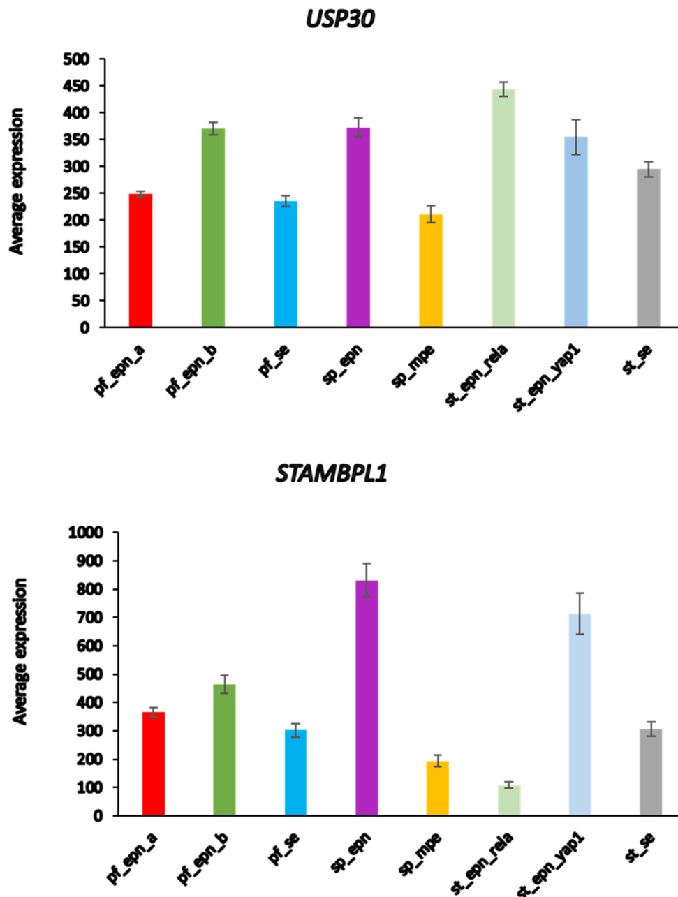
Figure 7. Differential expression of USP30 and STAMBPL1 in ependymoma molecular subgroups. USP30 , F = 12.58 , p = 2.38 \times 10^{-13} ; STAMBPL1 , F = 54.29 , p = 5.23 \times 10^{-43} . This dataset is missing non-tumor control group for comparison by t test.
