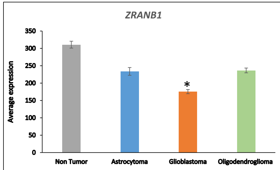
Figure 2. Differential expression of USP46 and ZNRANB1 in adult glioma groups. USP46 ( F = 42.34 , p = 1.53e-20 ); ZNRANB1 ( F = 45.17 , p = 1.40e-21 ) in the Sun dataset; Non tumor N = 23 , Astrocytoma, N = 26 , Glioblastoma, N = 77 , Oligodendroglioma, N = 50 ).
