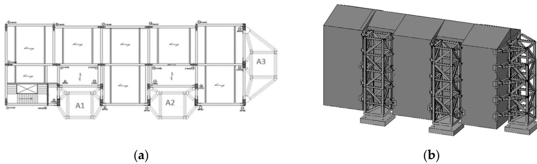
Figure 7. Planar and 3D view of the retrofitted building (A 1 , A 2 , and A 3 are the designed ADS).
