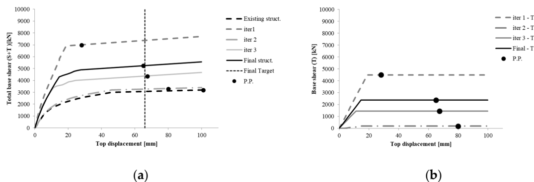
Figure 8. Variation of global response S+ADS (cumulative base shear-top displacement) and contribution of the dissipative towers T (towers base shear-top displacement).
