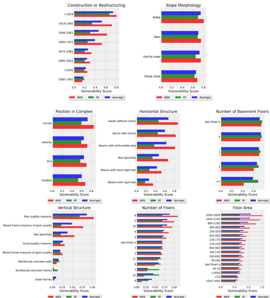
Figure 7. A-posteriori Vulnerability scores for the 8 considered building features, calculated by both random forest (RF, green bars) and artificial neural network (ANN, red bars) models, highlighting the impact of specific attributes on overall building vulnerability. For each feature, the average score of the two models is also reported (blue bars), representing a more reliable measure of the true features' vulnerability.
