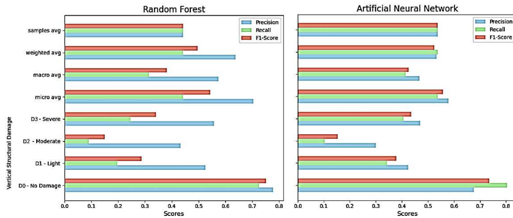
Figure 5. Performances on validation data: we evaluate the standard metrics of precision, recall and their geometric average, usually named F1 score; precision evaluates the percentage of true positives in classification, while recall is the percentage of buildings of any given class that were identified as such. We evaluate performance on each class and report various weighted averages.
