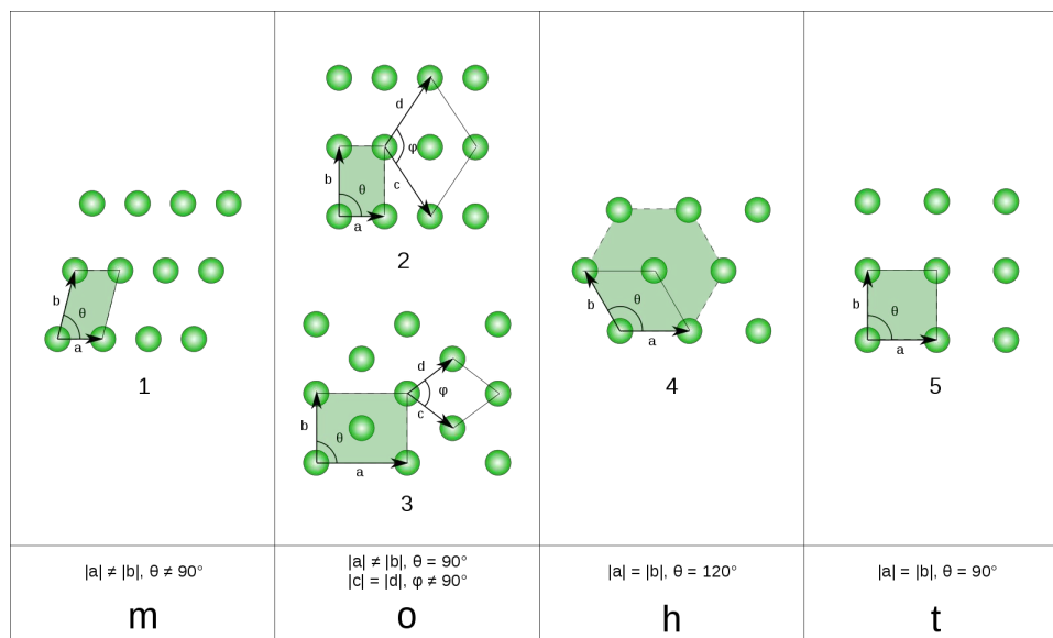
Figure 7. Five 2D lattice types. From 2d Bravais Licence CC BY-SA 3.0 DEED .
