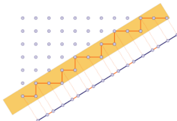
Figure 11. Cut and Project trick is a method to get a quasiperiodic set in \mathbb{R} from a lattice in \mathbb{R}^2 (From Cut&Project Fibonacci CC BY-NC-SA 2.0 Deed ).
