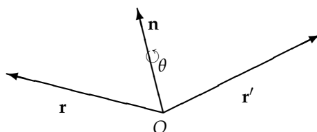
Figure 9. Proper rotation of vector \mathbf{r} to \mathbf{r}' by angle \theta about unit vector \mathbf{n} in space \mathbb{R}^3 .
