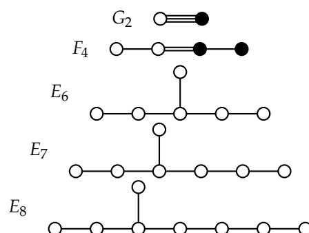
Figure A2. From top to bottom: Dynkin diagrams for G_2 , F_4 , E_6 , E_7 , E_8
