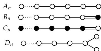
Figure A1. Dynkin diagrams A_n , B_n , C_n , D_n
