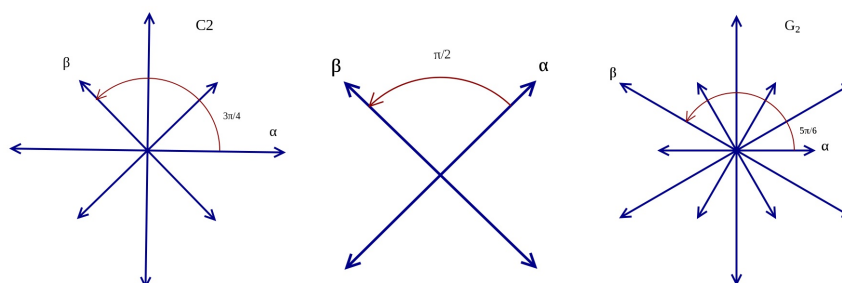
Figure A4. rank-2 root systems C_2 , D_2 , G_2 (from Licence CC BY-SA 3.0 DEED ).
