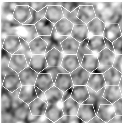
Figure 12. Quasicrystalline five-fold surface of \text{Al}_{70}\text{Pd}_{21}\text{Mn}_9 , from [45].
