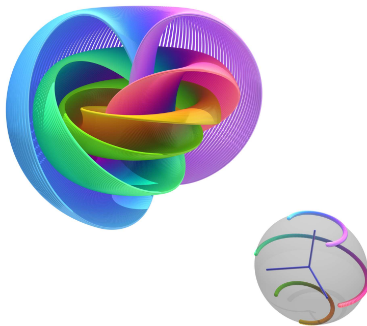
Figure 16. Hopf fibration (from Niles Johnson CC BY 4.0). The described fiber bundle structure, succinctly represented as \mathbb{S}^1 \hookrightarrow \mathbb{S}^3 \xrightarrow{p} \mathbb{S}^2 , intricately intertwines the components of the fiber space \mathbb{S}^1 within the overarching structure of the total space \mathbb{S}^3 . The projection, denoted as p and referred to as Hopf's map, serves as the intermediary, mapping the elements of \mathbb{S}^3 onto the base space \mathbb{S}^2 . In this visual representation, each fiber of \mathbb{S}^1 projects to a circle in three-dimensional space, with one such circle extending to infinity, forming what is termed a "circle through infinity" or effectively a line. The resulting arrangement fills space with a captivating array of tori (products of two circles), each of which is the stereographic projection of the inverse image of a latitude circle on \mathbb{S}^2 . The accompanying image on the right, depicting linked keyrings on the right, serves as an illustrative example of one of these tori. Points on \mathbb{S}^2 and their corresponding fibers are color-matched, providing a visual insight into the intricate and captivating structure induced by the Hopf fibration.
