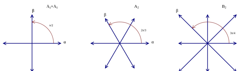
Figure A3. rank-2 root systems A_1 \times A_1 , A_2 , B_2 (from Licence CC BY-SA 3.0 DEED ).
