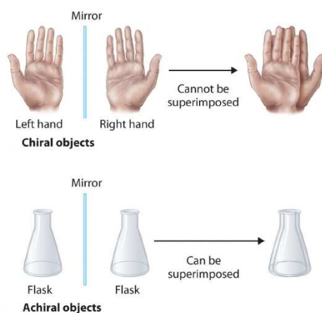
Figure 2. From https://chem.libretexts.org Licence CC BY-SA 4.0 DEED
