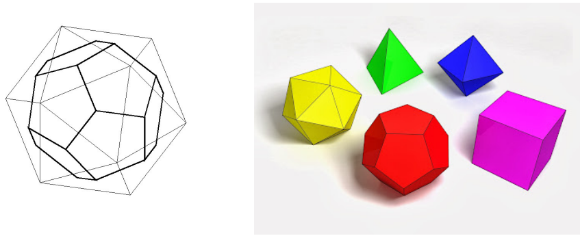
Figure 10. Dodecahedron and its dual, the icosahedron (left). With its twenty triangular faces, twelve vertices and thirty edges, the latter is one of the five Platonic Solids (right). From Don Steward: platonic solids and duals . Among the platonic solids (Theaetetus of Athens, 417- 369 BC; Plato, 428/427–348/347 BC; Euclid, fl. c. 300 BC; Johannes Kepler, 1571-1630), either the dodecahedron or the icosahedron may be seen as the best approximation to the sphere. Remind that a platonic solid is a convex polyhedron with vertices in a sphere \mathbb{S}_r^2 of radius r . The faces of a platonic solid are congruent regular polygons, with the same number of faces meeting at each vertex. All edges are congruent, as are its vertices and angles. See the celebrated Coxeter treatise [42] to know more about these objects.
