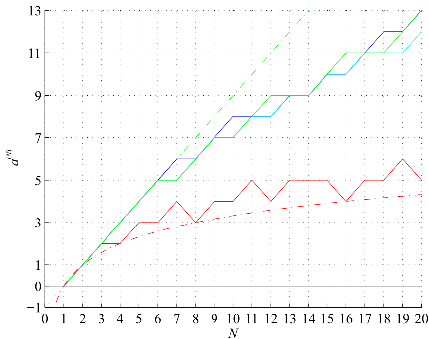
Figure 2. Lower bound on the binary string assembly index ?? (red) and \log_2(N) (red, dash-dot), conjectured upper bound on the binary string assembly index ?? (green), factual values of the string assembly index (blue) and the distinct string assembly index (cyan) and N - 1 (green, dash-dot), for the string length 0 \leq N \leq 20 .
