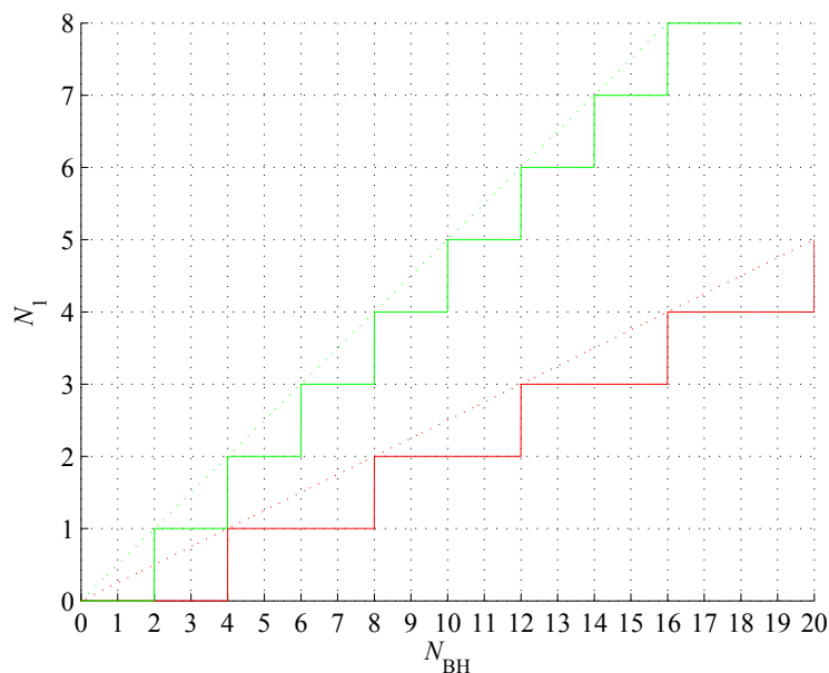
Figure 6. Lower (red) and upper (green) bound on the number of APTs N_1 on a VS as a function of the information capacity of the generating BB [?].
