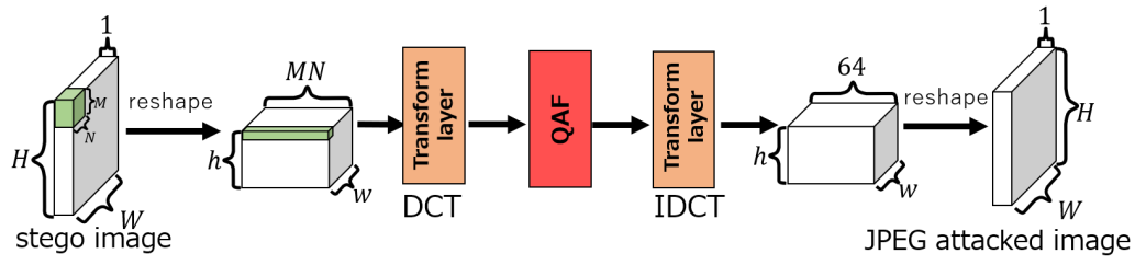
Figure 8. Proposed attack layer
