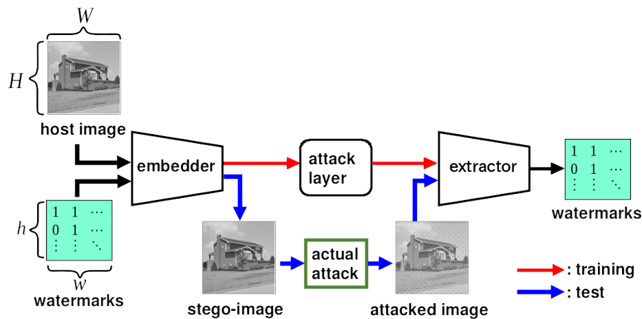
Figure 2. Overall structure of ReDMark [11]
