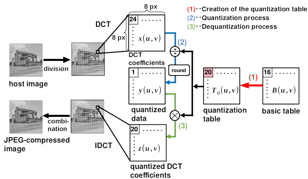
Figure 1. JPEG compression quantization for luminance components. 1) Creation of the quantization table T_Q , 2) The quantization process, 3) The dequantization process.
