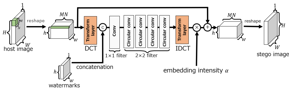
Figure 3. Embedding network of ReDMark [11]
