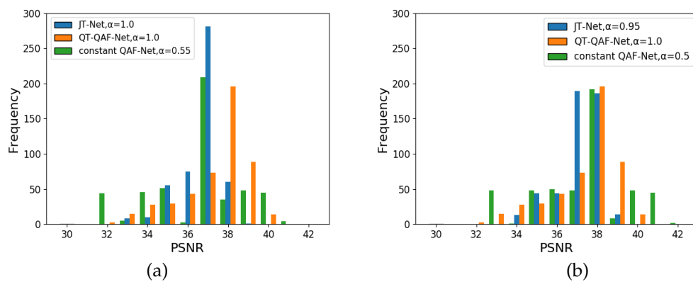
Figure 14. Histogram of PSNR for embedding intensity \alpha = 1.0 for QT-QAF-Net: (a) intensity \alpha = 1.0 for JT-Net and \alpha = 0.55 for constant QAF-Net and (b) intensity \alpha = 0.95 for JT-Net and intensity for constant QAF-Net \alpha = 0.50 .
