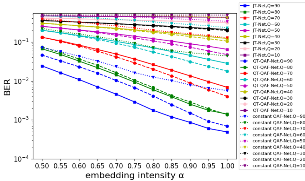
Figure 13. BER for embedding intensity \alpha
