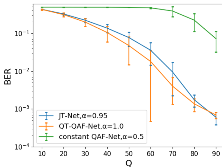
Figure 15. BER for the JPEG compression level Q
