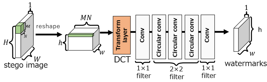
Figure 5. Extraction network of ReDMark [11]
