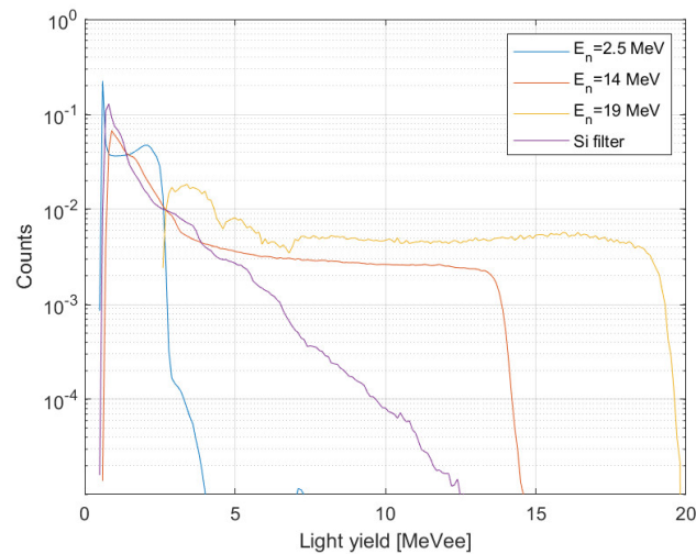
Figure 9. The normalized pulse-height spectra for p-Therphenyl scintillator.
