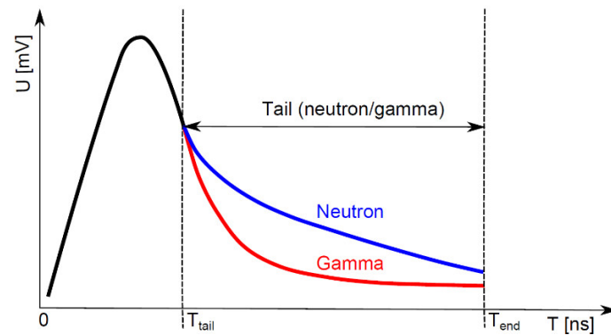
Figure 5. The Mechanism of pulse shape discrimination.
