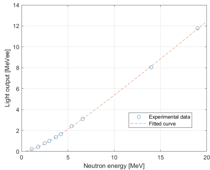
Figure 8. The light output function for p-Terphenyl scintillator.
